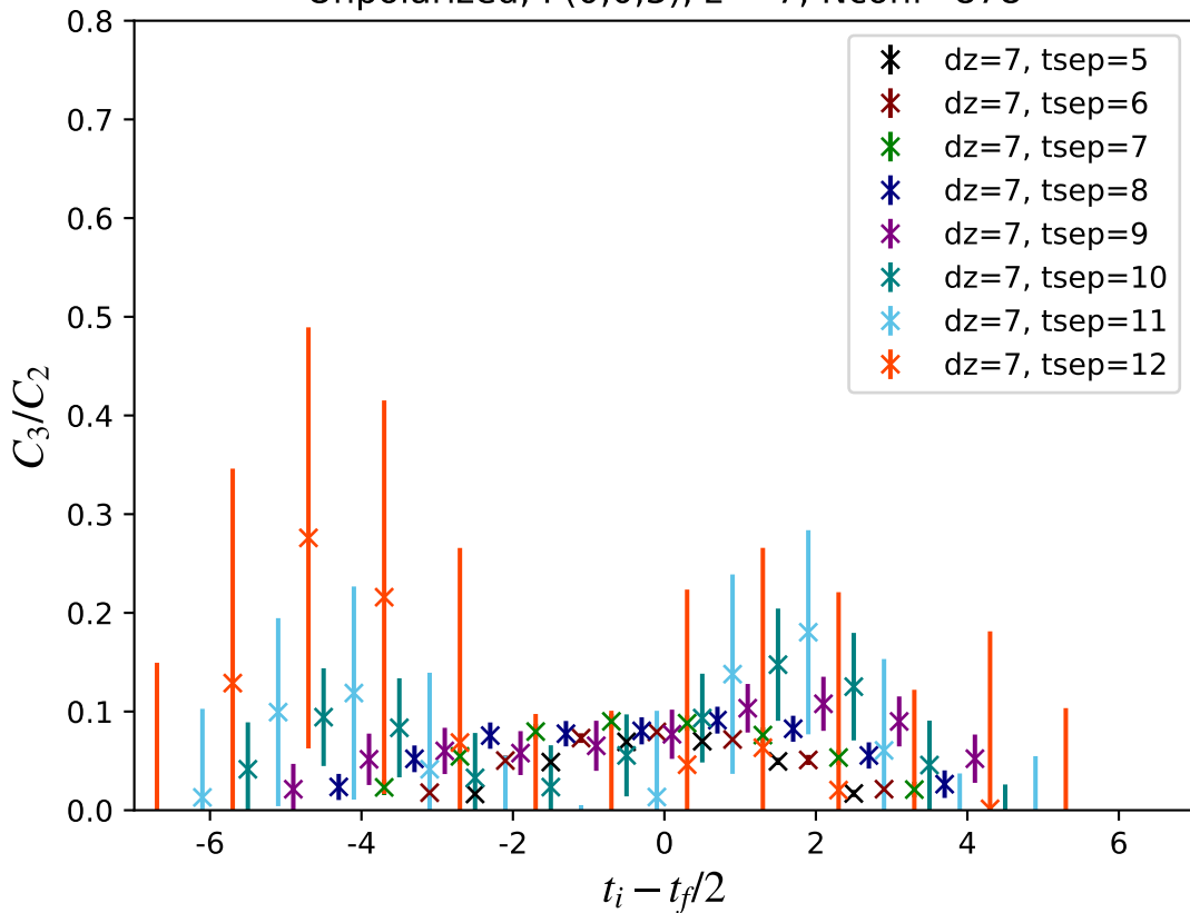
Unpolarized, P(0,0,3), z = 7 , Nconf=878
