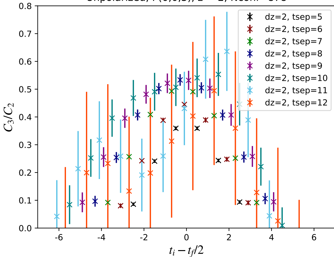
Unpolarized, P(0,0,3), z = 2 , Nconf=878
