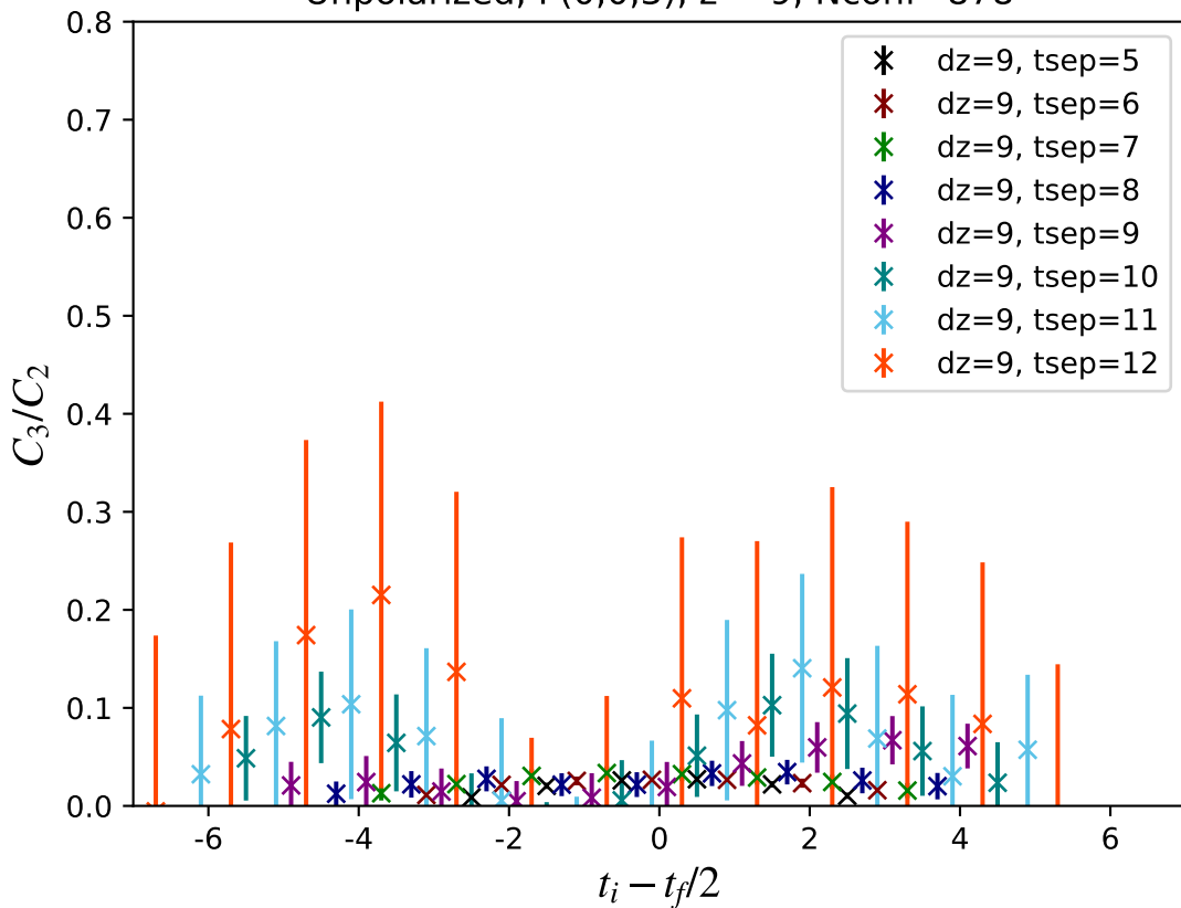
Unpolarized, P(0,0,3), z = 9 , Nconf=878
