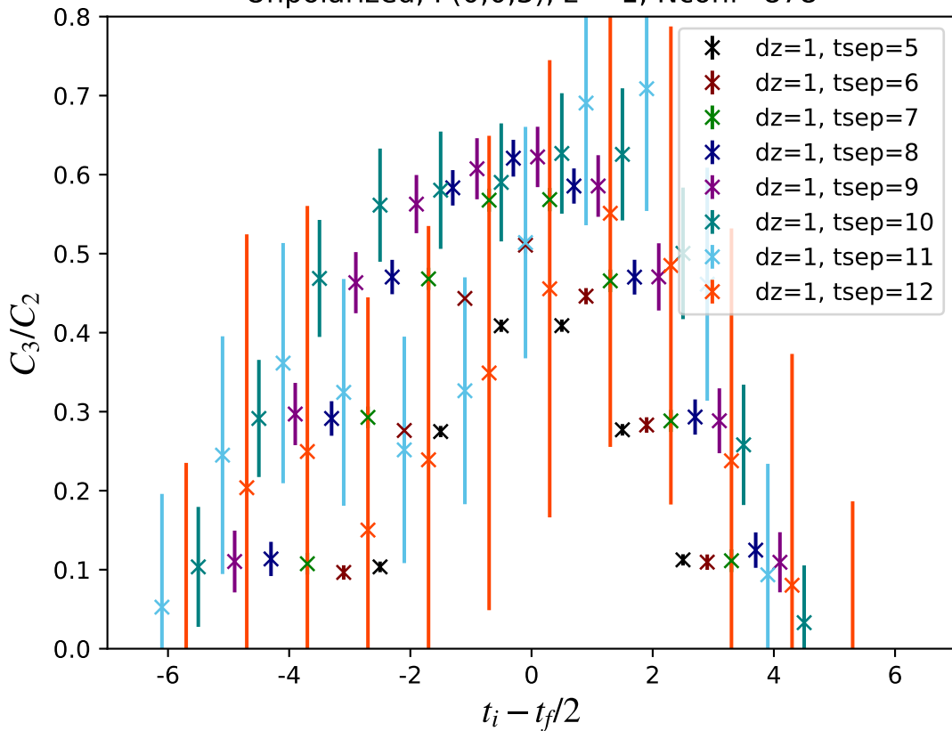
Unpolarized, P(0,0,3), z = 1 , Nconf=878
