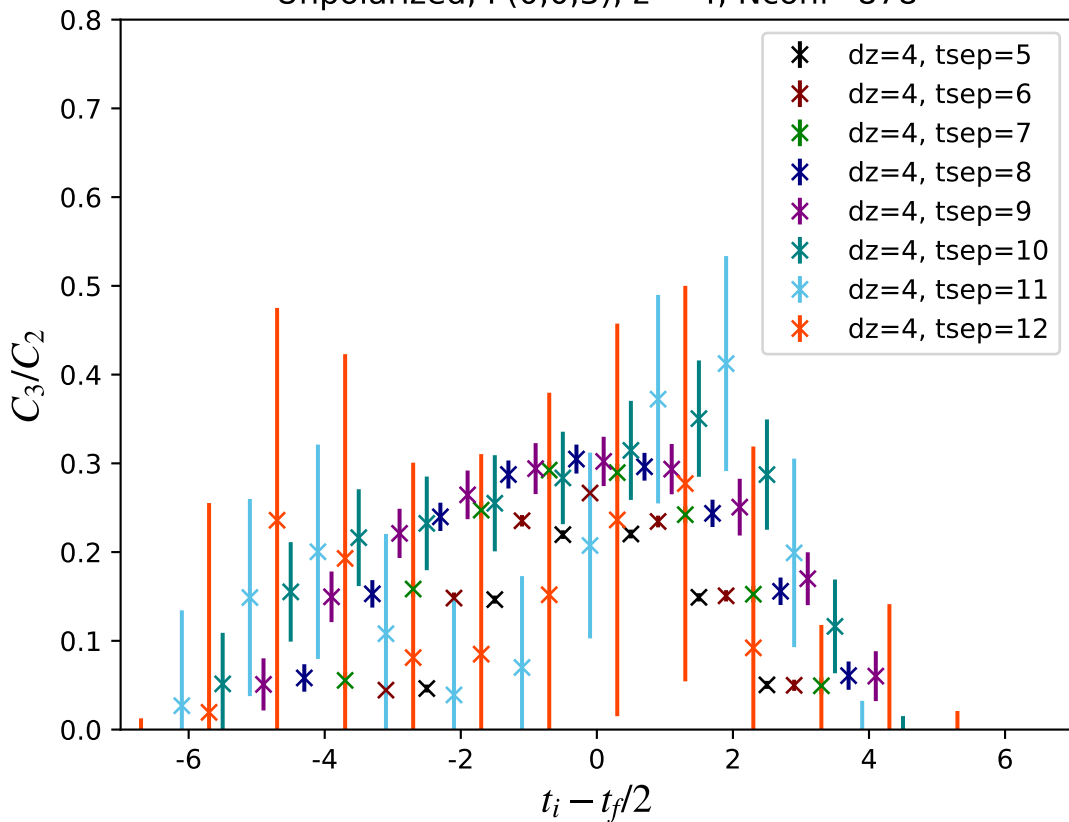
Unpolarized, P(0,0,3), z = 4 , Nconf=878
