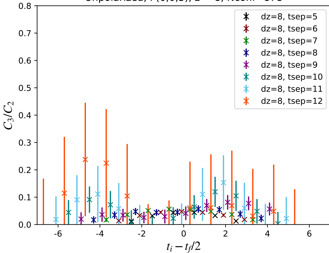
Unpolarized, P(0,0,3), z = 8 , Nconf=878
