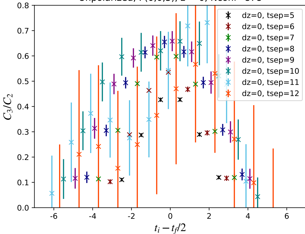
Unpolarized, P(0,0,3), z = 0 , Nconf=878
