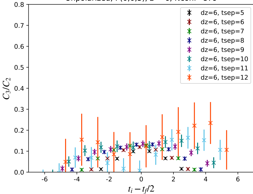
Unpolarized, P(0,0,3), z = 6 , Nconf=879
