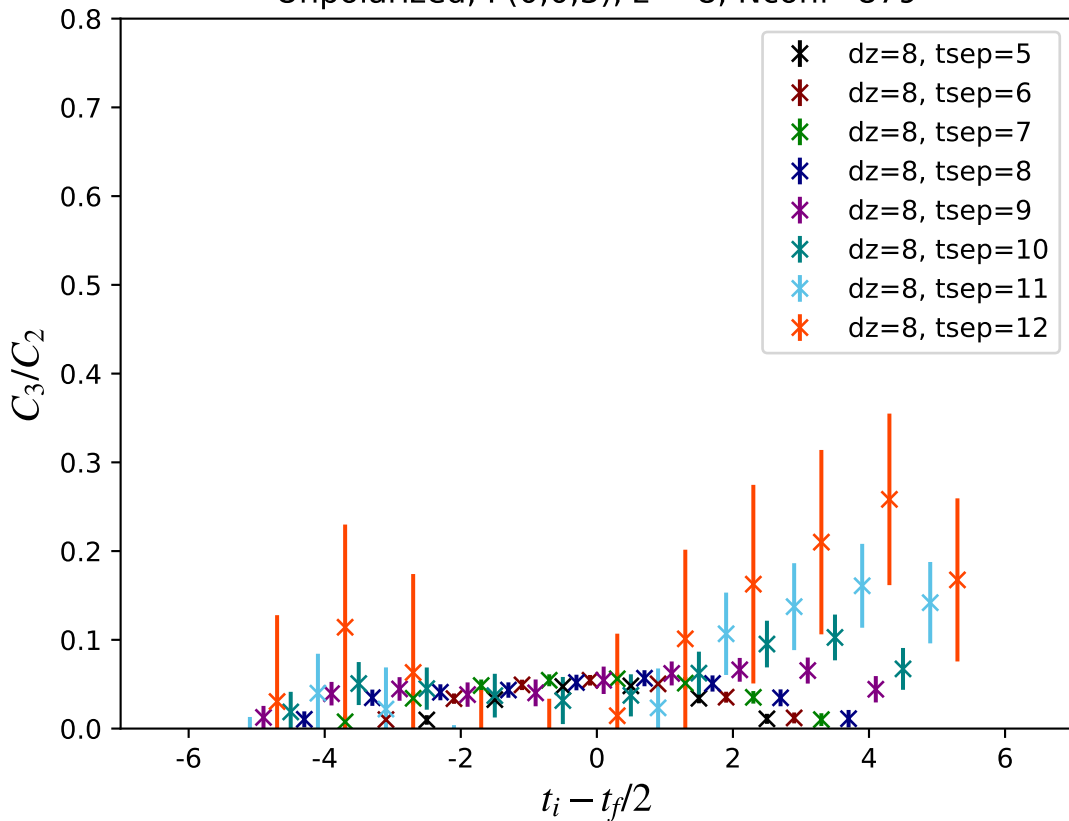
Unpolarized, P(0,0,3), z = 8 , Nconf=879
