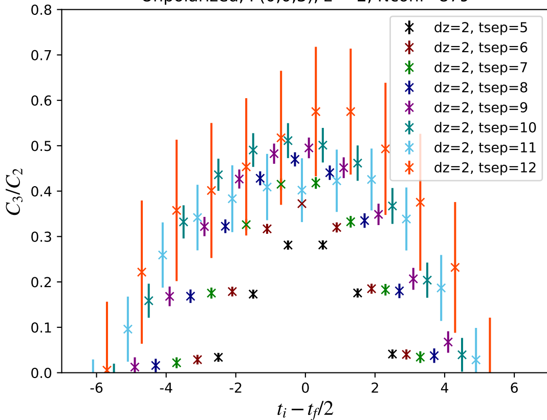
Unpolarized, P(0,0,3), z = 2 , Nconf=879
