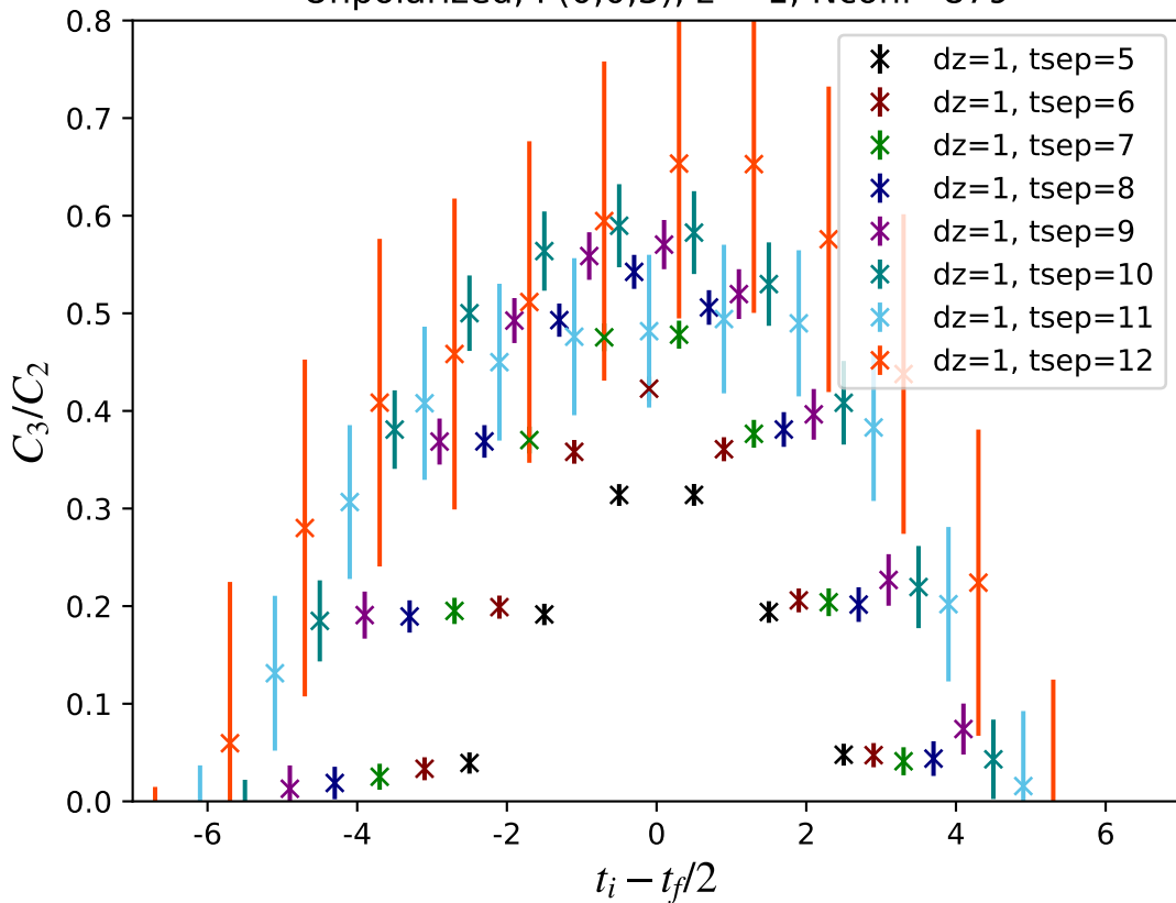
Unpolarized, P(0,0,3), z = 1 , Nconf=879
