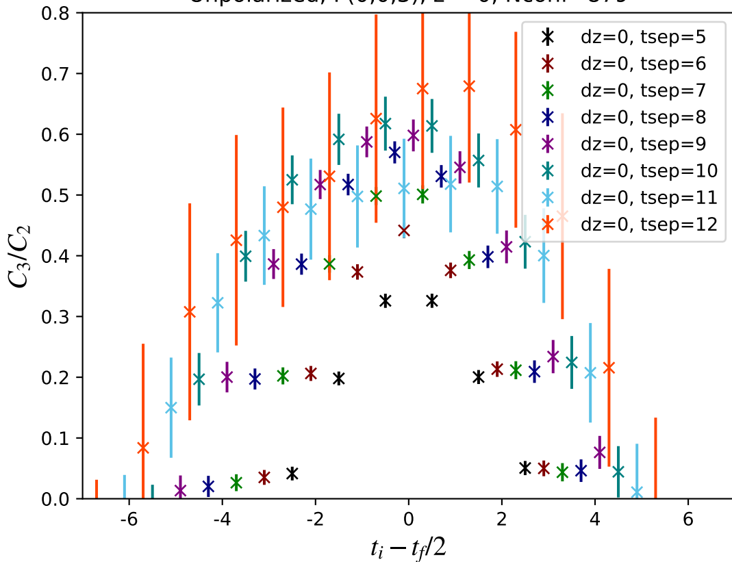
Unpolarized, P(0,0,3), z = 0 , Nconf=879
