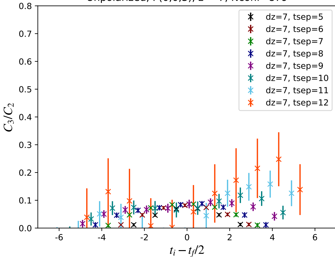
Unpolarized, P(0,0,3), z = 7 , Nconf=879
