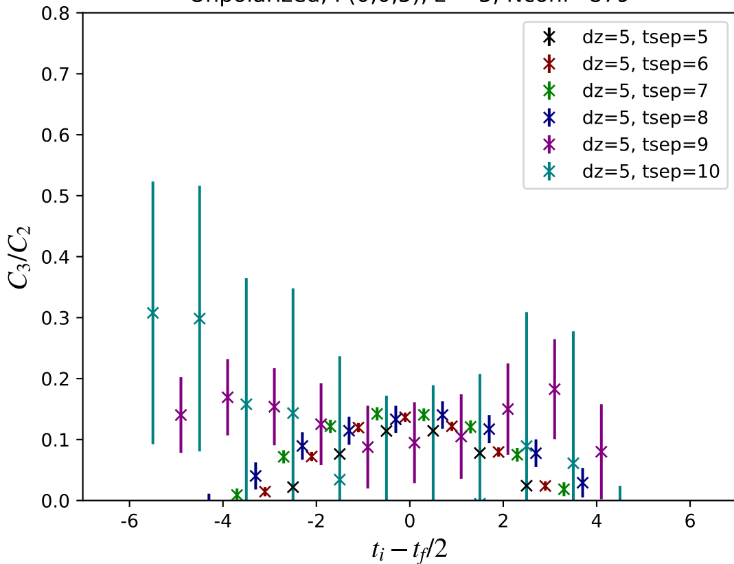
Unpolarized, P(0,0,5), z = 5 , Nconf=879
