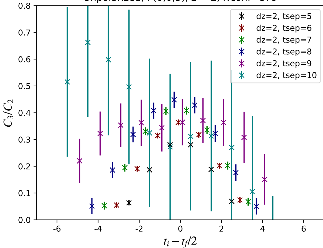
Unpolarized, P(0,0,5), z = 2 , Nconf=879
