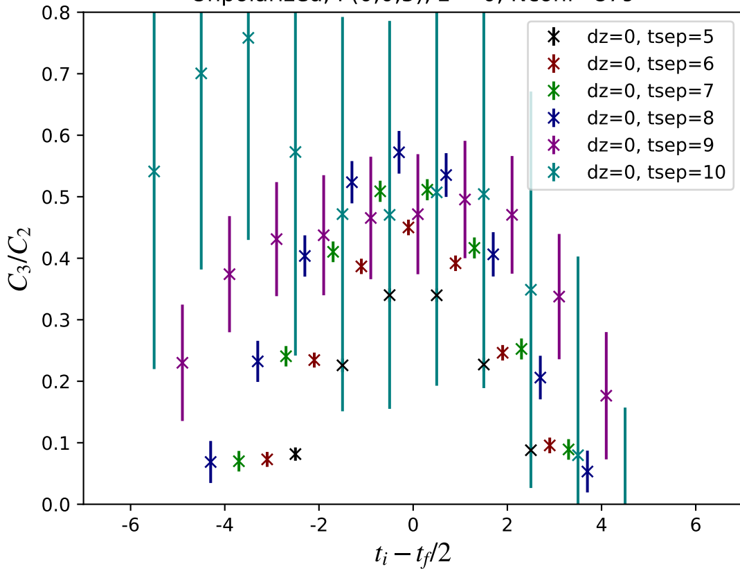
Unpolarized, P(0,0,5), z = 0 , Nconf=879
