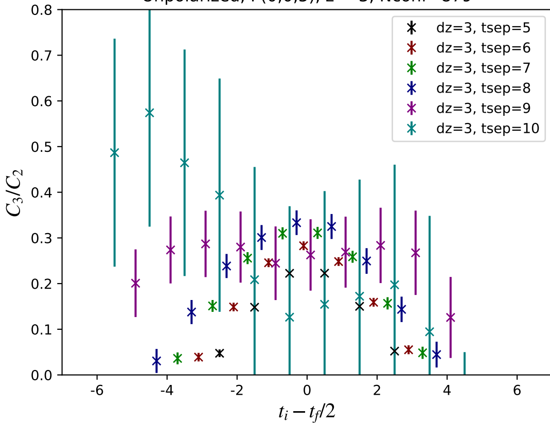
Unpolarized, P(0,0,5), z = 3 , Nconf=879
