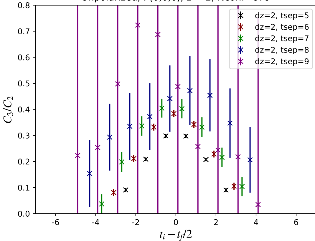
Unpolarized, P(0,0,6), z = 2 , Nconf=879
