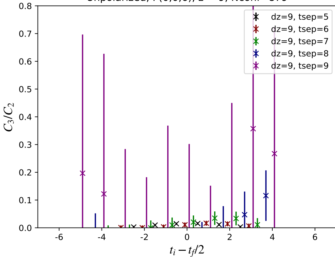
Unpolarized, P(0,0,6), z = 9 , Nconf=879
