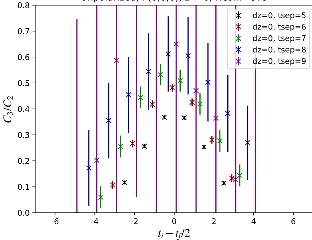
Unpolarized, P(0,0,6), z = 0 , Nconf=879
