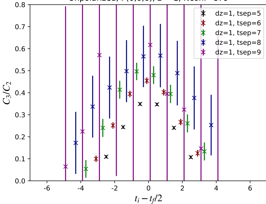
Unpolarized, P(0,0,6), z = 1 , Nconf=879
