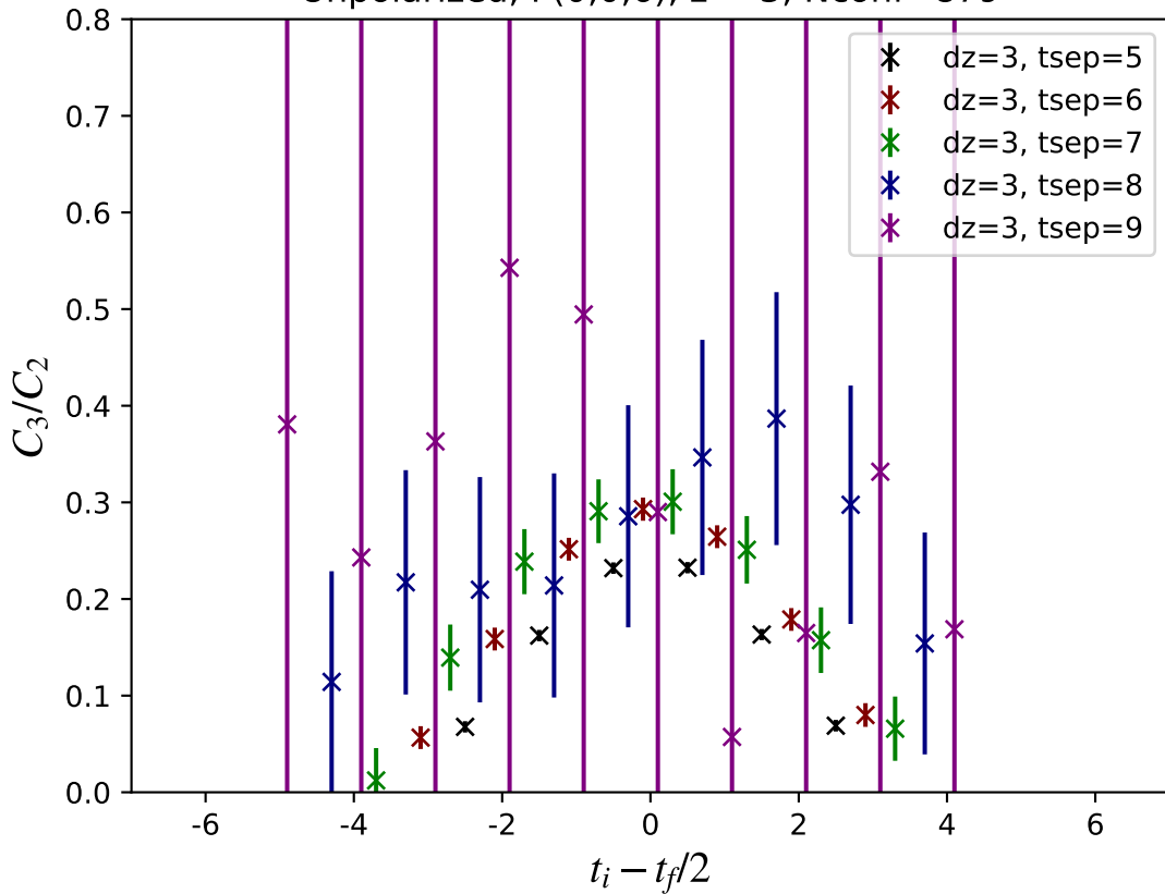
Unpolarized, P(0,0,6), z = 3 , Nconf=879
