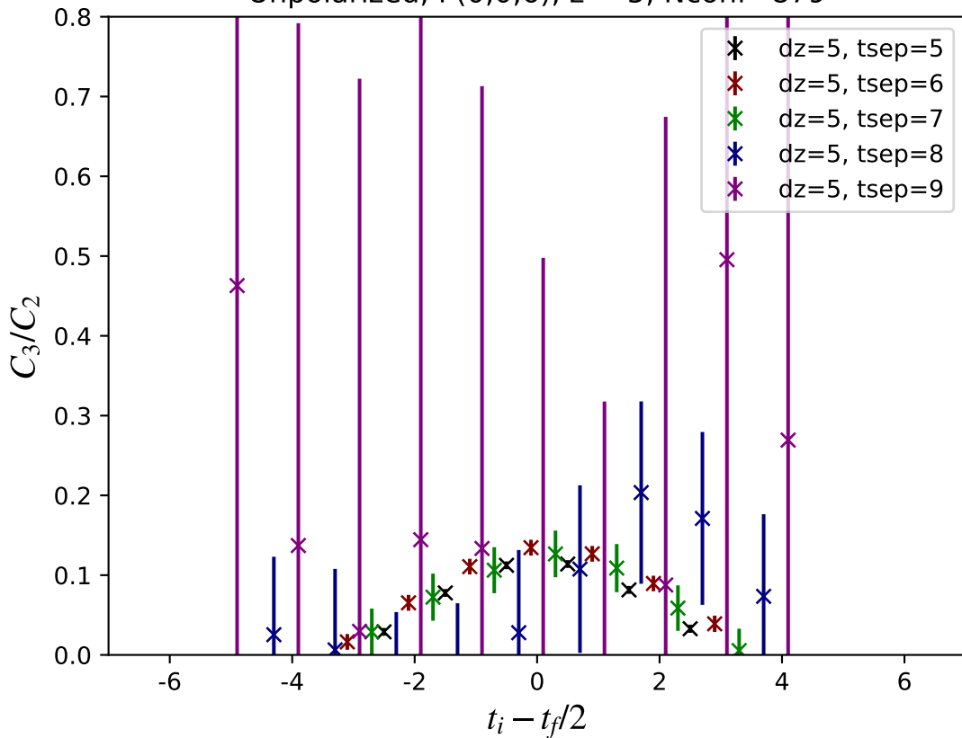
Unpolarized, P(0,0,6), z = 5 , Nconf=879
