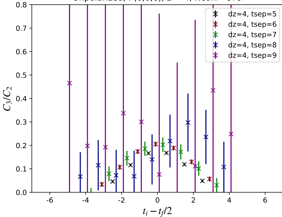
Unpolarized, P(0,0,6), z = 4 , Nconf=879
