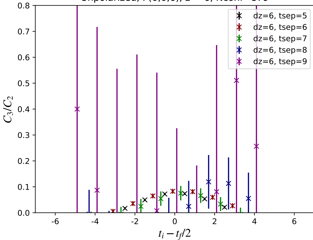
Unpolarized, P(0,0,6), z = 6 , Nconf=879
