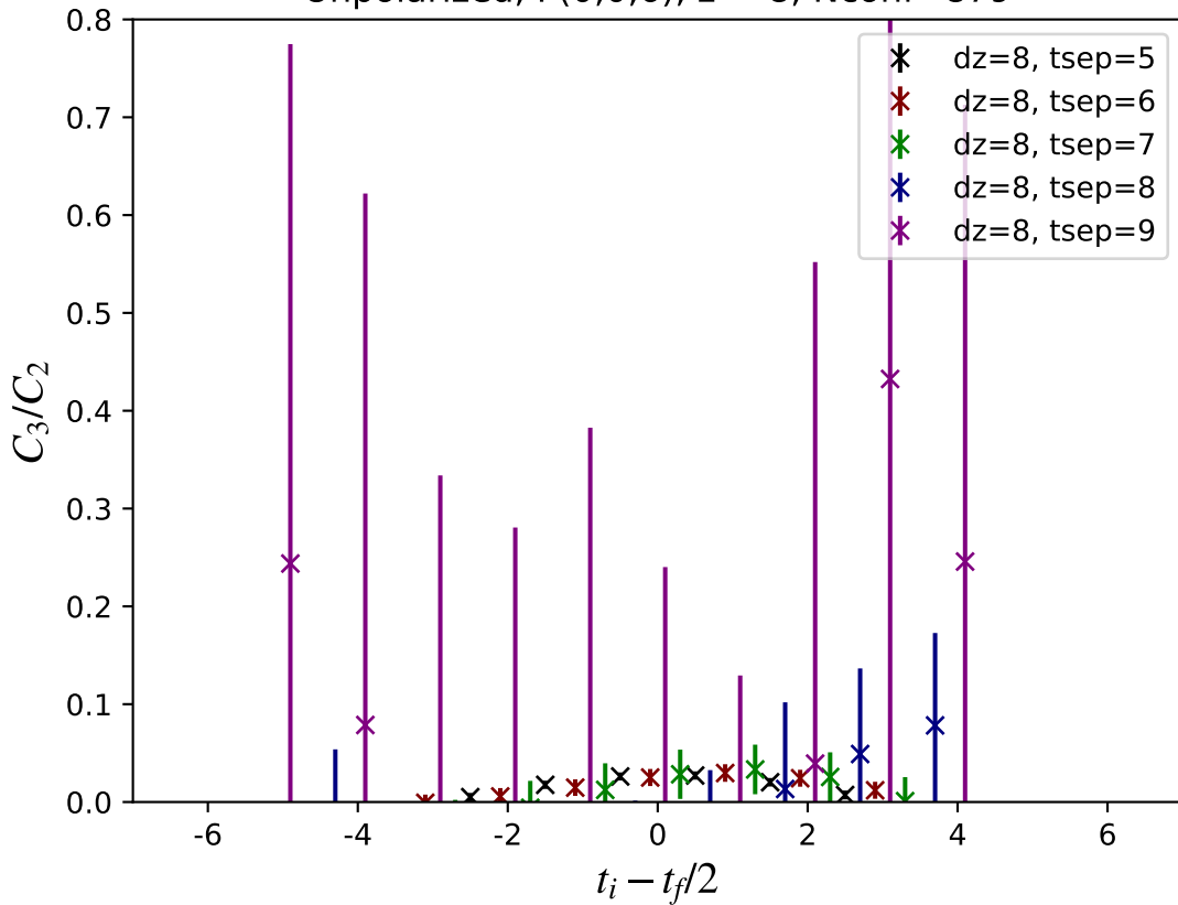
Unpolarized, P(0,0,6), z = 8 , Nconf=879
