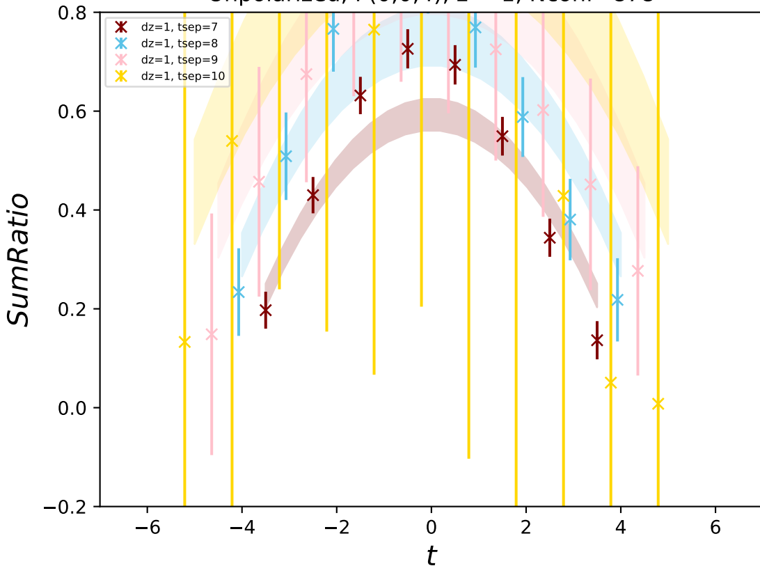
Unpolarized, P(0,0,4) , z = 1 , Nconf=878
