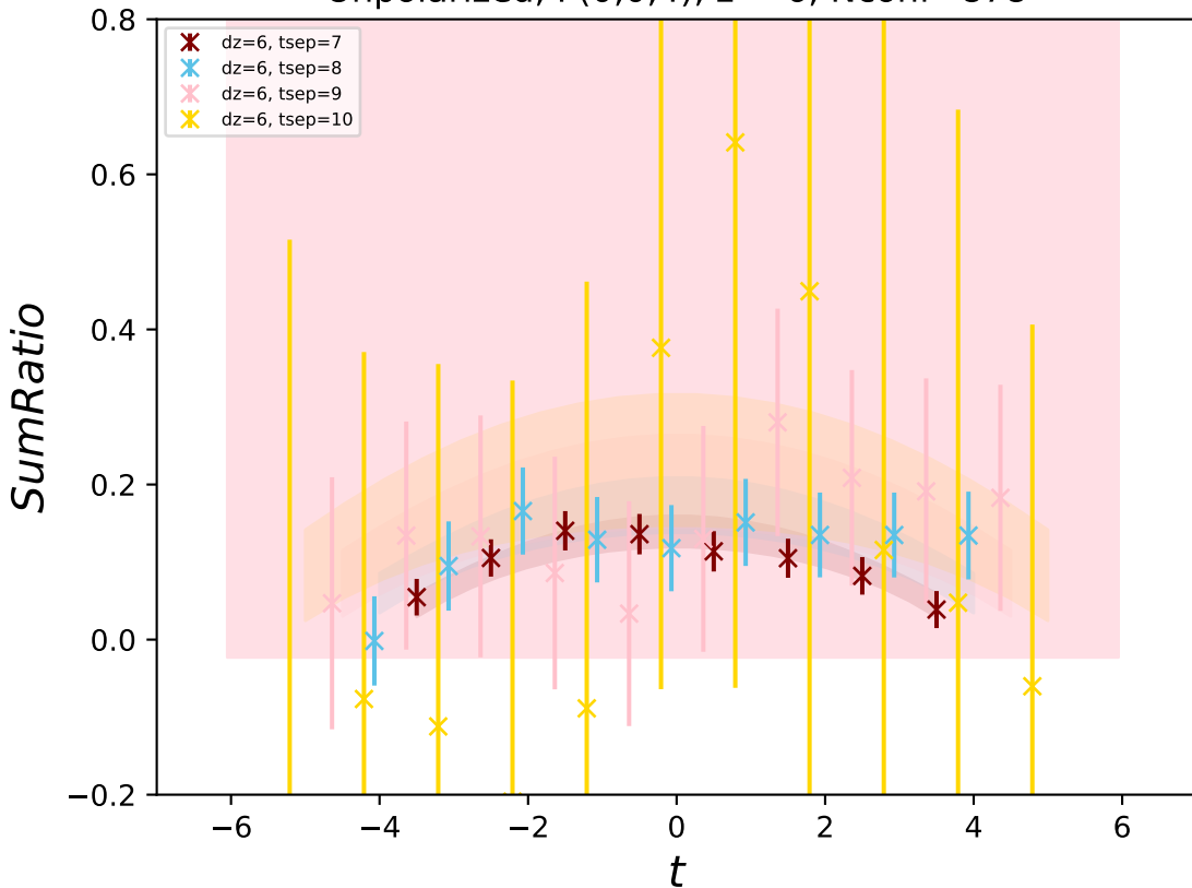
Unpolarized, P(0,0,4) , z = 6 , Nconf=878
