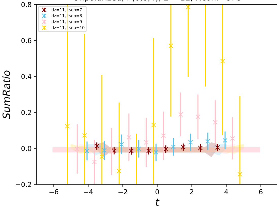
Unpolarized, P(0,0,4) , z = 11 , N_{\text{conf}}=878
