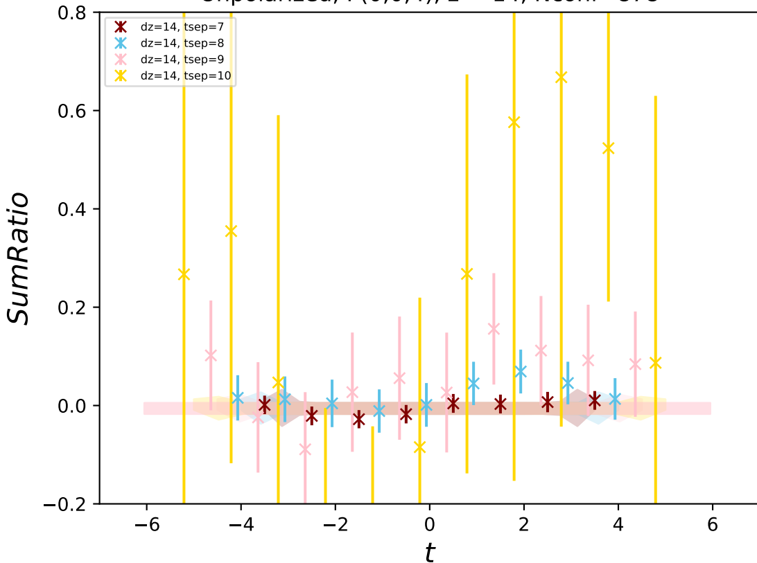
Unpolarized, P(0,0,4) , z = 14 , N_{\text{conf}}=878
