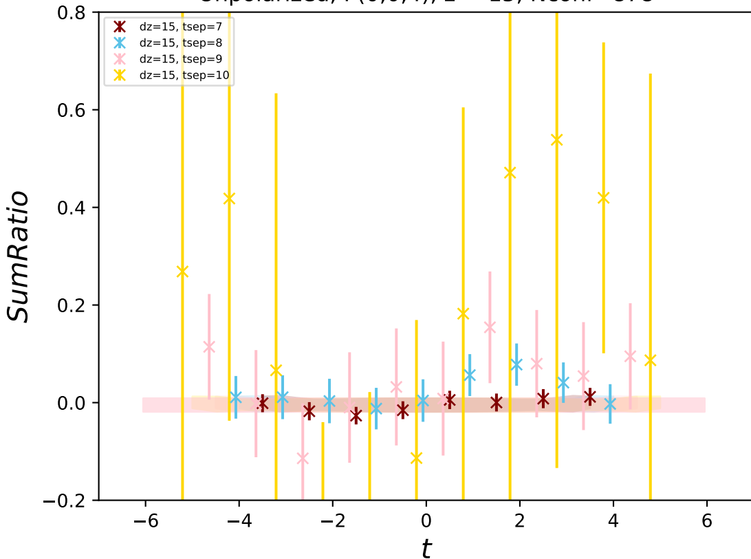
Unpolarized, P(0,0,4) , z = 15 , N_{\text{conf}}=878
