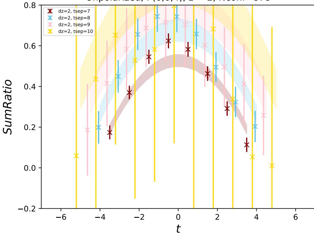
Unpolarized, P(0,0,4) , z = 2 , Nconf=878
