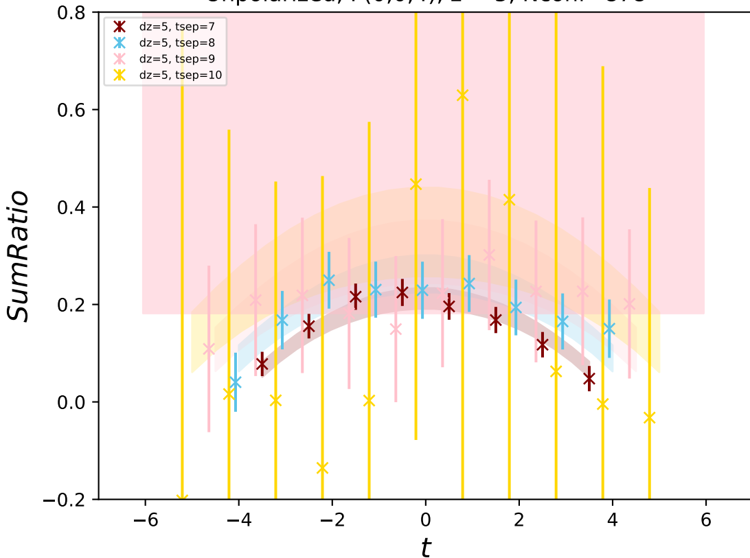
Unpolarized, P(0,0,4) , z = 5 , Nconf=878
