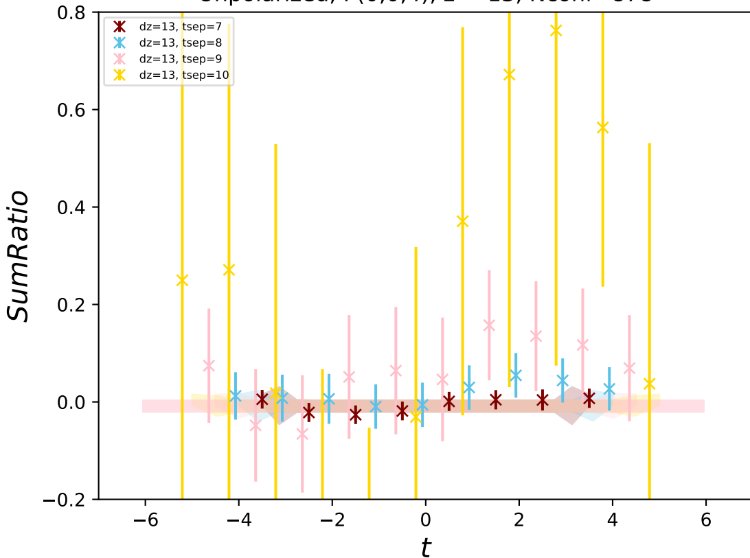
Unpolarized, P(0,0,4) , z = 13 , N_{\text{conf}}=878
