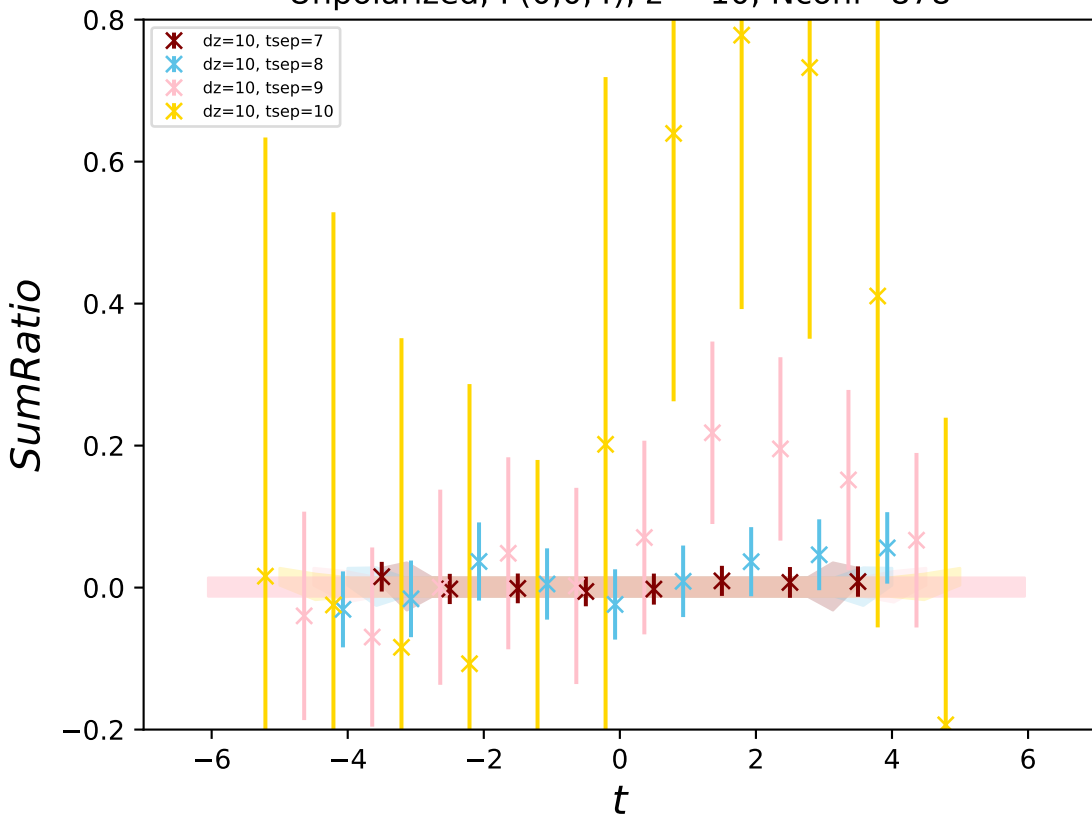
Unpolarized, P(0,0,4) , z = 10 , N_{\text{conf}}=878
