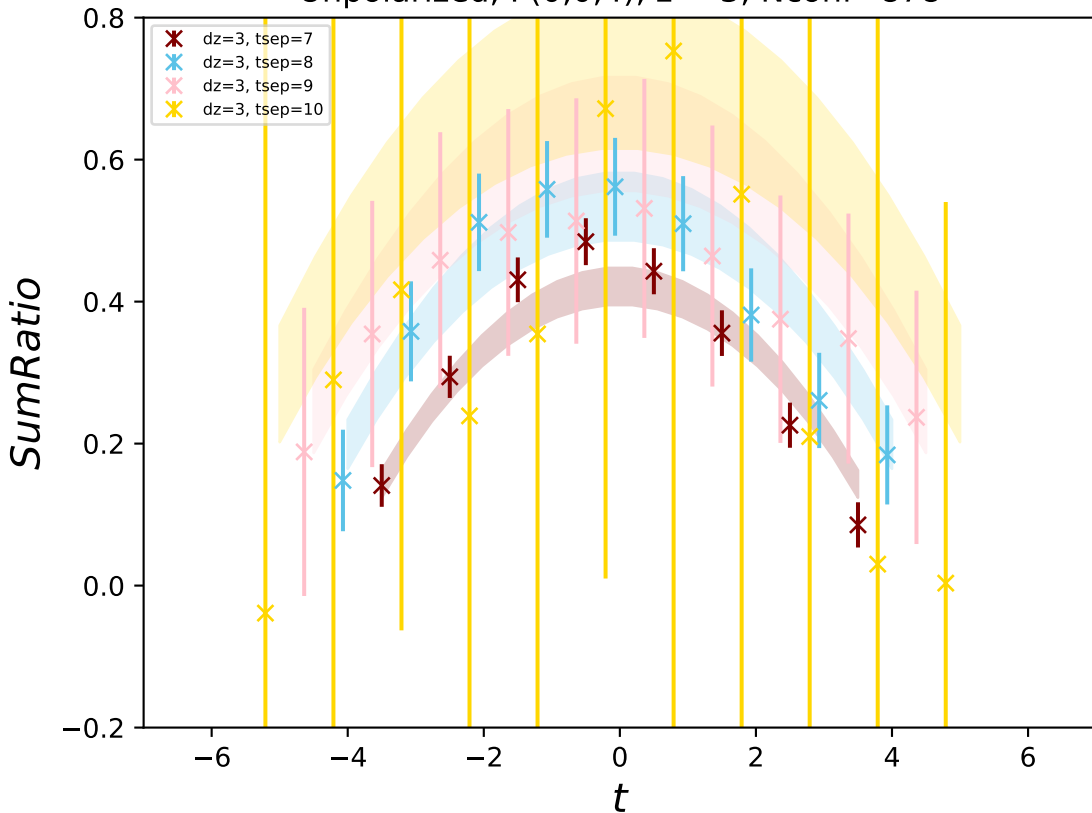
Unpolarized, P(0,0,4) , z = 3 , Nconf=878
