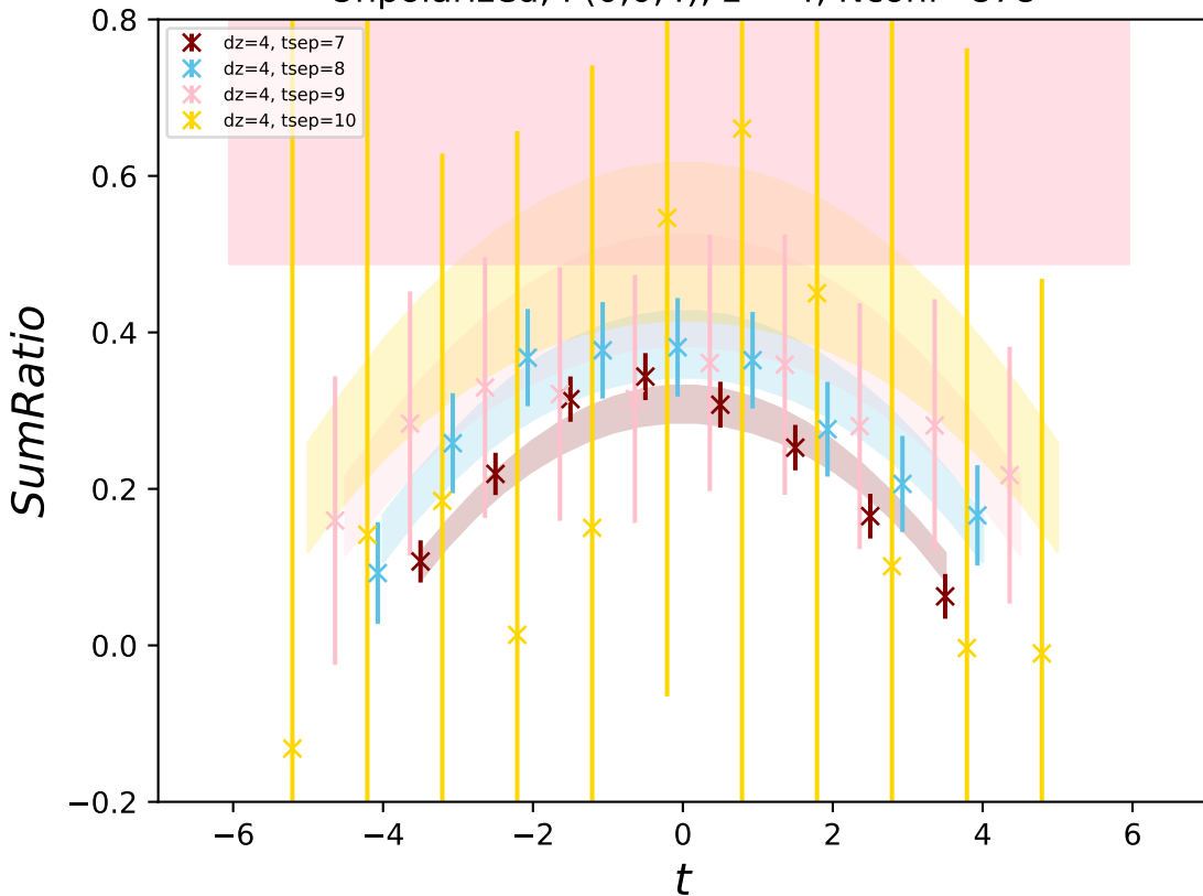
Unpolarized, P(0,0,4) , z = 4 , Nconf=878
