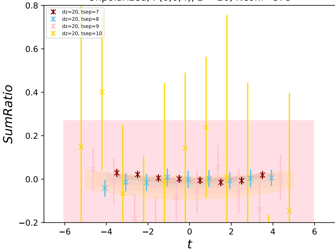
Unpolarized, P(0,0,4) , z = 20 , Nconf=878
