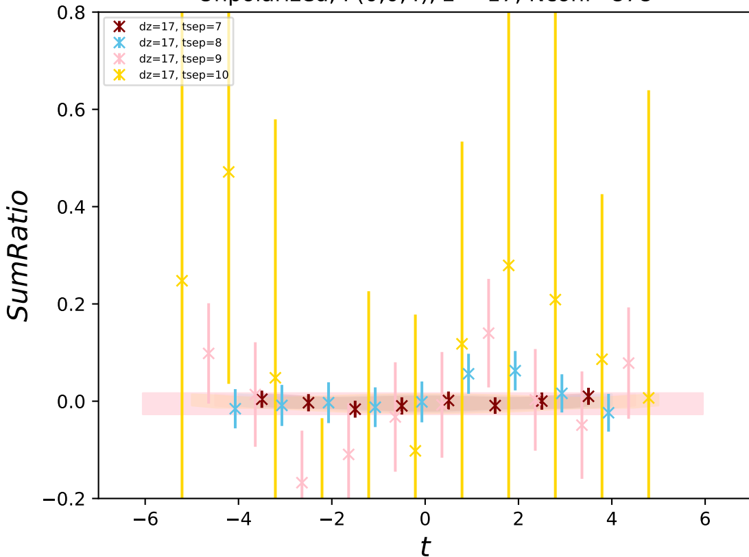
Unpolarized, P(0,0,4) , z = 17 , N_{\text{conf}}=878
