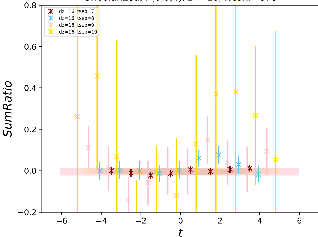
Unpolarized, P(0,0,4) , z = 16 , N_{\text{conf}}=878
