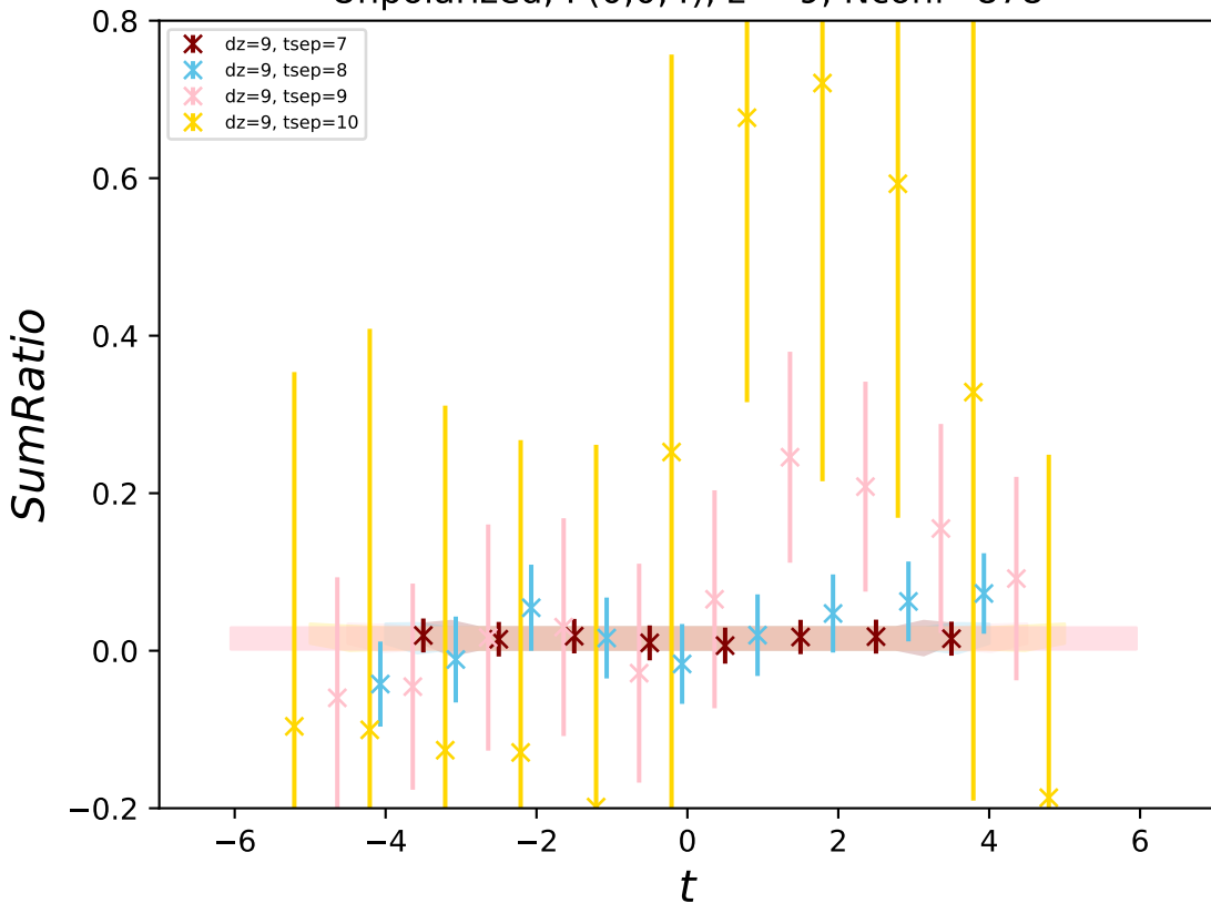
Unpolarized, P(0,0,4) , z = 9 , Nconf=878
