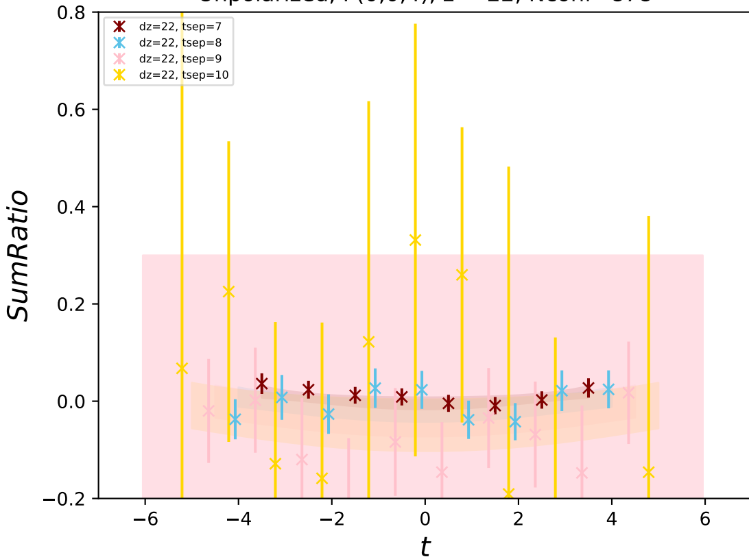
Unpolarized, P(0,0,4) , z = 22 , N_{\text{conf}}=878
