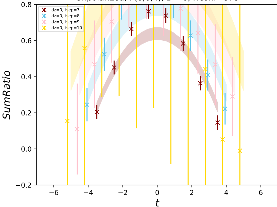
Unpolarized, P(0,0,4) , z = 0 , Nconf=878
