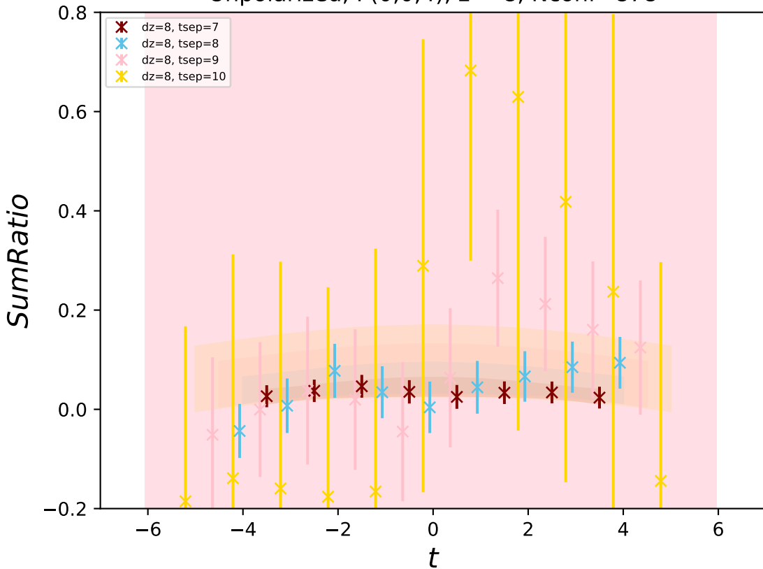
Unpolarized, P(0,0,4) , z = 8 , Nconf=878
