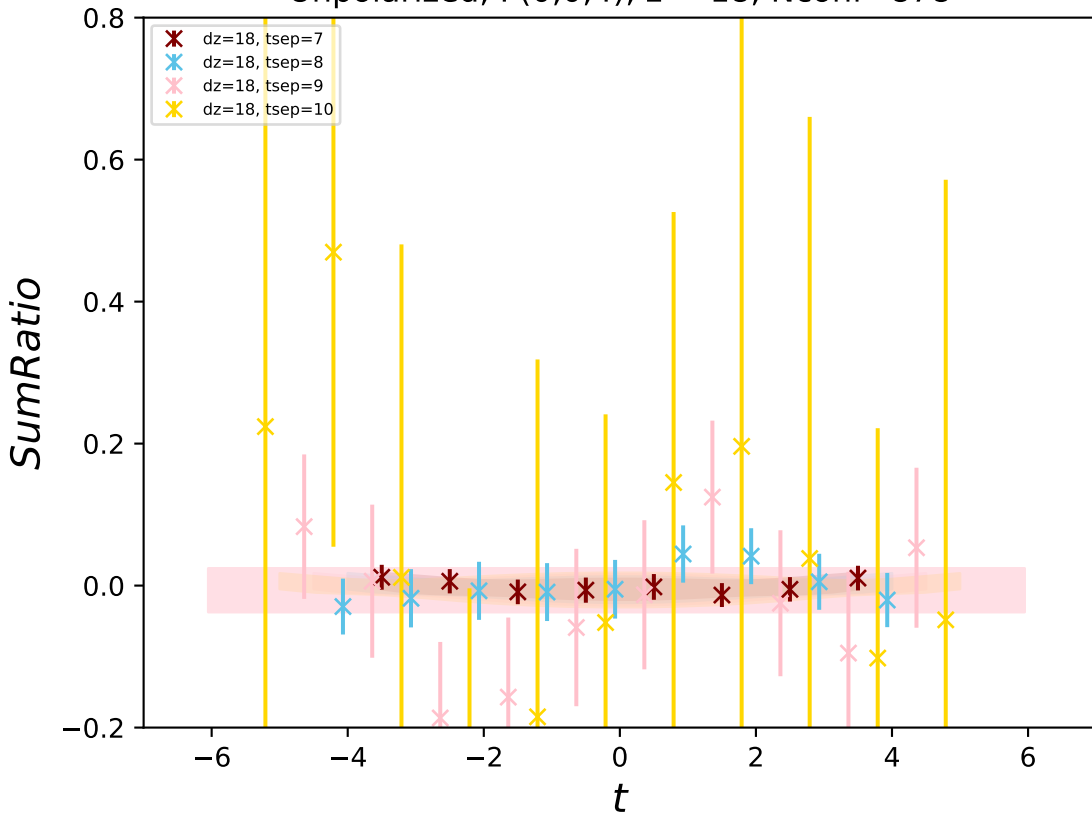
Unpolarized, P(0,0,4) , z = 18 , Nconf=878
