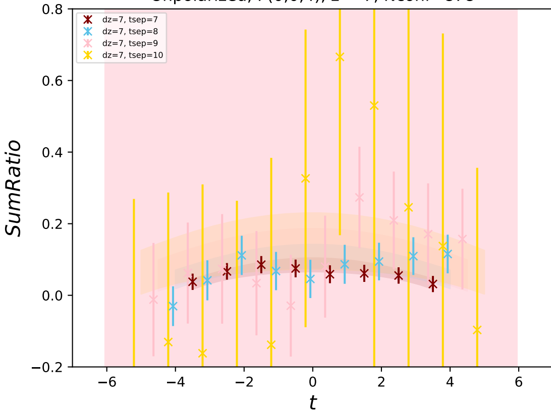
Unpolarized, P(0,0,4) , z = 7 , Nconf=878
