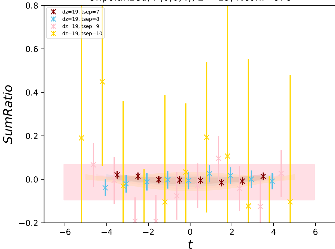
Unpolarized, P(0,0,4) , z = 19 , Nconf=878
