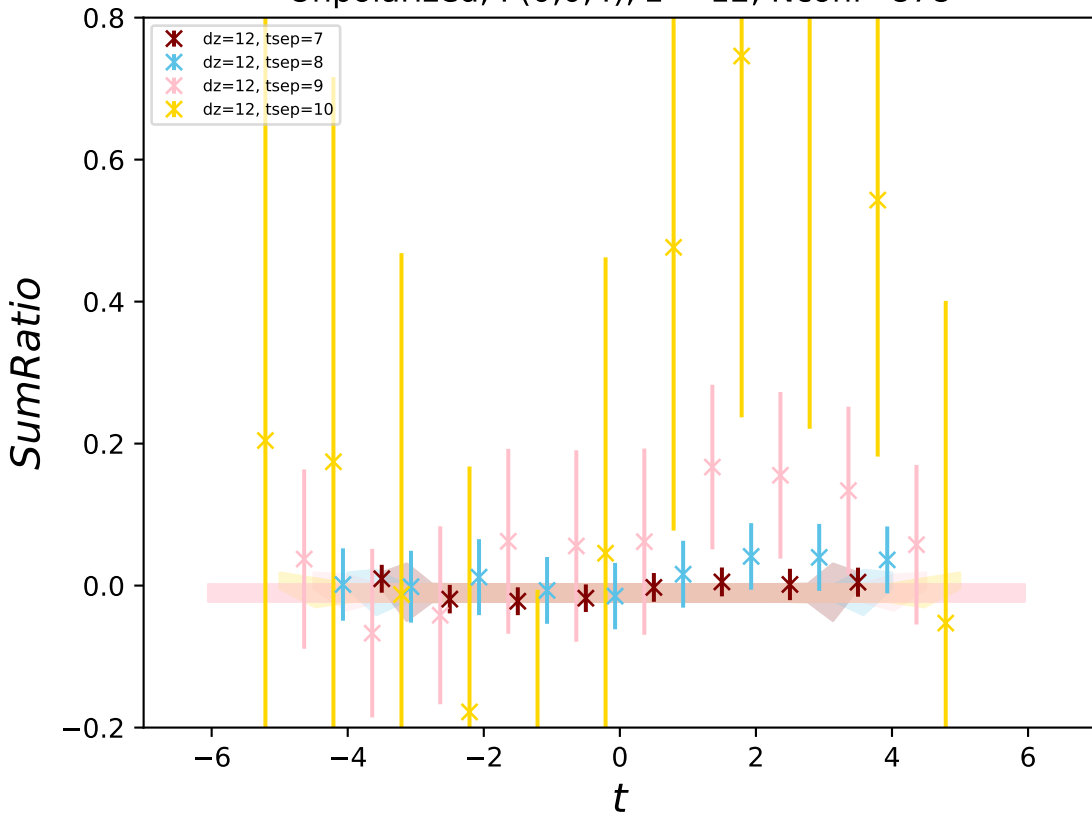
Unpolarized, P(0,0,4) , z = 12 , Nconf=878
