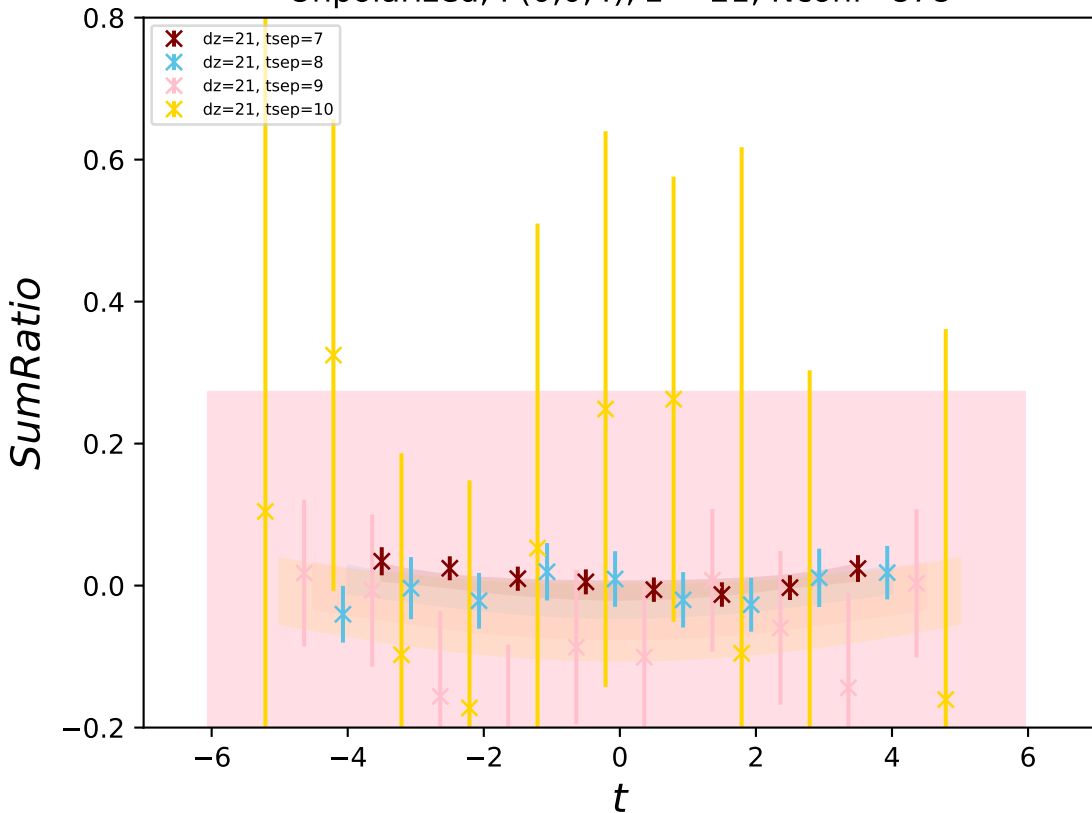
Unpolarized, P(0,0,4) , z = 21 , Nconf=878
