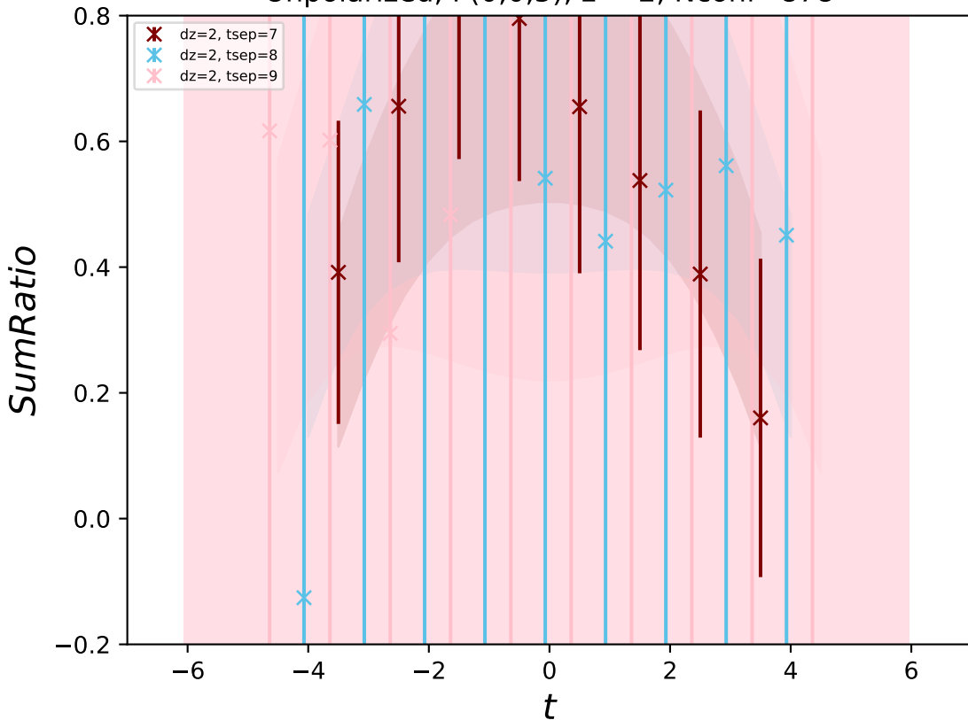
Unpolarized, P(0,0,5) , z = 2 , Nconf=878
