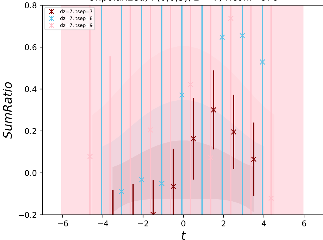
Unpolarized, P(0,0,5) , z = 7 , N_{\text{conf}}=878
