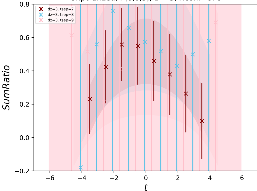
Unpolarized, P(0,0,5) , z = 3 , Nconf=878
