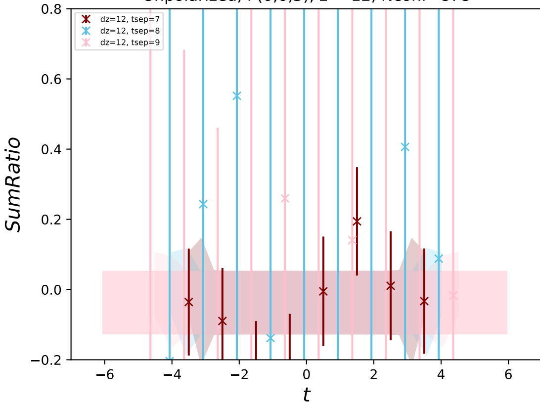
Unpolarized, P(0,0,5) , z = 12 , Nconf=878
