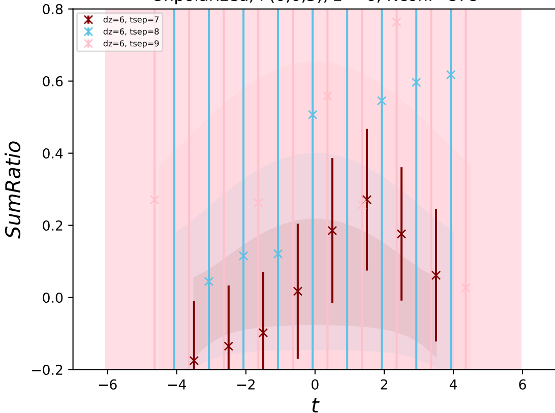
Unpolarized, P(0,0,5), z = 6 , Nconf=878
