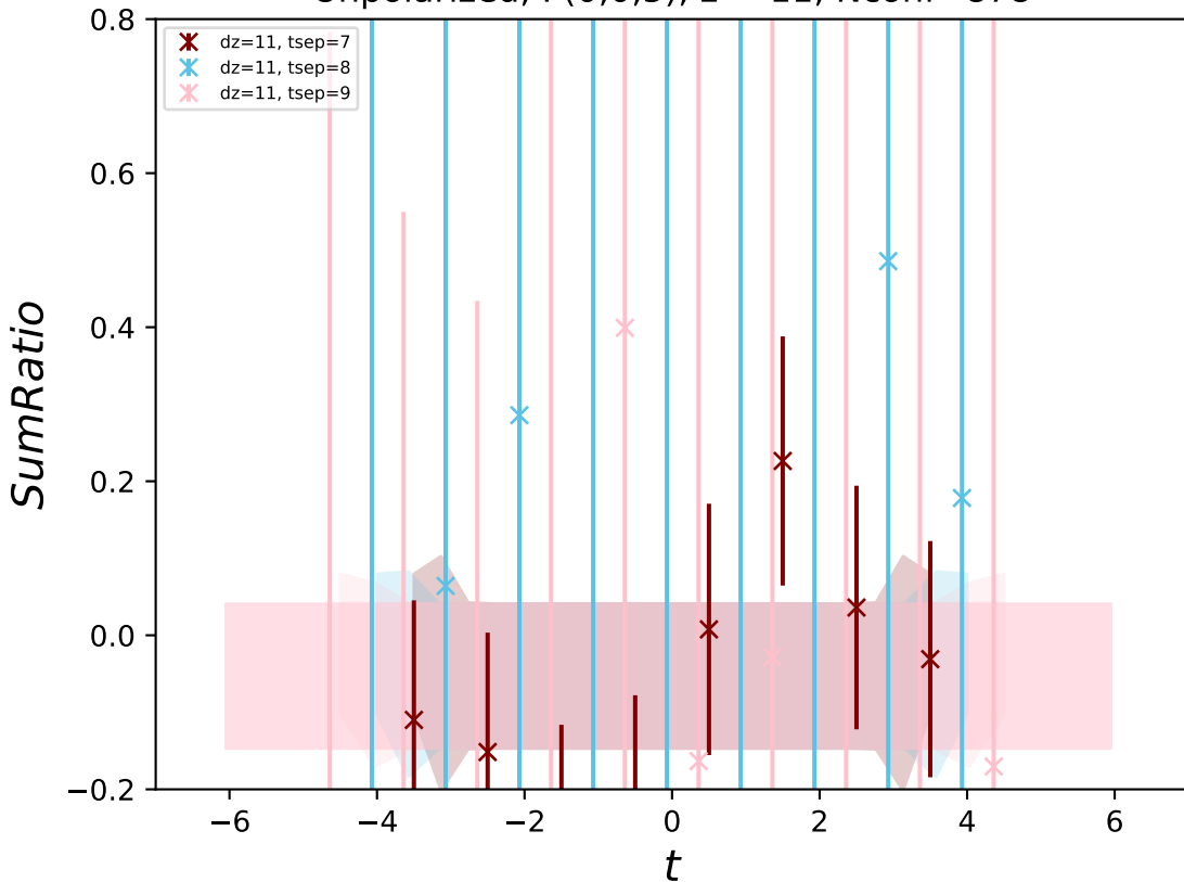
Unpolarized, P(0,0,5) , z = 11 , Nconf=878
