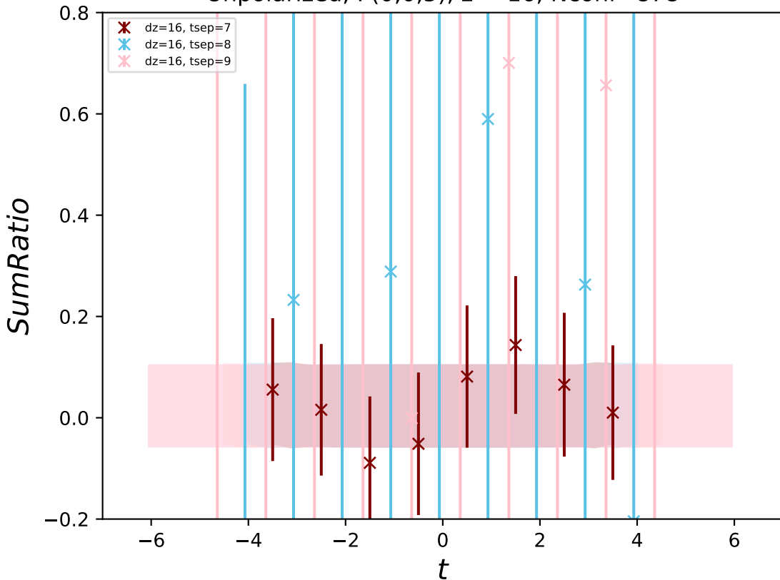
Unpolarized, P(0,0,5) , z = 16 , N_{\text{conf}}=878
