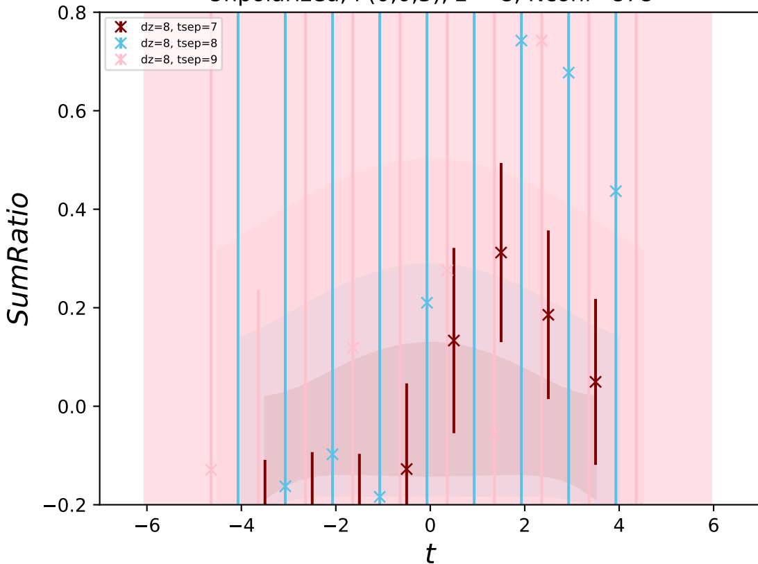
Unpolarized, P(0,0,5) , z = 8 , Nconf=878
