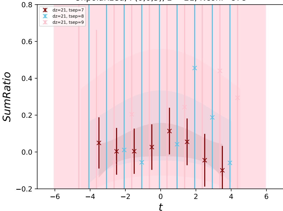
Unpolarized, P(0,0,5) , z = 21 , Nconf=878
