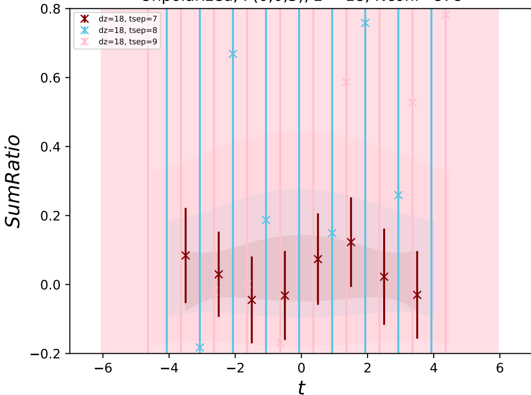
Unpolarized, P(0,0,5) , z = 18 , Nconf=878
