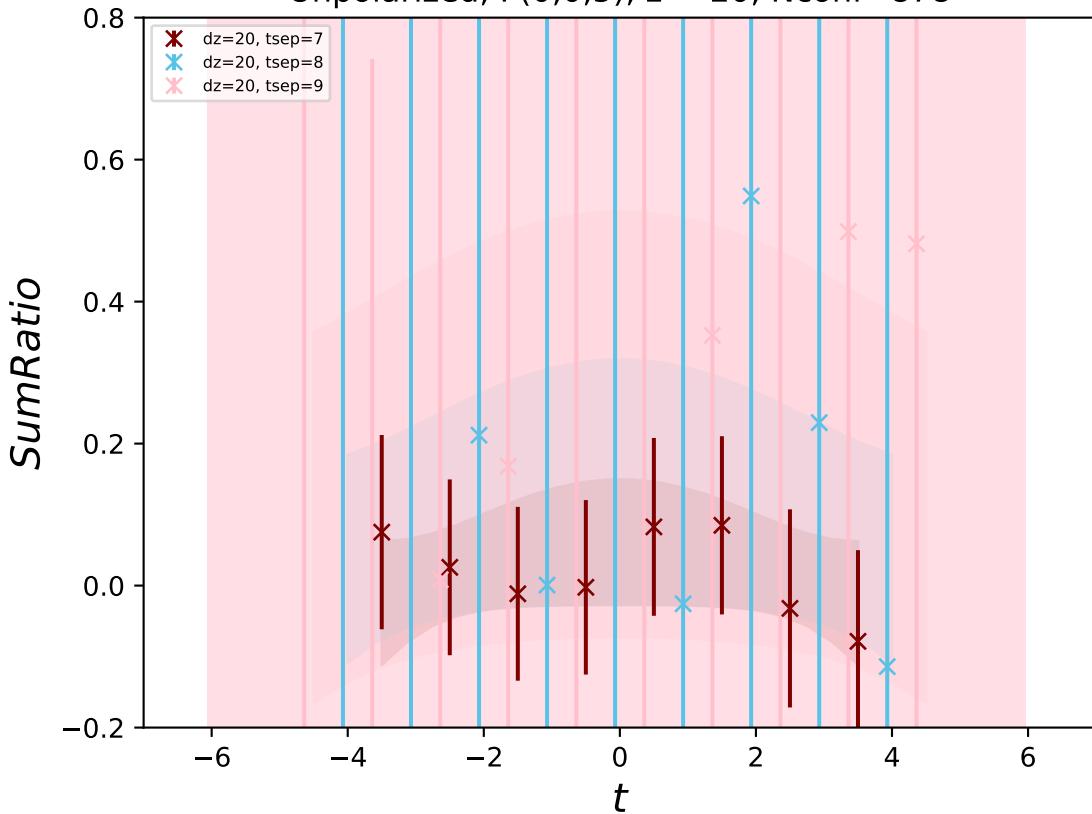
Unpolarized, P(0,0,5) , z = 20 , Nconf=878
