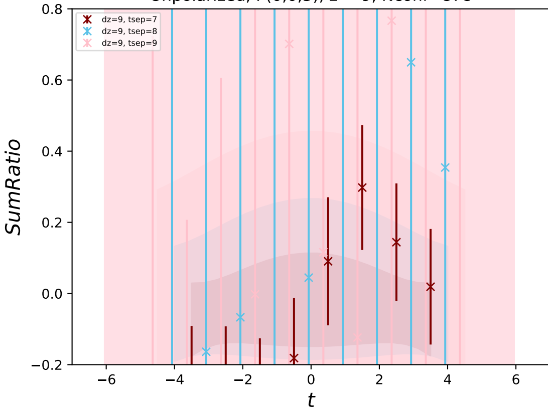
Unpolarized, P(0,0,5) , z = 9 , N_{\text{conf}}=878
