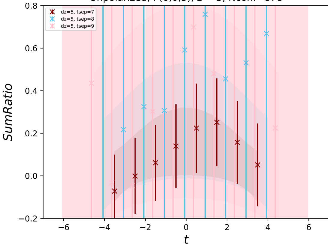
Unpolarized, P(0,0,5) , z = 5 , N_{\text{conf}}=878
