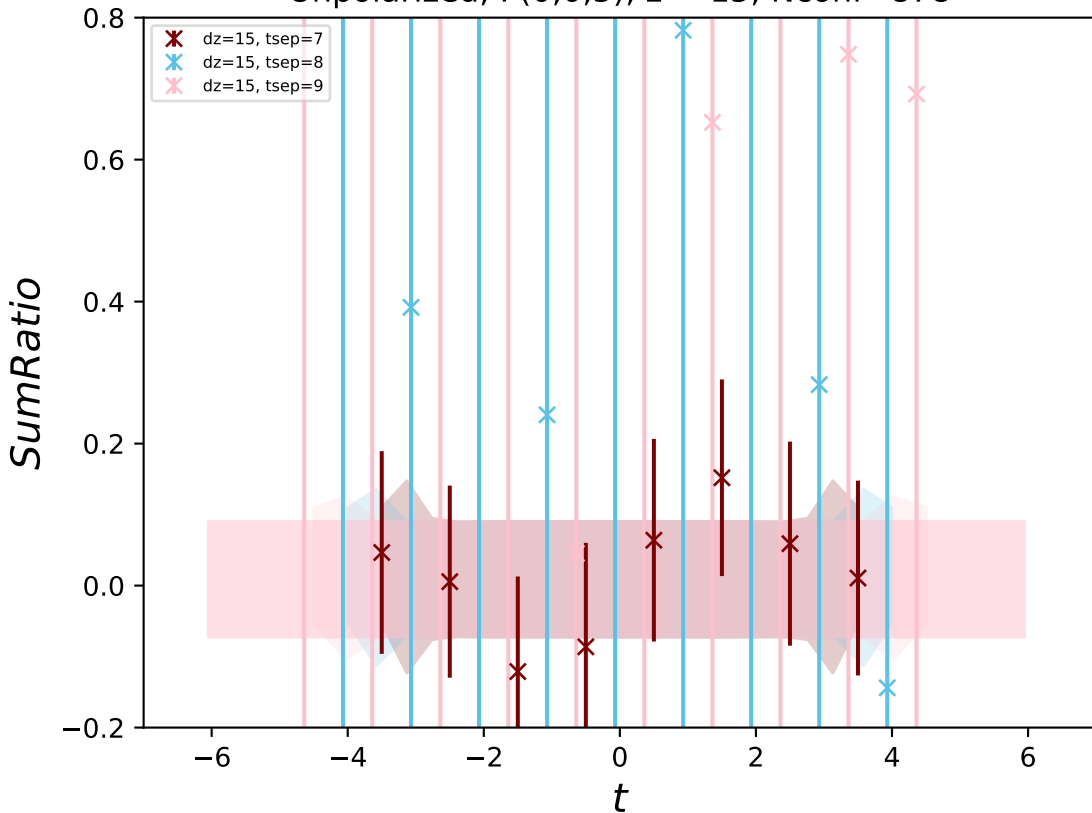
Unpolarized, P(0,0,5) , z = 15 , N_{\text{conf}}=878
