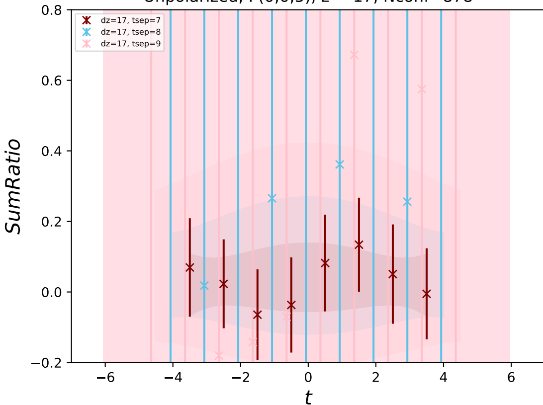
Unpolarized, P(0,0,5) , z = 17 , Nconf=878
