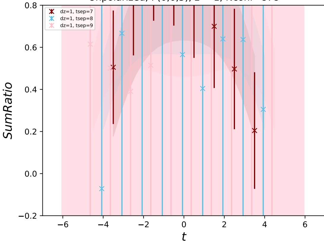
Unpolarized, P(0,0,5), z = 1 , Nconf=878
