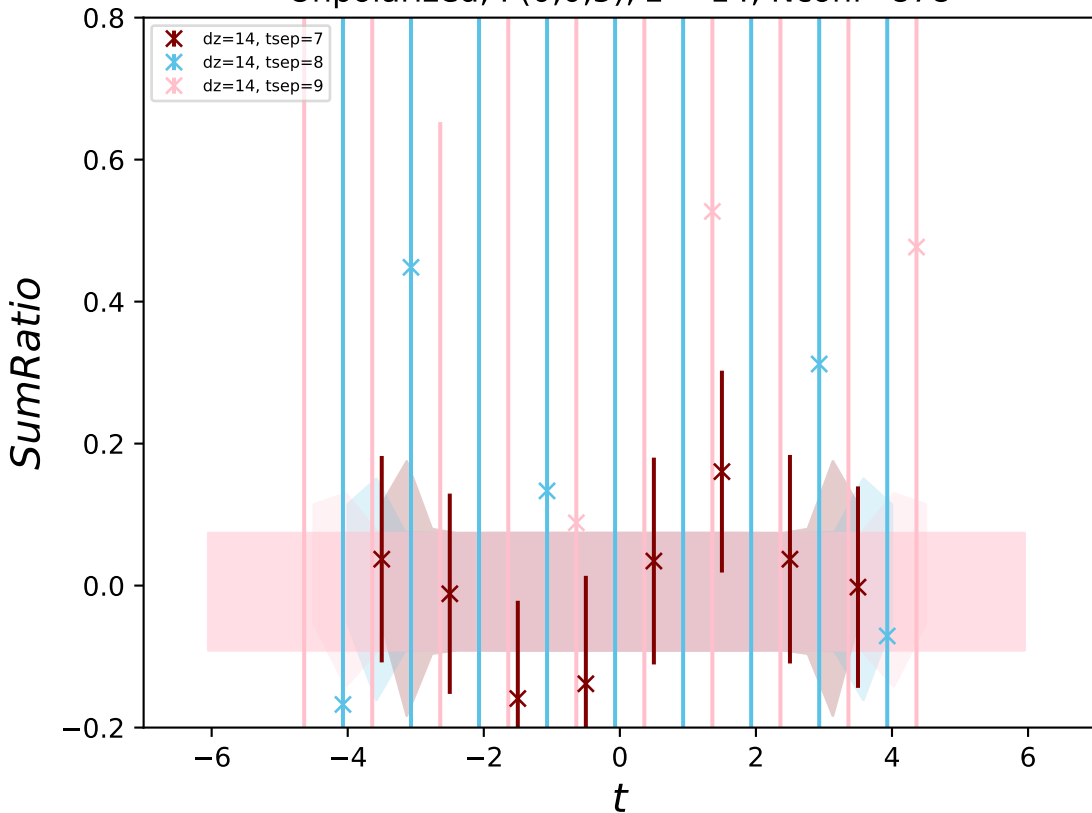
Unpolarized, P(0,0,5) , z = 14 , Nconf=878
