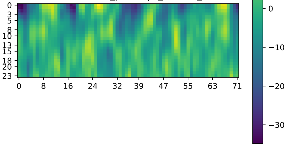
Real Part of two_point/ops_L24x72_dhx
