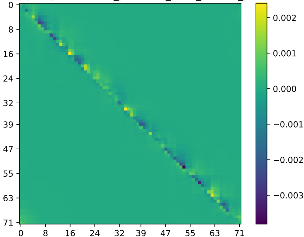
Imaginary Part of two_point/two_point_L24x72_cc
