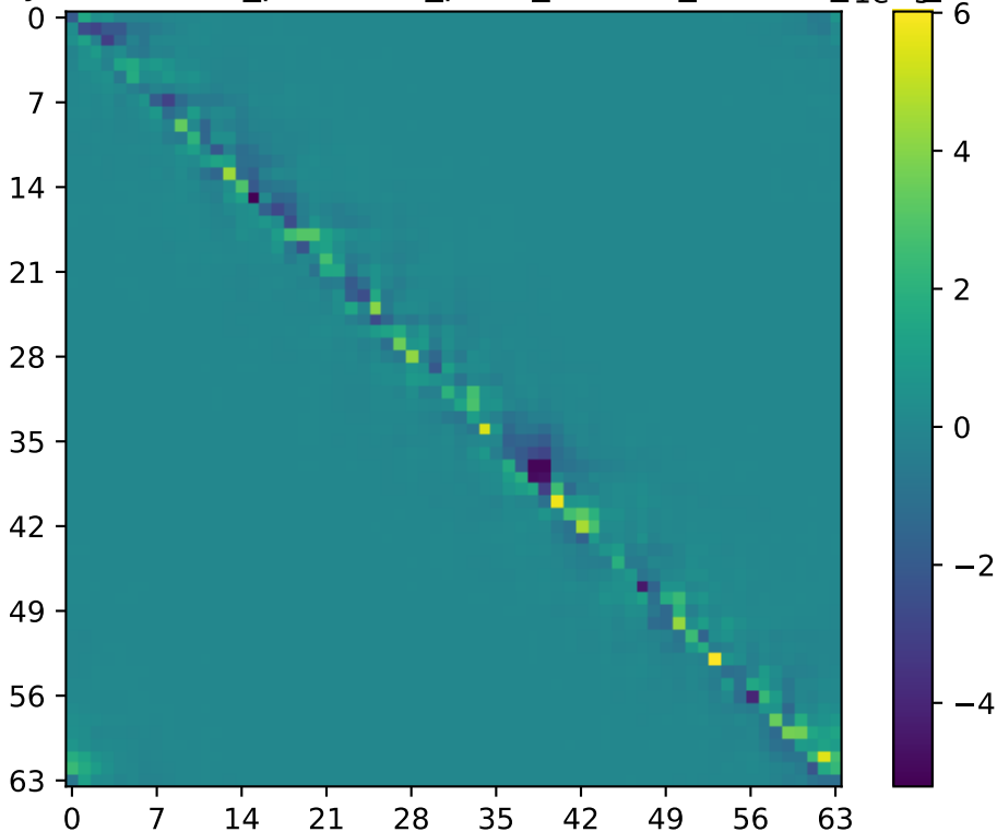
Imaginary Part of two_point/two_point_L32x64_C32P23_GPD 5 mean
