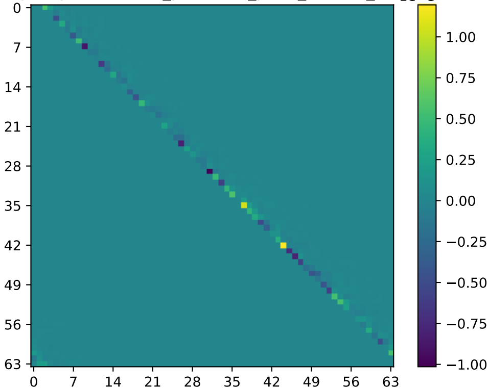
Imaginary Part of two_point/two_point_L32x64_C32x64_P23
