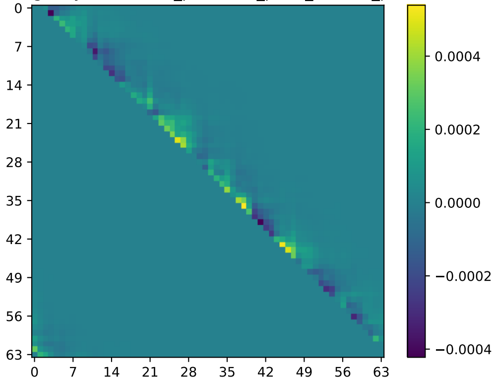
Imaginary Part of two_point/two_point_L32x64_plus
