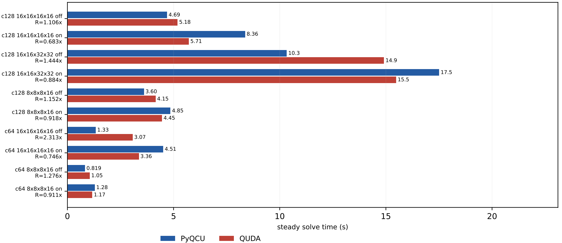
P100 absolute MG-3 steady times mass=0.050, block=2x2x2x2, nvec=12
