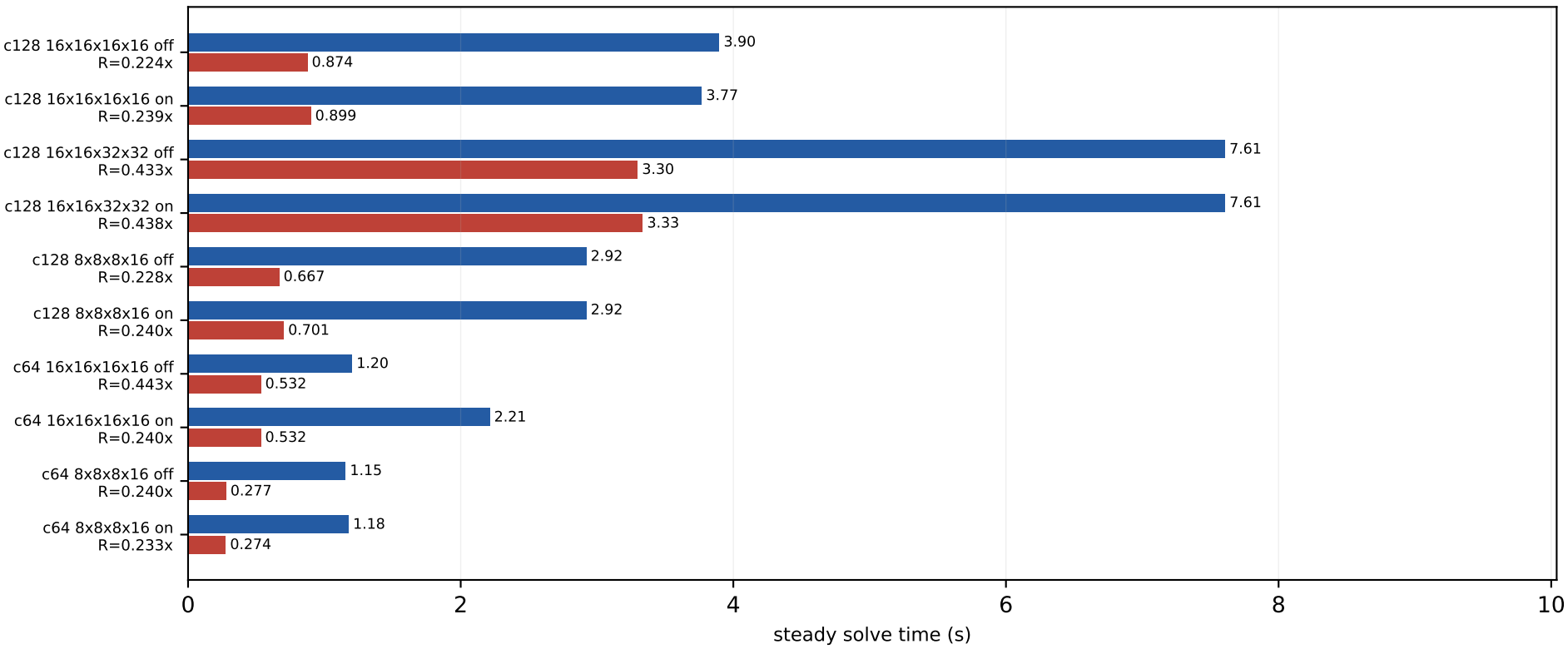
P100 absolute BiCGStab steady times mass=0.050, block=2x2x2x2, nvec=12
