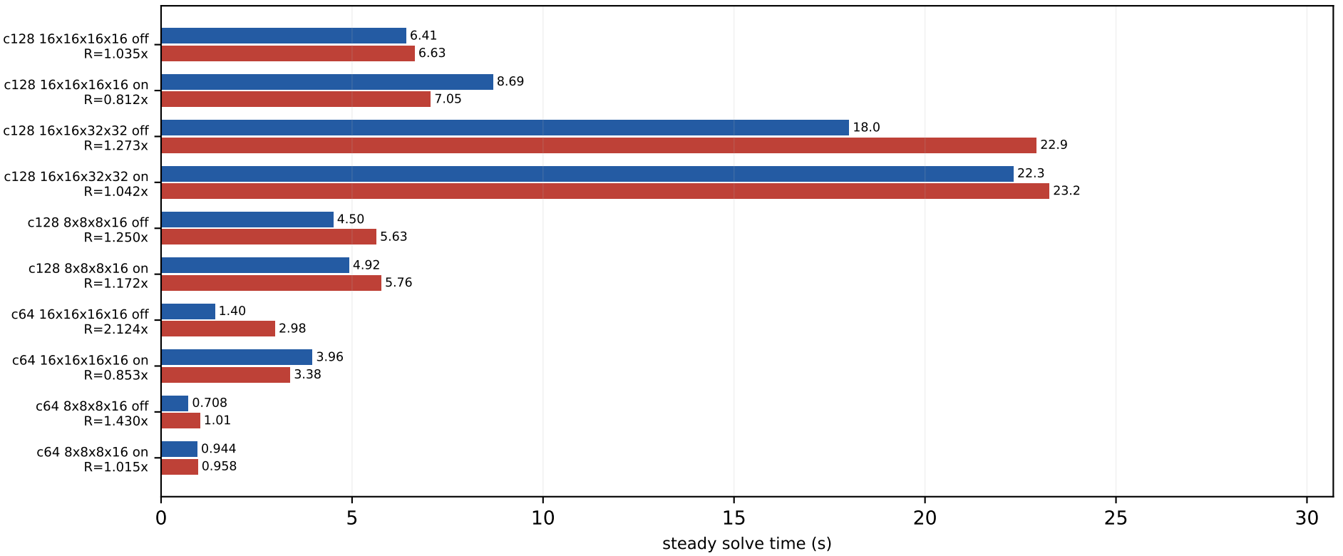
P100 absolute MG-2 steady times mass=0.050, block=2x2x2x2, nvec=12
