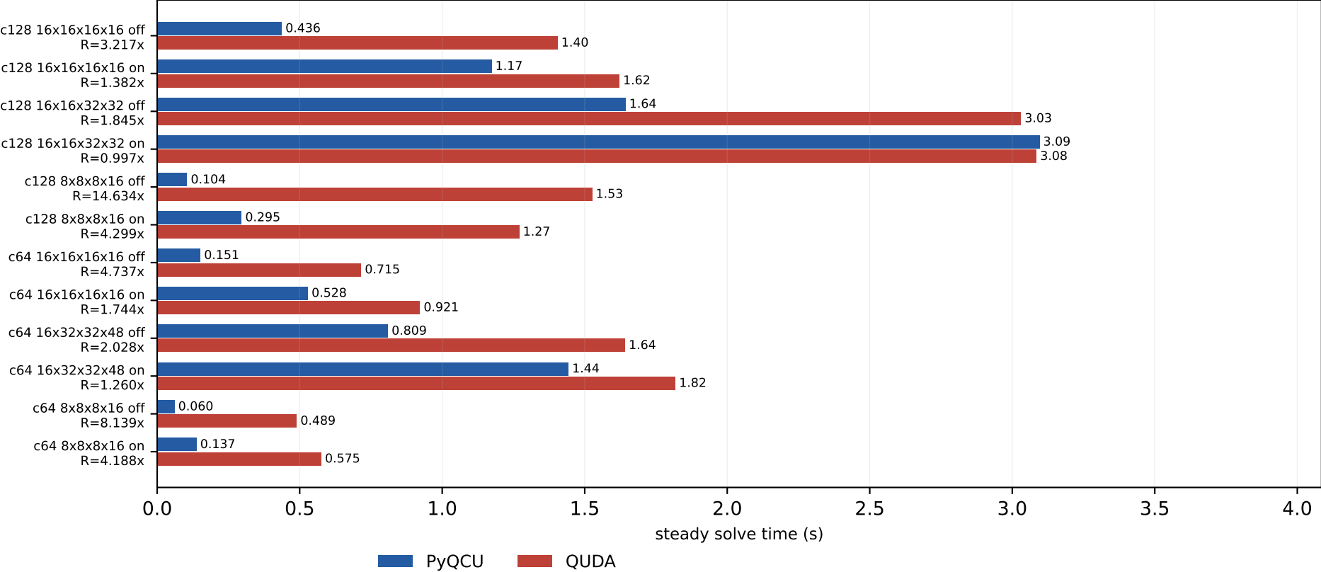
V100 absolute MG-3 steady times mass=0.050, block=2x2x2x2, nvec=12
