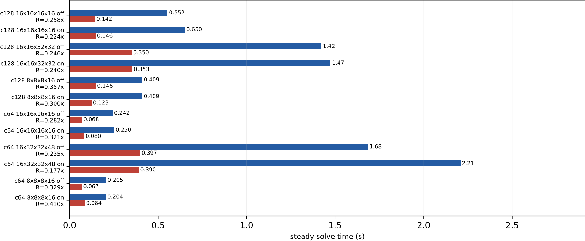
V100 absolute BiCGStab steady times mass=0.050, block=2x2x2x2, nvec=12
