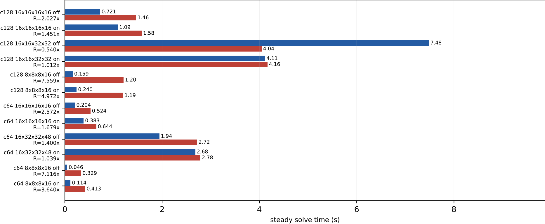
V100 absolute MG-2 steady times mass=0.050, block=2x2x2x2, nvec=12
