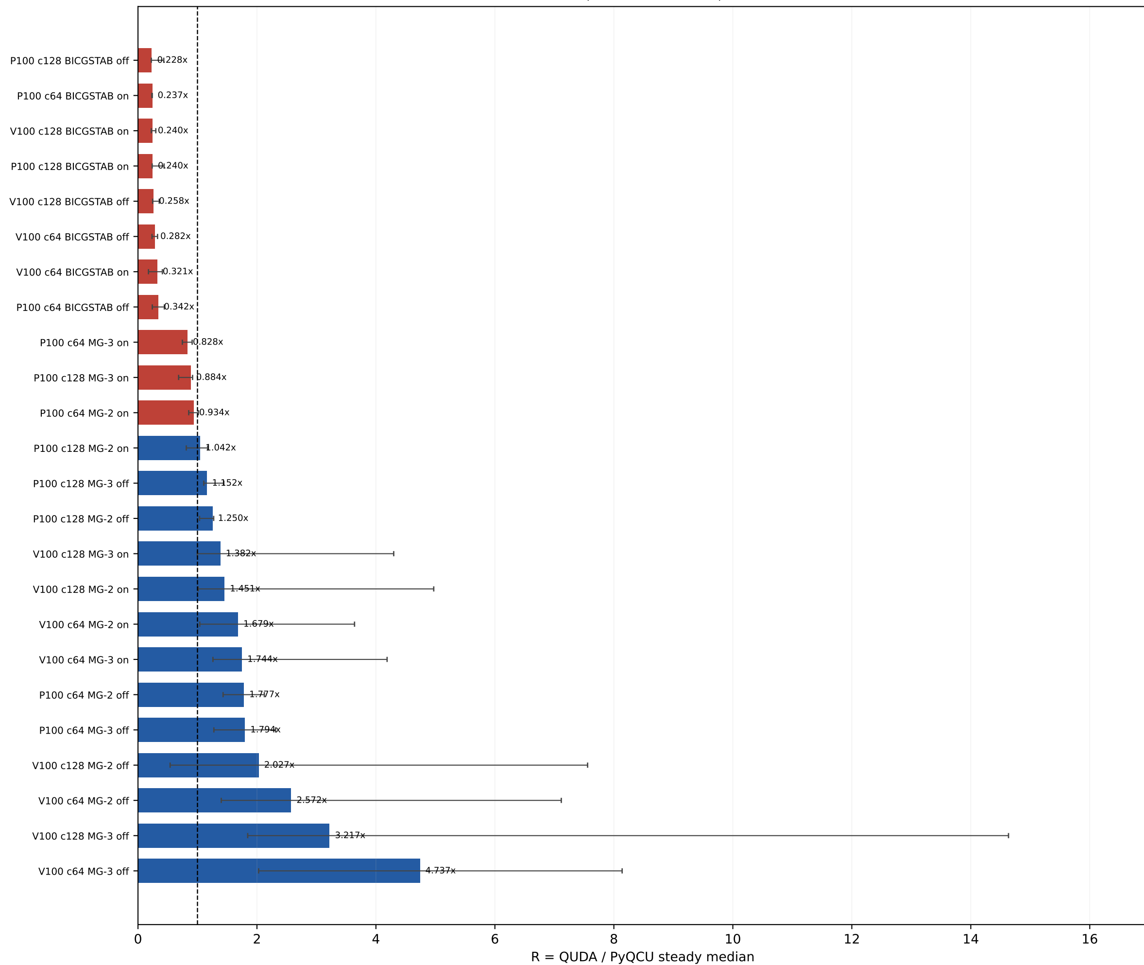
Group median time ratio with min-max range mass=0.050, block=2x2x2x2, nvec=12
