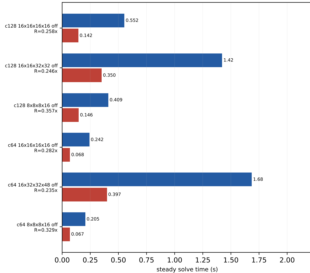
V100 BiCGStab trace-off absolute times mass=0.050, block=2x2x2x2, nvec=12
