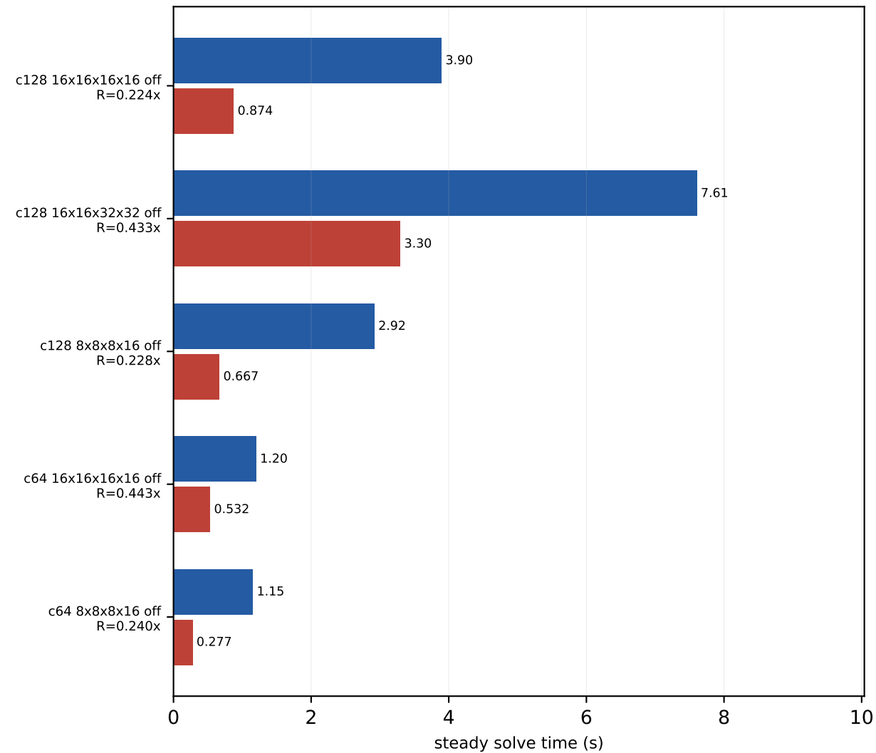
P100 BiCGStab trace-off absolute times mass=0.050, block=2x2x2x2, nvec=12
