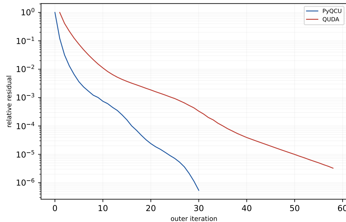
P100 c64 16x16x16x16 MG-2 trace-on mass=0.050, block=2x2x2x2, nvec=12
