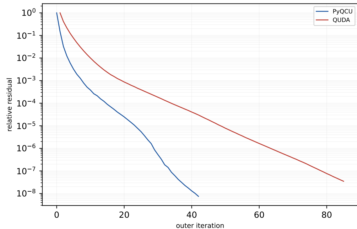
P100 c128 16x16x32x32 MG-2 trace-on mass=0.050, block=2x2x2x2, nvec=12
