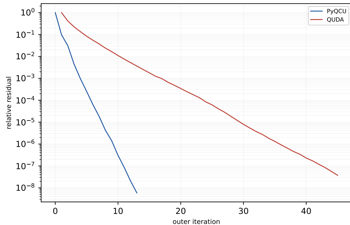
P100 c128 8x8x8x16 MG-2 trace-on mass=0.050, block=2x2x2x2, nvec=12
