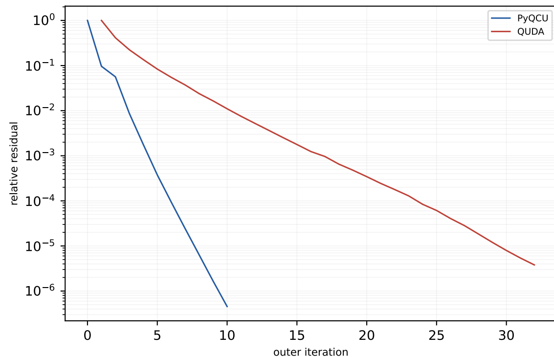
P100 c64 8x8x8x16 MG-2 trace-on mass=0.050, block=2x2x2x2, nvec=12
