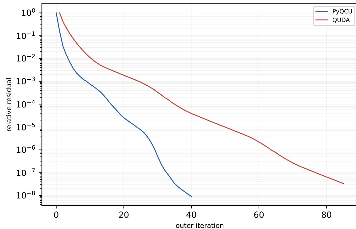
P100 c128 16x16x16x16 MG-2 trace-on mass=0.050, block=2x2x2x2, nvec=12
