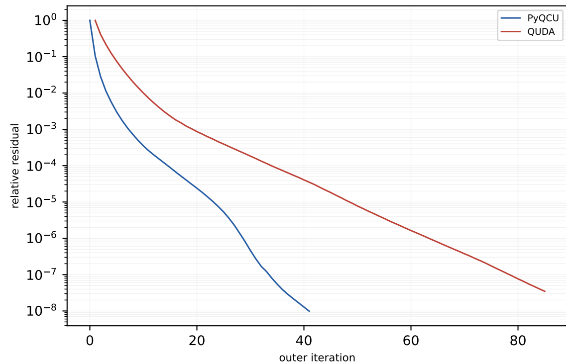
V100 c128 16x16x32x32 MG-2 trace-on mass=0.050, block=2x2x2x2, nvec=12
