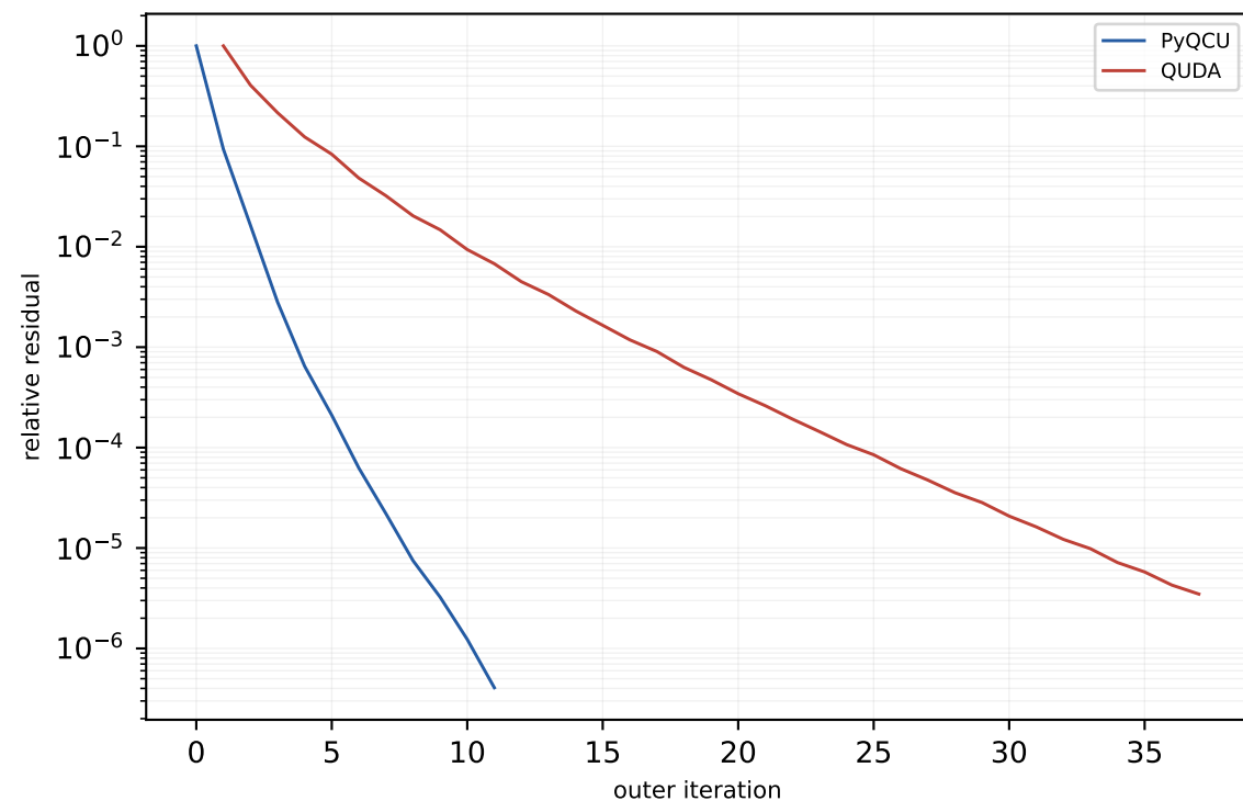
V100 c64 16x32x32x48 MG-2 trace-on mass=0.050, block=2x2x2x2, nvec=12
