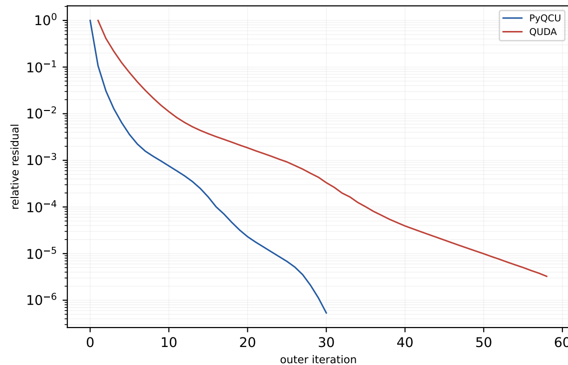
V100 c64 16x16x16x16 MG-2 trace-on mass=0.050, block=2x2x2x2, nvec=12
