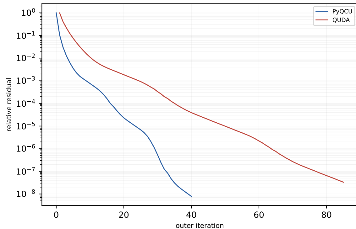
V100 c128 16x16x16x16 MG-2 trace-on mass=0.050, block=2x2x2x2, nvec=12
