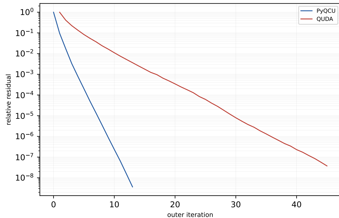
V100 c128 8x8x8x16 MG-2 trace-on mass=0.050, block=2x2x2x2, nvec=12
