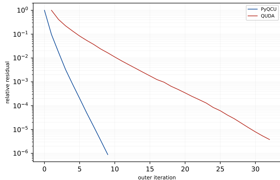
V100 c64 8x8x8x16 MG-2 trace-on mass=0.050, block=2x2x2x2, nvec=12
