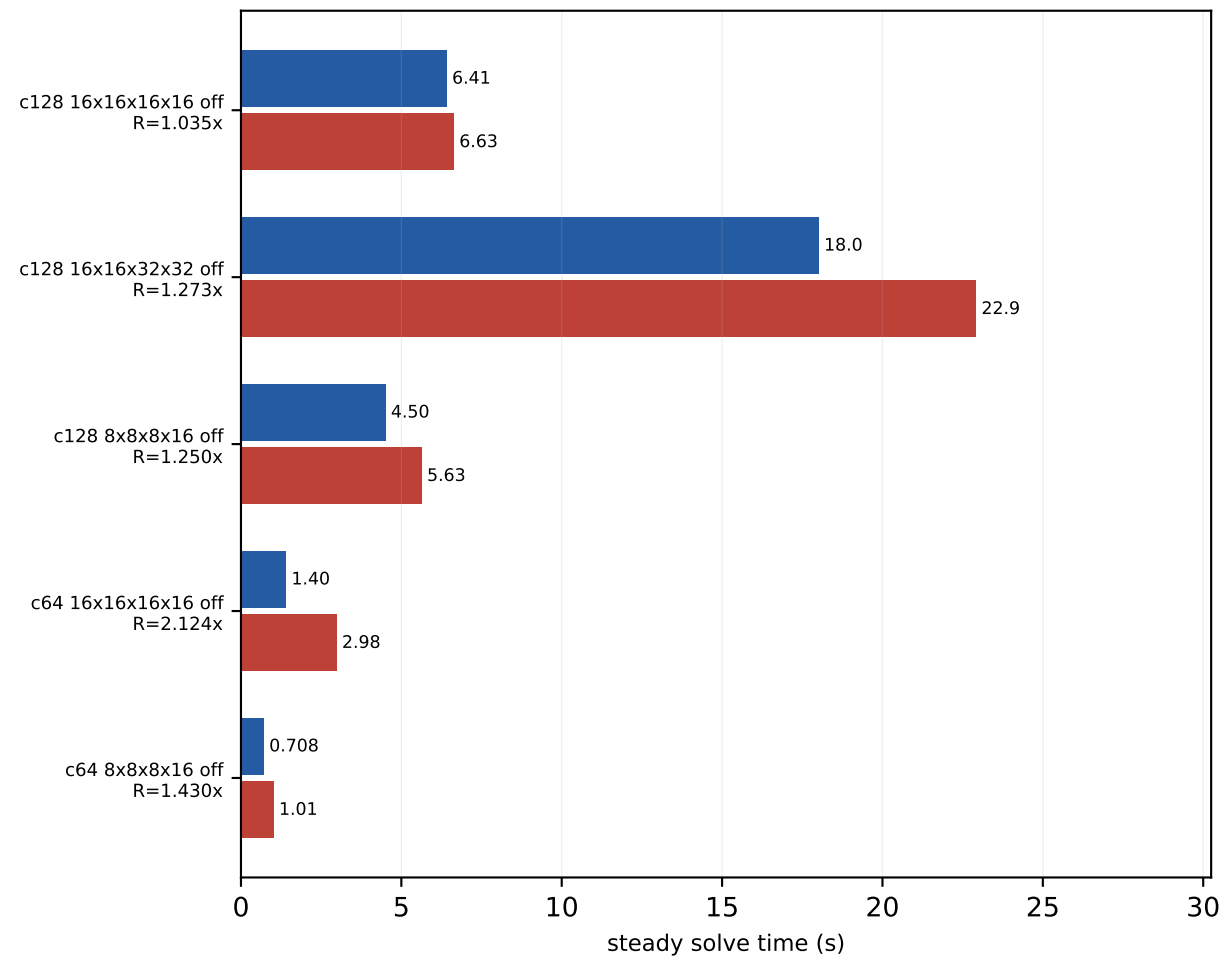
P100 MG-2 trace-off absolute times mass=0.050, block=2x2x2x2, nvec=12
