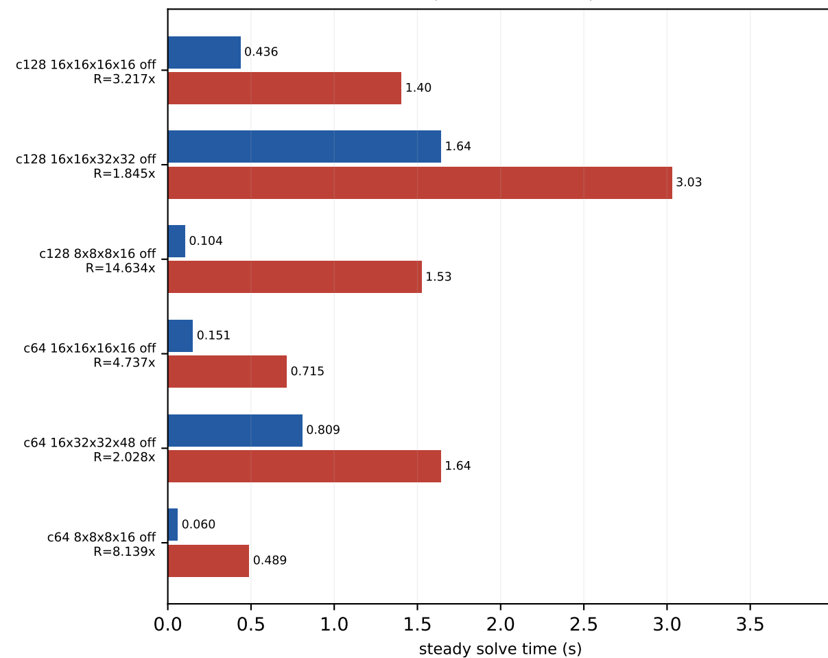
V100 MG-3 trace-off absolute times mass=0.050, block=2x2x2x2, nvec=12
