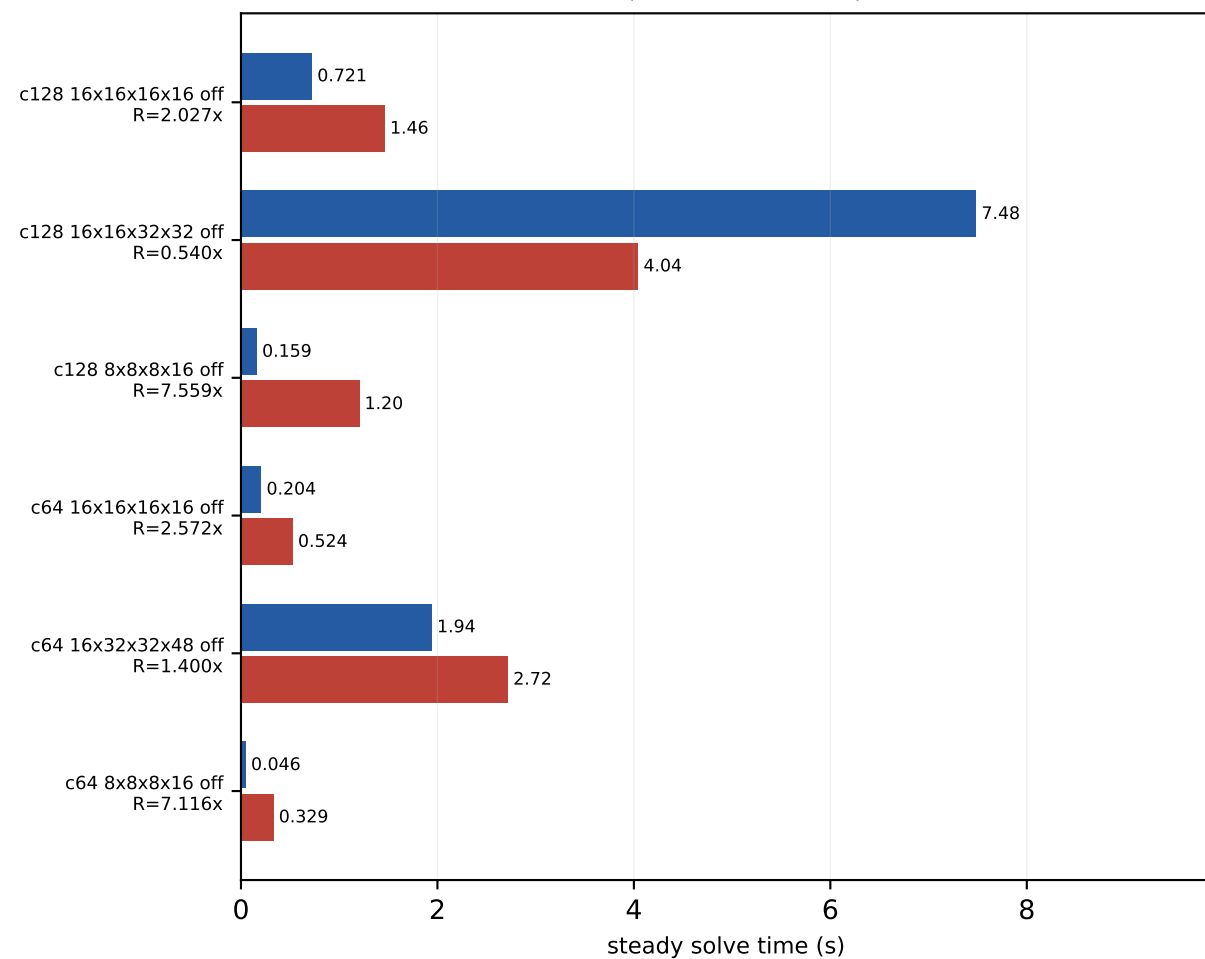
V100 MG-2 trace-off absolute times mass=0.050, block=2x2x2x2, nvec=12
