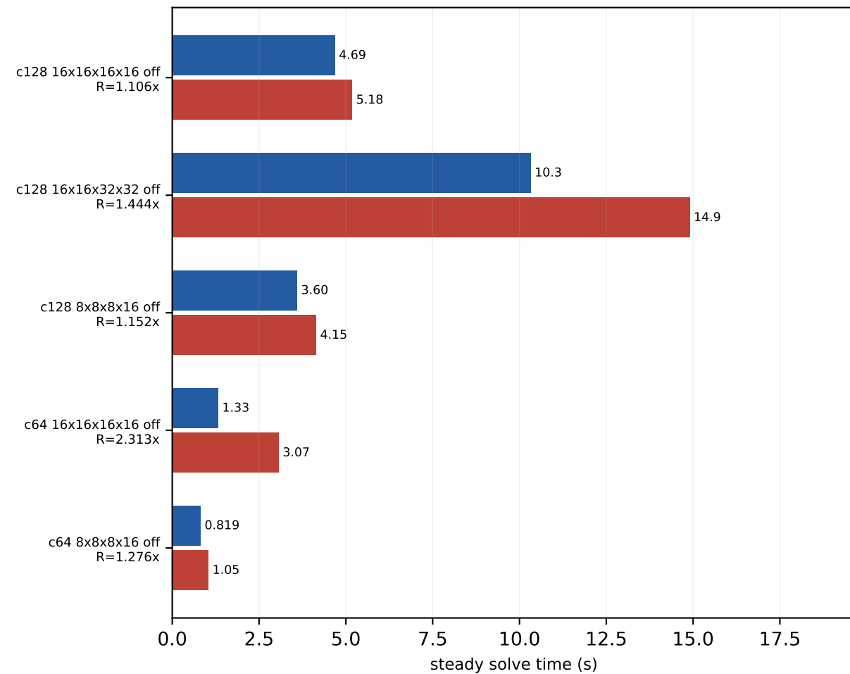
P100 MG-3 trace-off absolute times mass=0.050, block=2x2x2x2, nvec=12
