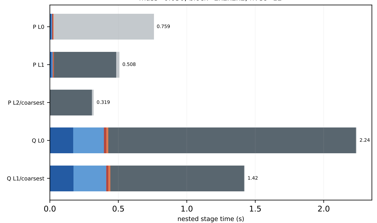
V100 c64 8x8x8x16 MG-3 trace-on mass=0.050, block=2x2x2x2, nvec=12
