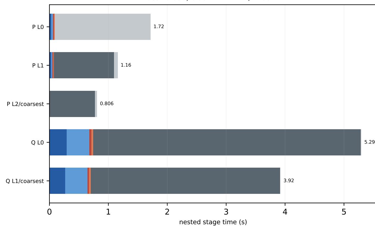
V100 c128 8x8x8x16 MG-3 trace-on mass=0.050, block=2x2x2x2, nvec=12
