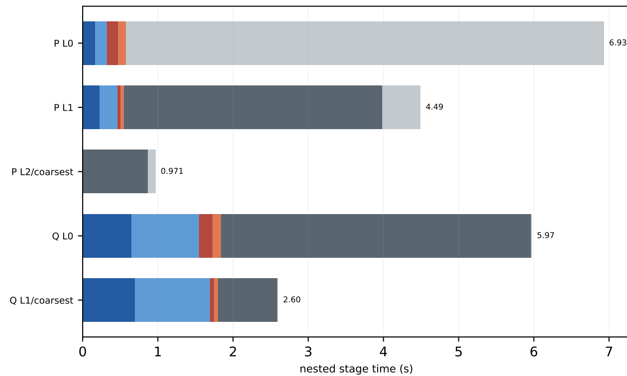
V100 c128 16x16x16x16 MG-3 trace-on mass=0.050, block=2x2x2x2, nvec=12
