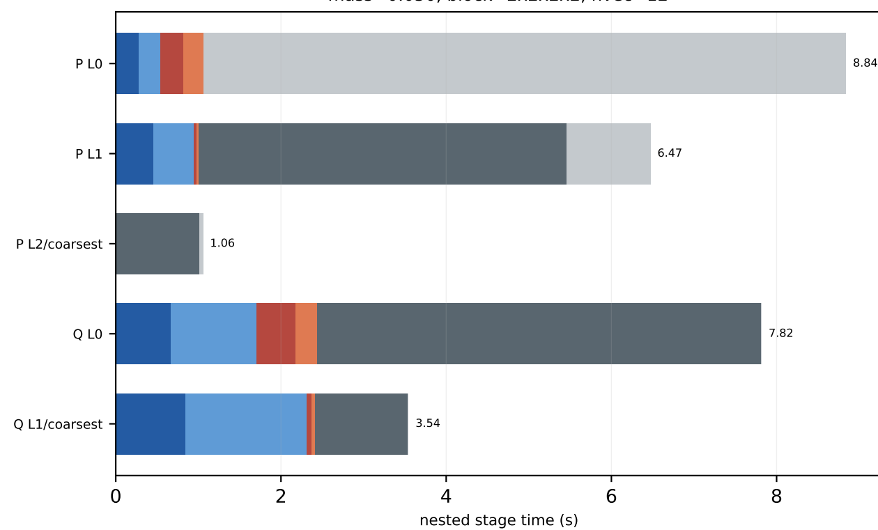
V100 c64 16x32x32x48 MG-3 trace-on mass=0.050, block=2x2x2x2, nvec=12
