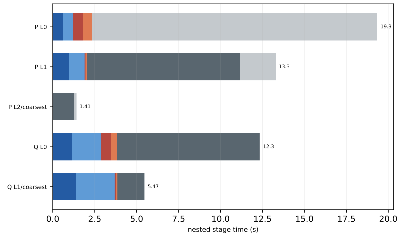
V100 c128 16x16x32x32 MG-3 trace-on mass=0.050, block=2x2x2x2, nvec=12
