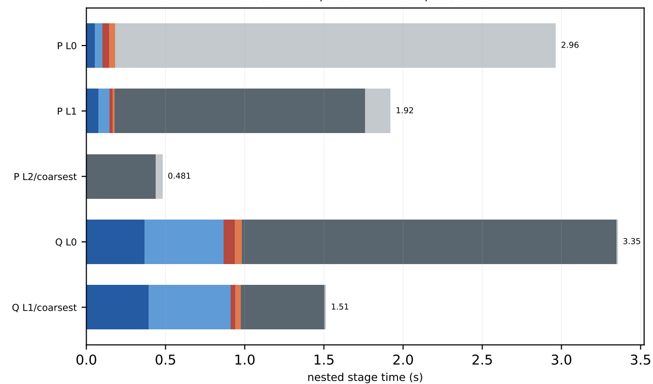
V100 c64 16x16x16x16 MG-3 trace-on mass=0.050, block=2x2x2x2, nvec=12
