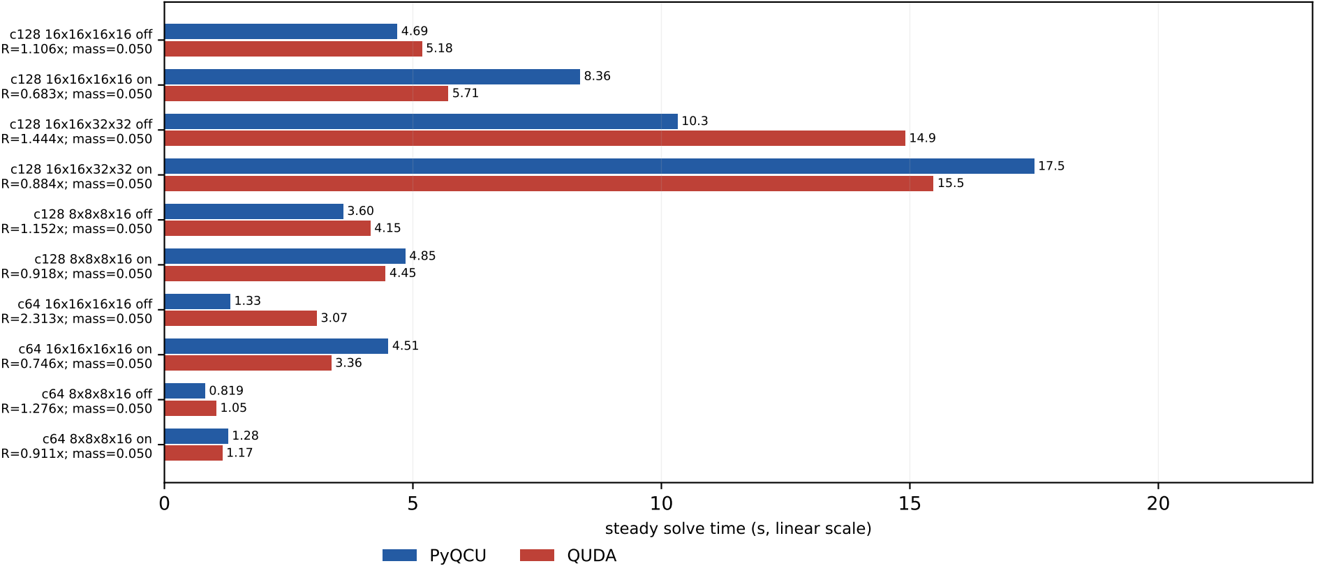
P100 absolute MG-3 steady times mass=0.050, kappa=0.123457, block=2x2x2x2, nvec=12
