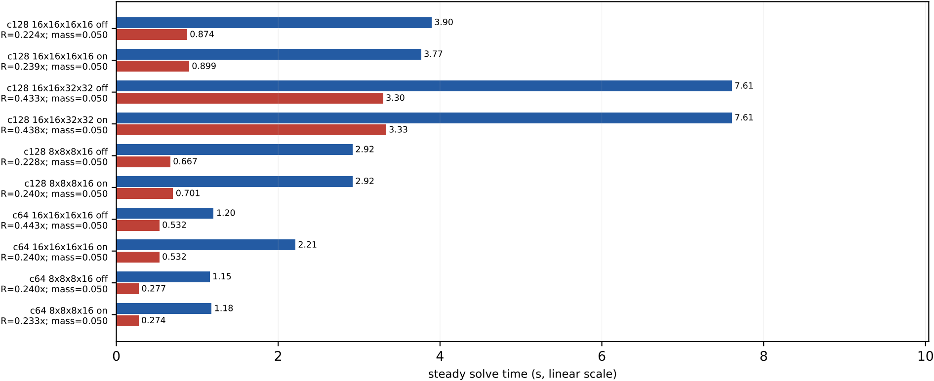
P100 absolute BiCGStab steady times mass=0.050, kappa=0.123457, block=2x2x2x2, nvec=12
