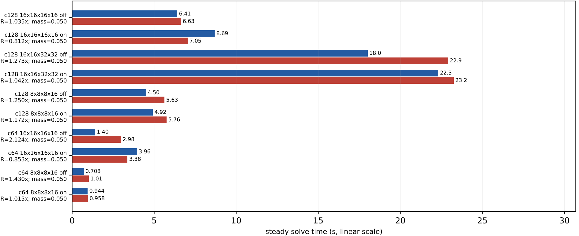
P100 absolute MG-2 steady times mass=0.050, kappa=0.123457, block=2x2x2x2, nvec=12
