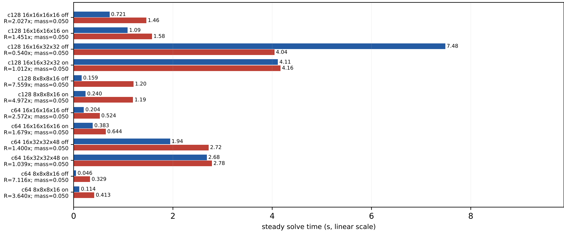
V100 absolute MG-2 steady times mass=0.050, kappa=0.123457, block=2x2x2x2, nvec=12
