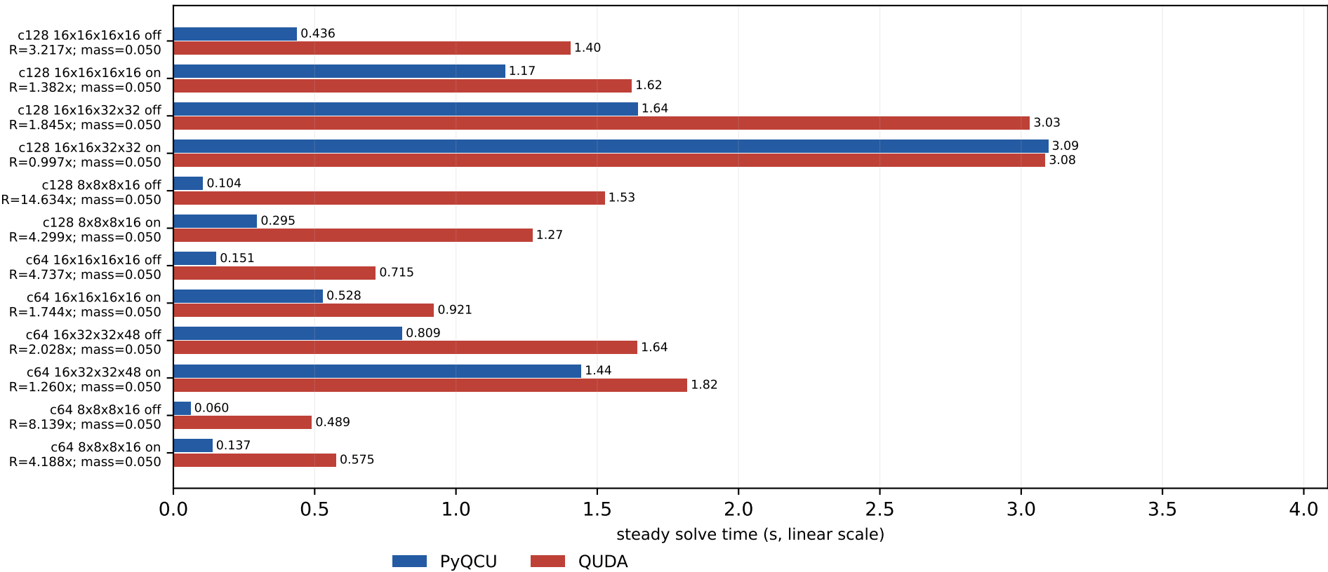
V100 absolute MG-3 steady times mass=0.050, kappa=0.123457, block=2x2x2x2, nvec=12
