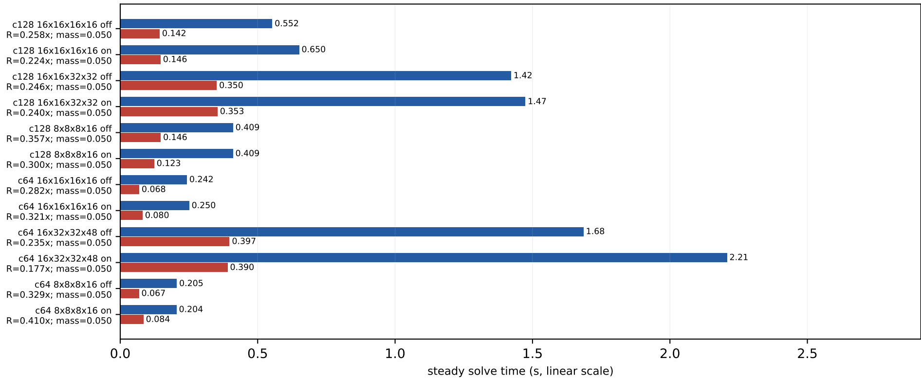
V100 absolute BiCGStab steady times mass=0.050, kappa=0.123457, block=2x2x2x2, nvec=12
