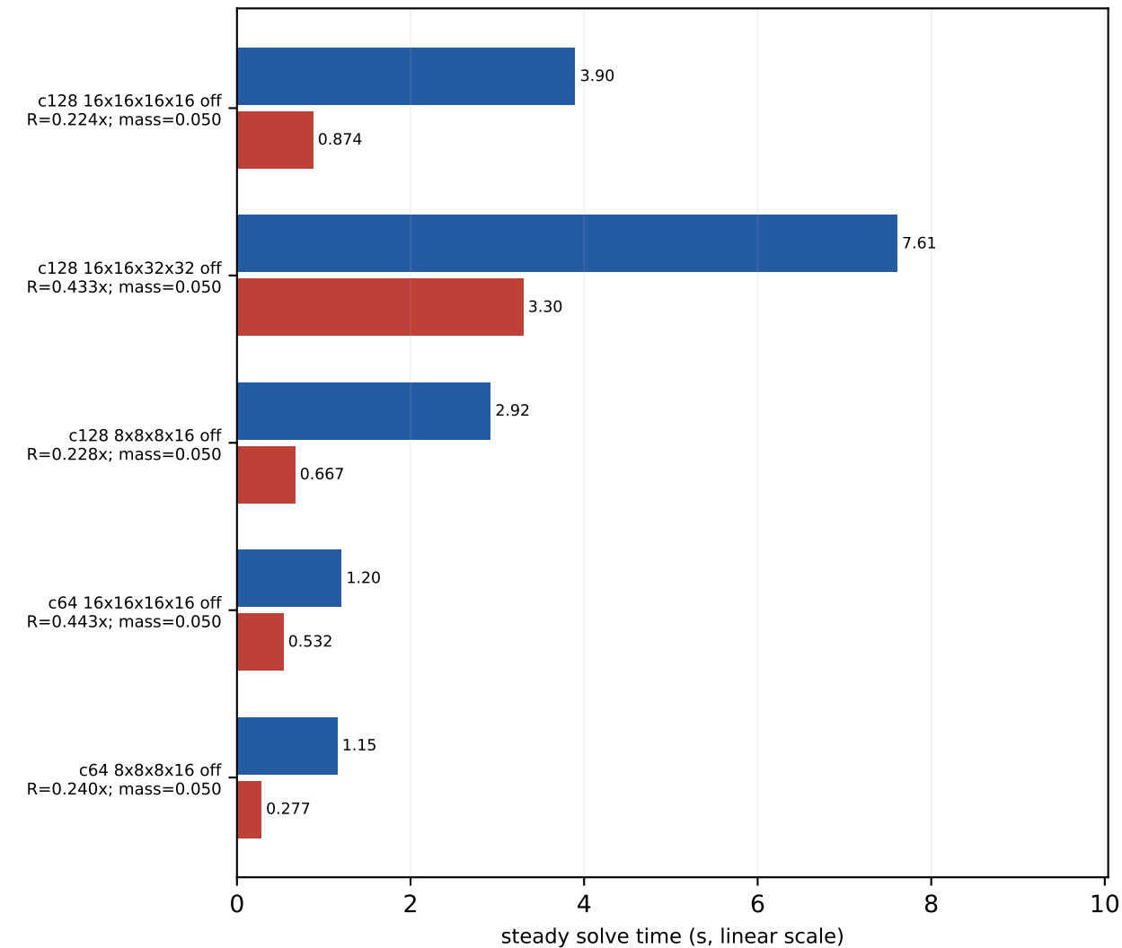
P100 BiCGStab trace-off absolute times mass=0.050, kappa=0.123457, block=2x2x2x2, nvec=12
