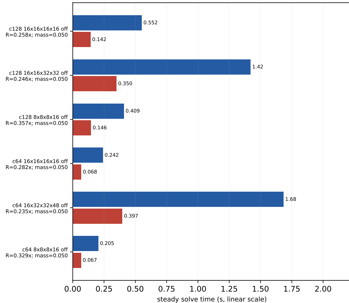
V100 BiCGStab trace-off absolute times mass=0.050, kappa=0.123457, block=2x2x2x2, nvec=12
