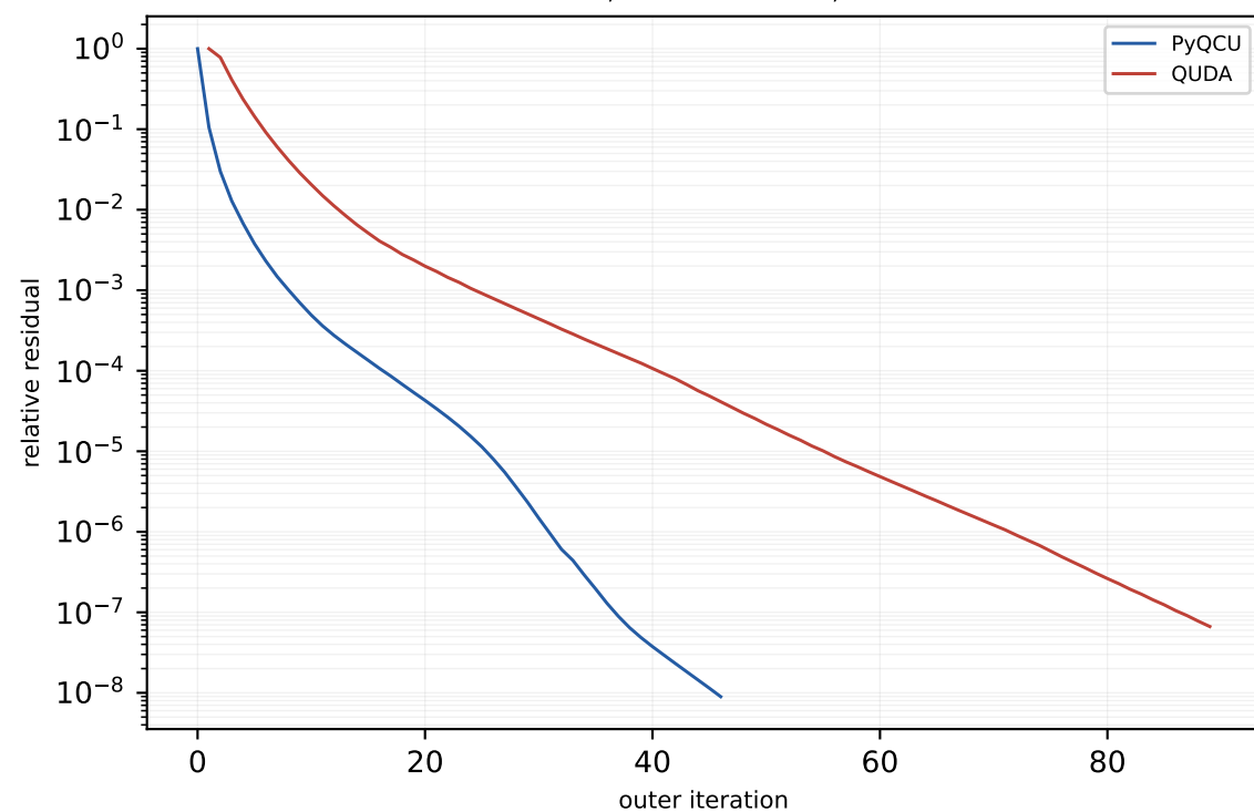
V100 c128 16x16x32x32 MG-3 trace-on mass=0.050, block=2x2x2x2, nvec=12
