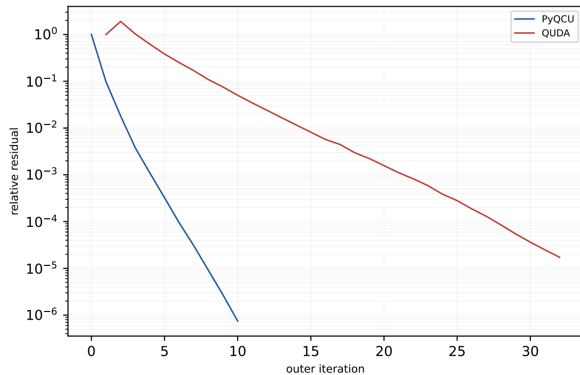
V100 c64 8x8x8x16 MG-3 trace-on mass=0.050, block=2x2x2x2, nvec=12
