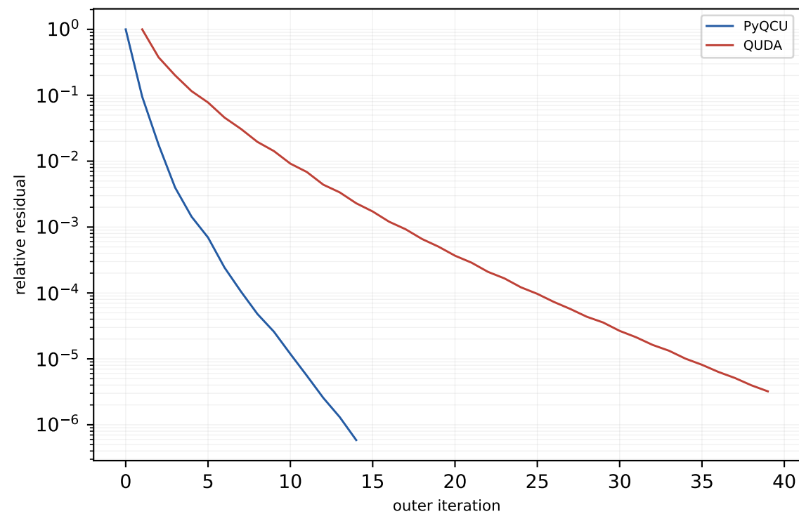
V100 c64 16x32x32x48 MG-3 trace-on mass=0.050, block=2x2x2x2, nvec=12
