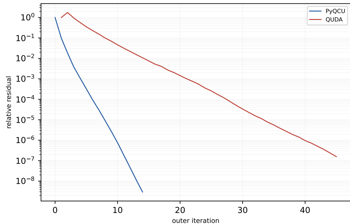
V100 c128 8x8x8x16 MG-3 trace-on mass=0.050, block=2x2x2x2, nvec=12
