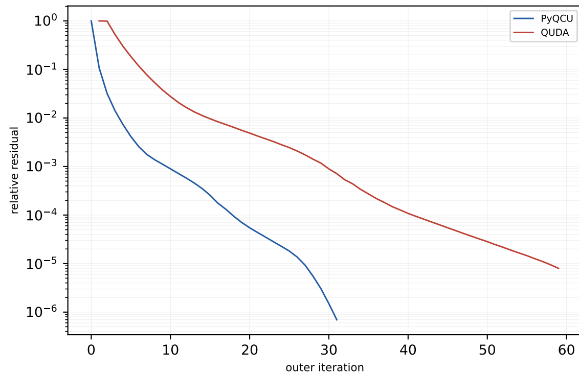
V100 c64 16x16x16x16 MG-3 trace-on mass=0.050, block=2x2x2x2, nvec=12
