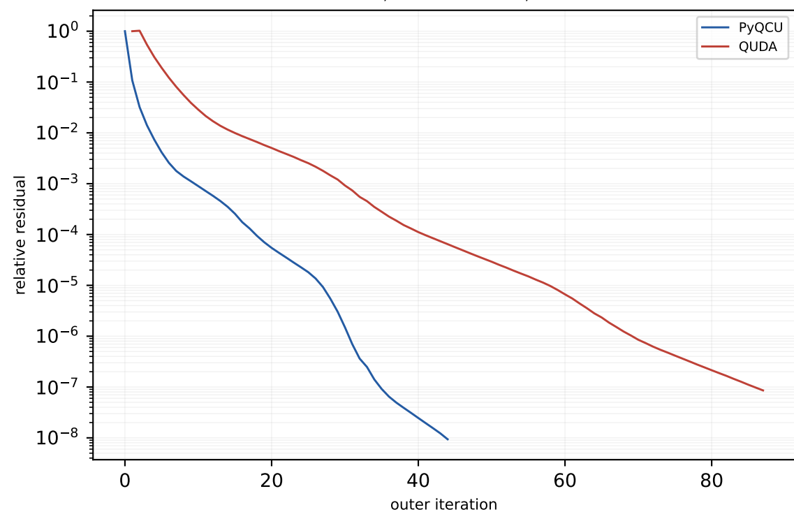
V100 c128 16x16x16x16 MG-3 trace-on mass=0.050, block=2x2x2x2, nvec=12
