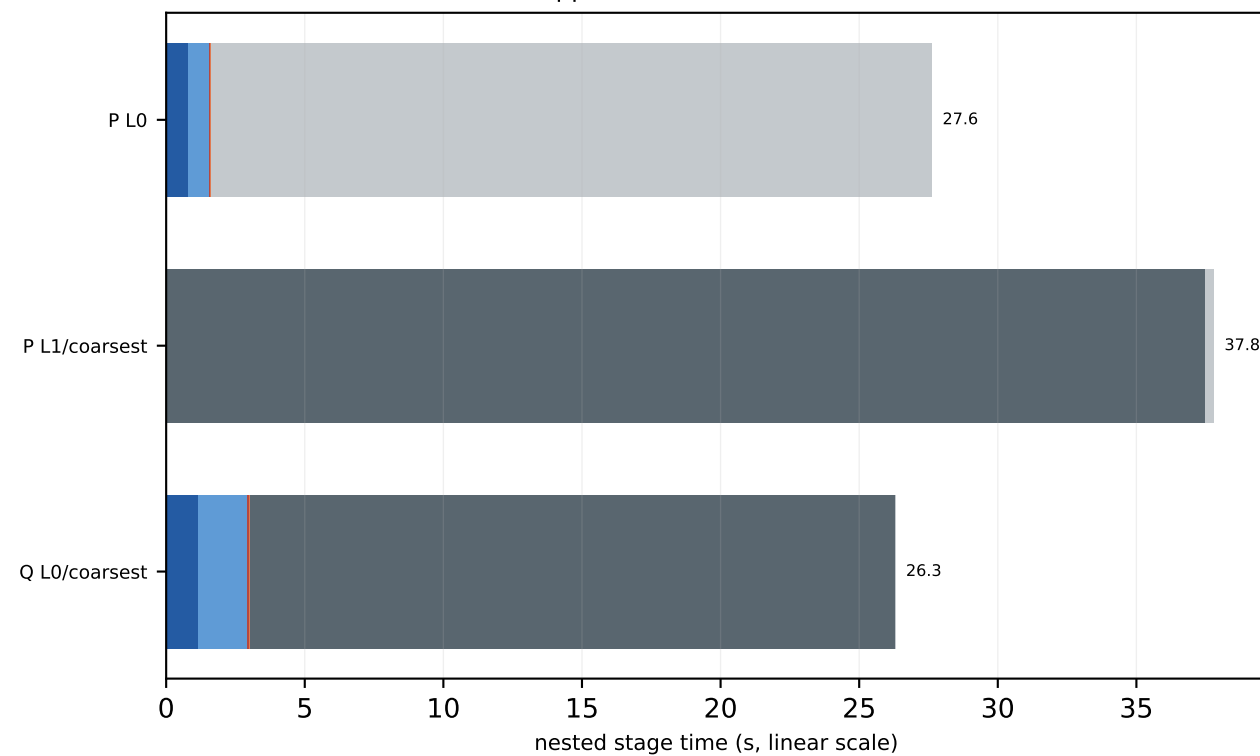
P100 c128 8x8x8x16 MG-2 trace-on mass=0.050, kappa=0.123457, block=2x2x2x2, nvec=12
