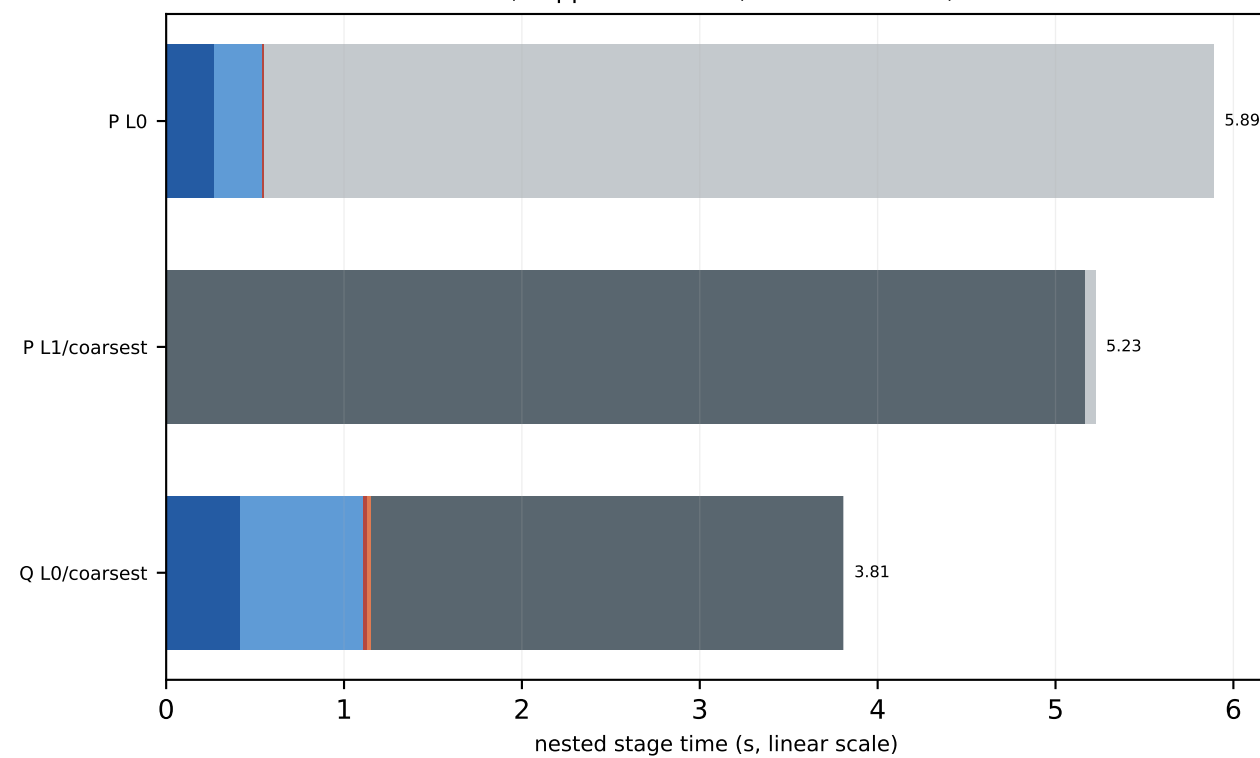
P100 c64 8x8x8x16 MG-2 trace-on mass=0.050, kappa=0.123457, block=2x2x2x2, nvec=12
