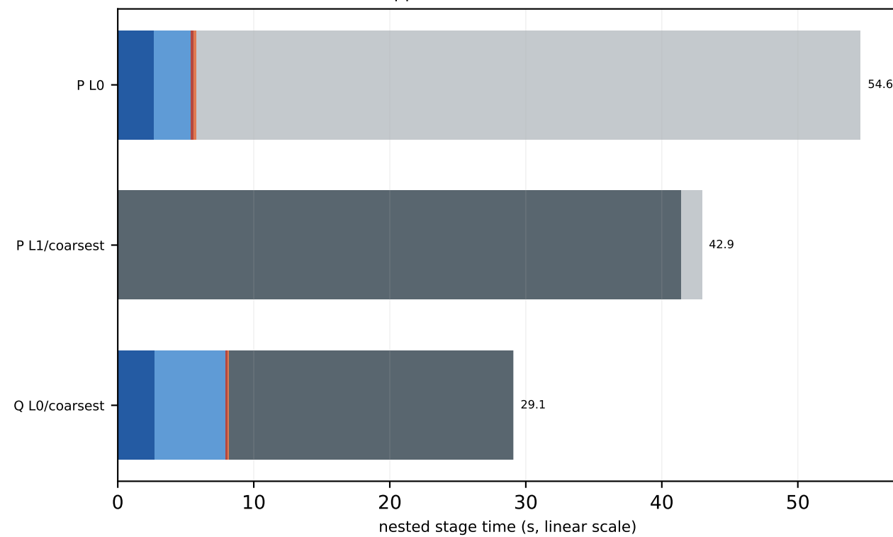
P100 c128 16x16x16x16 MG-2 trace-on mass=0.050, kappa=0.123457, block=2x2x2x2, nvec=12
