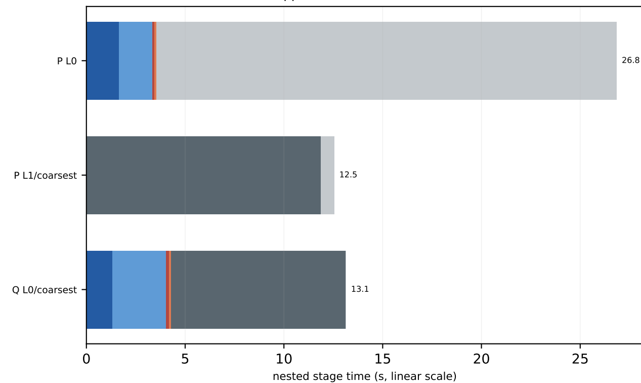
P100 c64 16x16x16x16 MG-2 trace-on mass=0.050, kappa=0.123457, block=2x2x2x2, nvec=12
