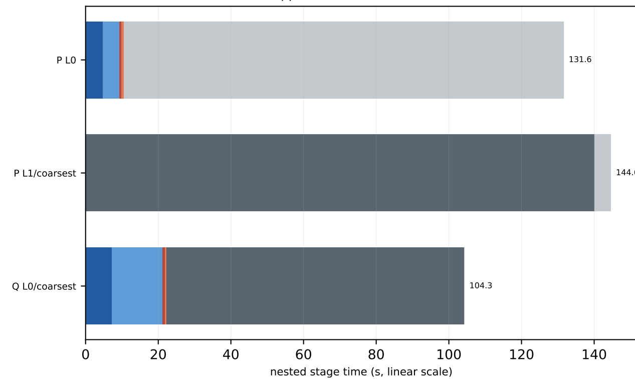
P100 c128 16x16x32x32 MG-2 trace-on mass=0.050, kappa=0.123457, block=2x2x2x2, nvec=12
