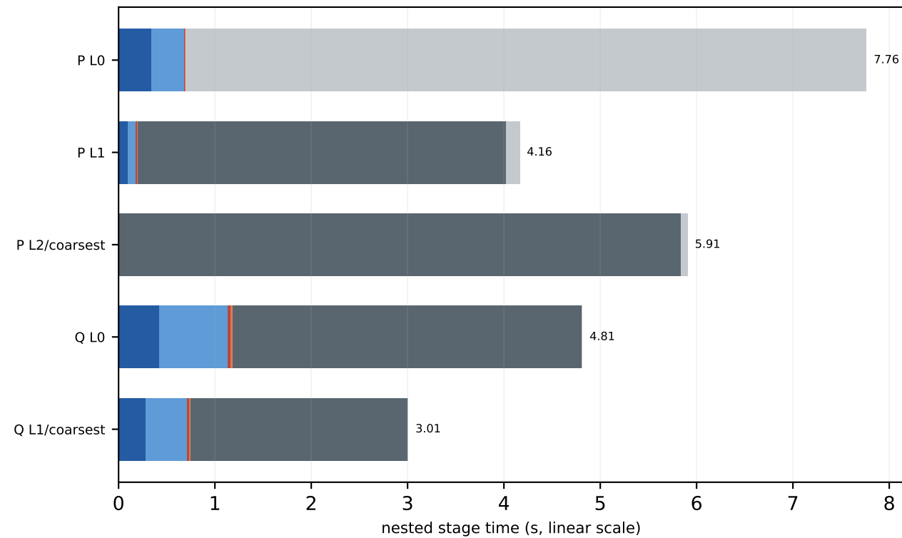
P100 c64 8x8x8x16 MG-3 trace-on mass=0.050, kappa=0.123457, block=2x2x2x2, nvec=12
