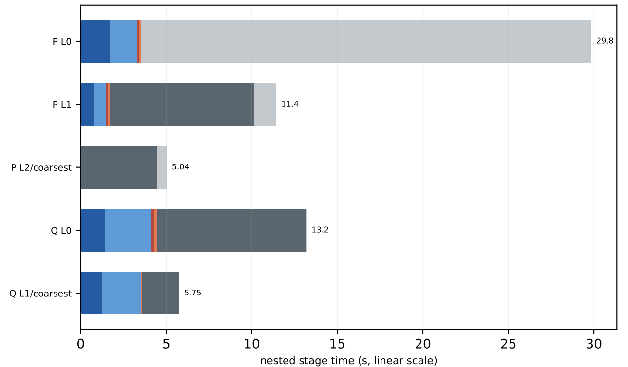
P100 c64 16x16x16x16 MG-3 trace-on mass=0.050, kappa=0.123457, block=2x2x2x2, nvec=12
