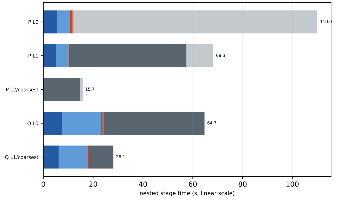
P100 c128 16x16x32x32 MG-3 trace-on mass=0.050, kappa=0.123457, block=2x2x2x2, nvec=12
