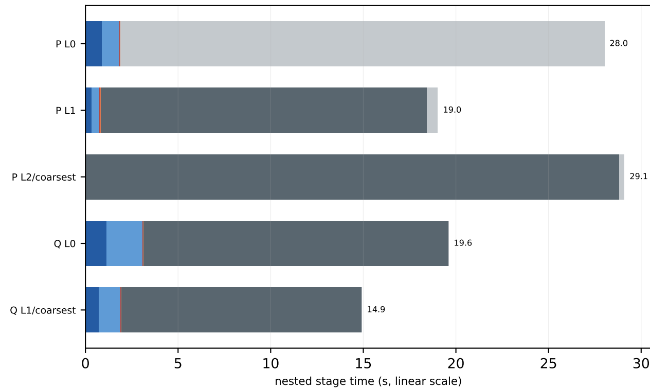
P100 c128 8x8x8x16 MG-3 trace-on mass=0.050, kappa=0.123457, block=2x2x2x2, nvec=12
