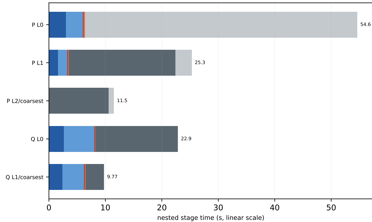
P100 c128 16x16x16x16 MG-3 trace-on mass=0.050, kappa=0.123457, block=2x2x2x2, nvec=12
