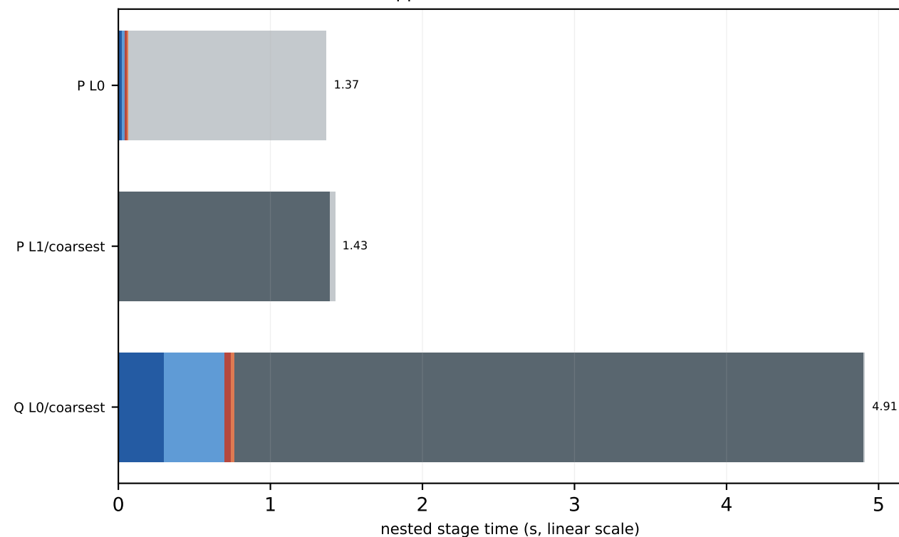
V100 c128 8x8x8x16 MG-2 trace-on mass=0.050, kappa=0.123457, block=2x2x2x2, nvec=12
