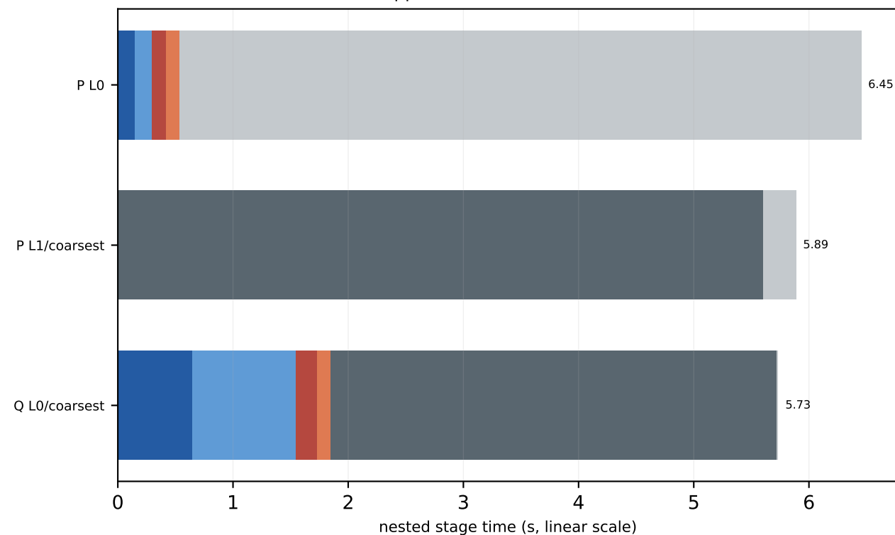
V100 c128 16x16x16x16 MG-2 trace-on mass=0.050, kappa=0.123457, block=2x2x2x2, nvec=12
