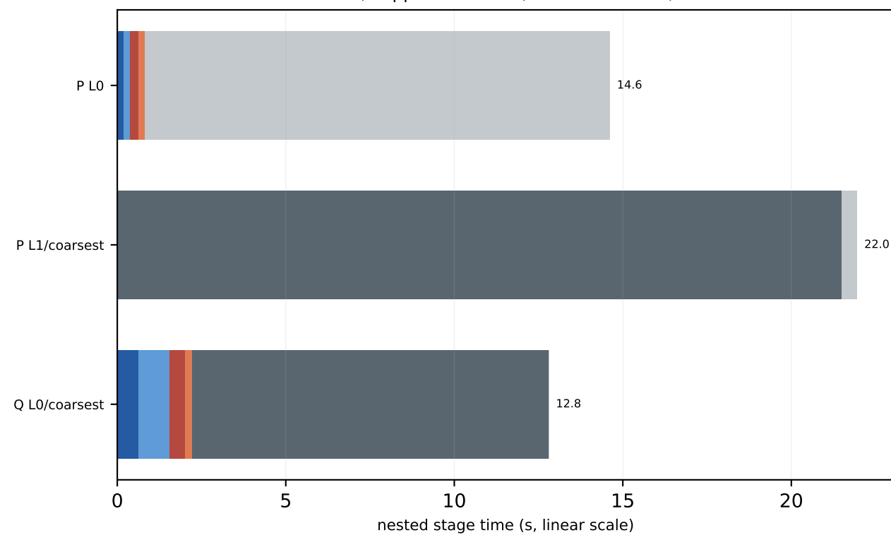
V100 c64 16x32x32x48 MG-2 trace-on mass=0.050, kappa=0.123457, block=2x2x2x2, nvec=12
