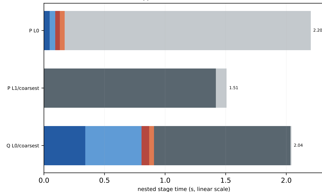
V100 c64 16x16x16x16 MG-2 trace-on mass=0.050, kappa=0.123457, block=2x2x2x2, nvec=12
