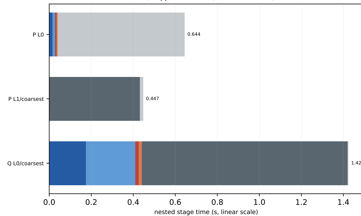
V100 c64 8x8x8x16 MG-2 trace-on mass=0.050, kappa=0.123457, block=2x2x2x2, nvec=12
