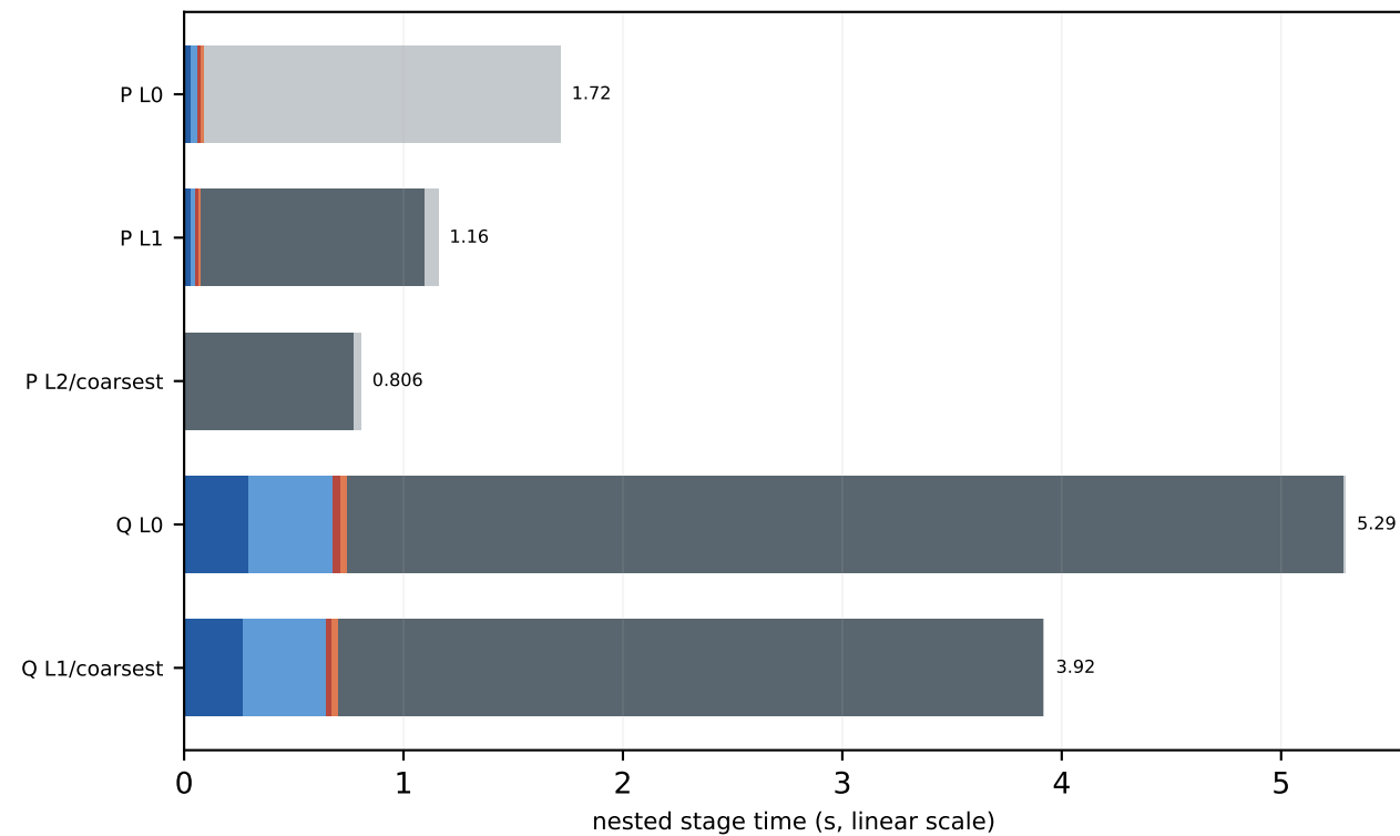
V100 c128 8x8x8x16 MG-3 trace-on mass=0.050, kappa=0.123457, block=2x2x2x2, nvec=12
