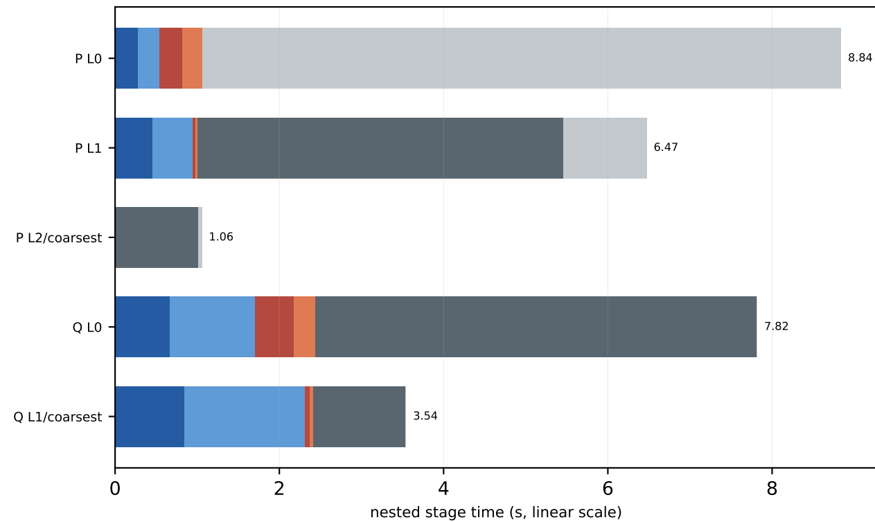
V100 c64 16x32x32x48 MG-3 trace-on mass=0.050, kappa=0.123457, block=2x2x2x2, nvec=12
