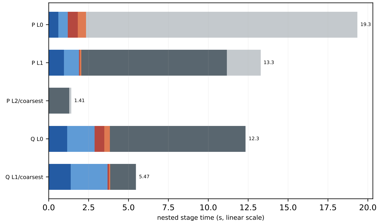
V100 c128 16x16x32x32 MG-3 trace-on mass=0.050, kappa=0.123457, block=2x2x2x2, nvec=12
