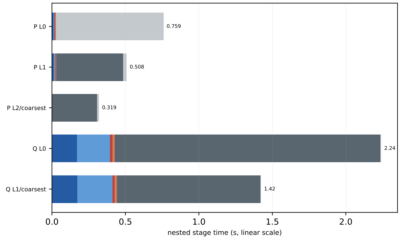
V100 c64 8x8x8x16 MG-3 trace-on mass=0.050, kappa=0.123457, block=2x2x2x2, nvec=12
