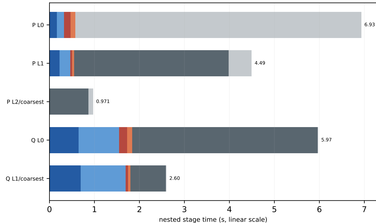
V100 c128 16x16x16x16 MG-3 trace-on mass=0.050, kappa=0.123457, block=2x2x2x2, nvec=12
