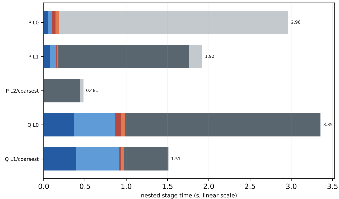
V100 c64 16x16x16x16 MG-3 trace-on mass=0.050, kappa=0.123457, block=2x2x2x2, nvec=12
