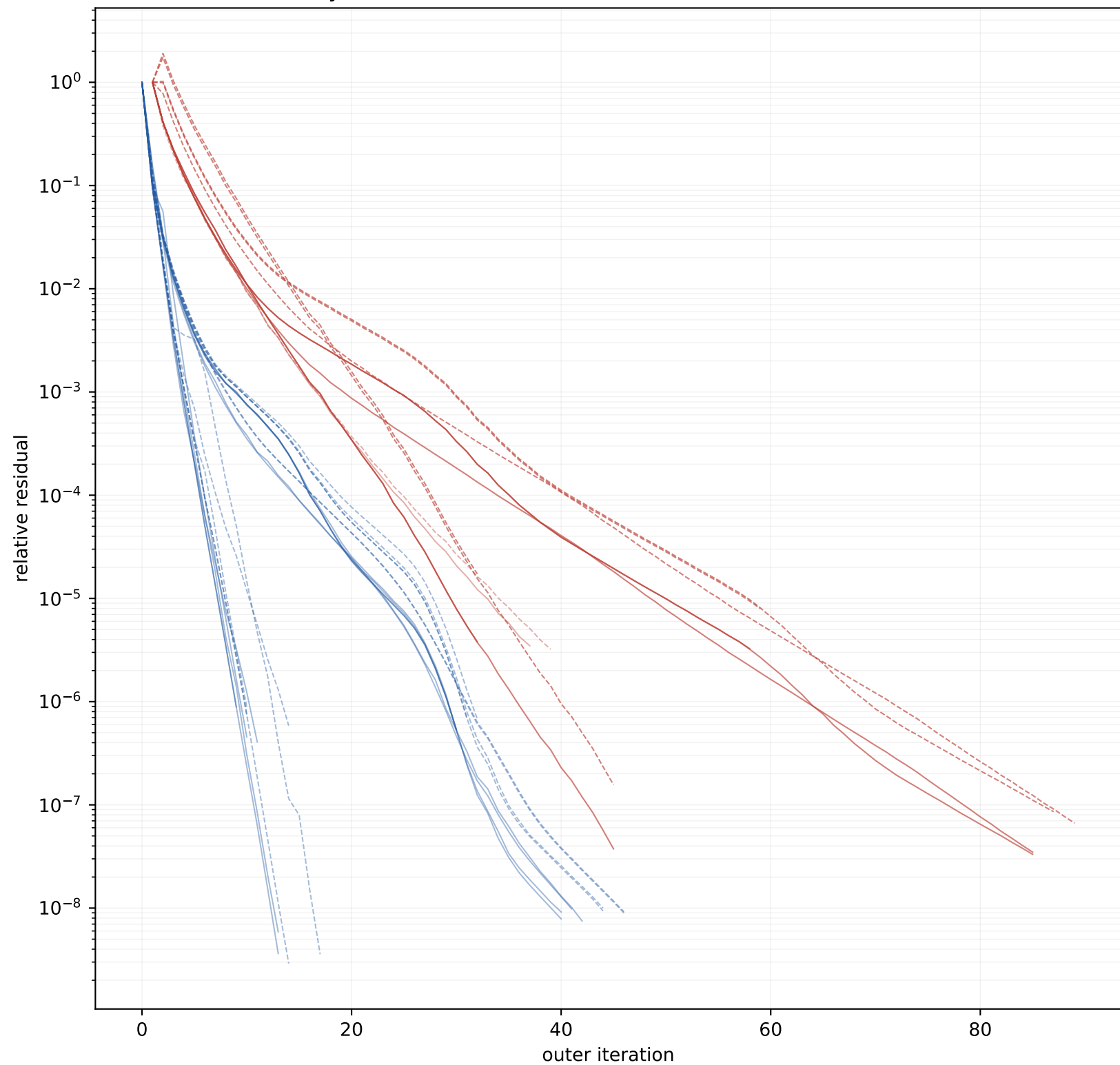
Steady-state finest-level residual curves (44 side/case curves)
