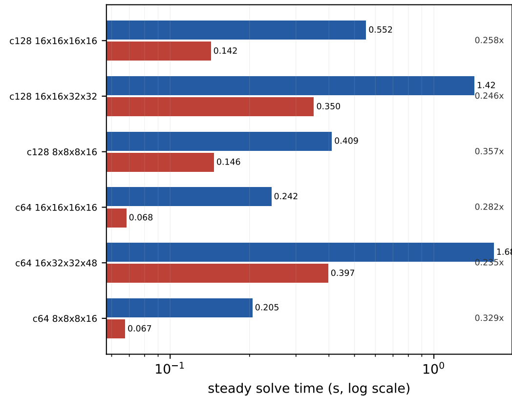
V100 BiCGStab trace-off (n=6)
