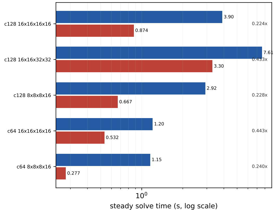
P100 BiCGStab trace-off (n=5)
