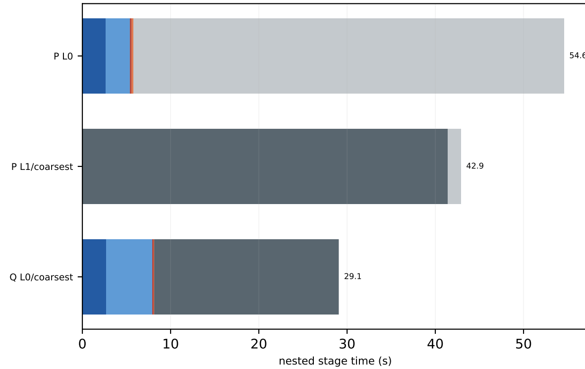
P100 c128 16x16x16x16 MG-2 trace-on
