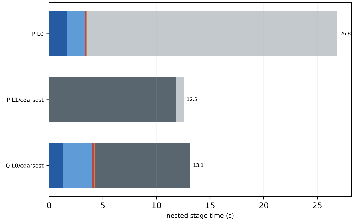
P100 c64 16x16x16x16 MG-2 trace-on
