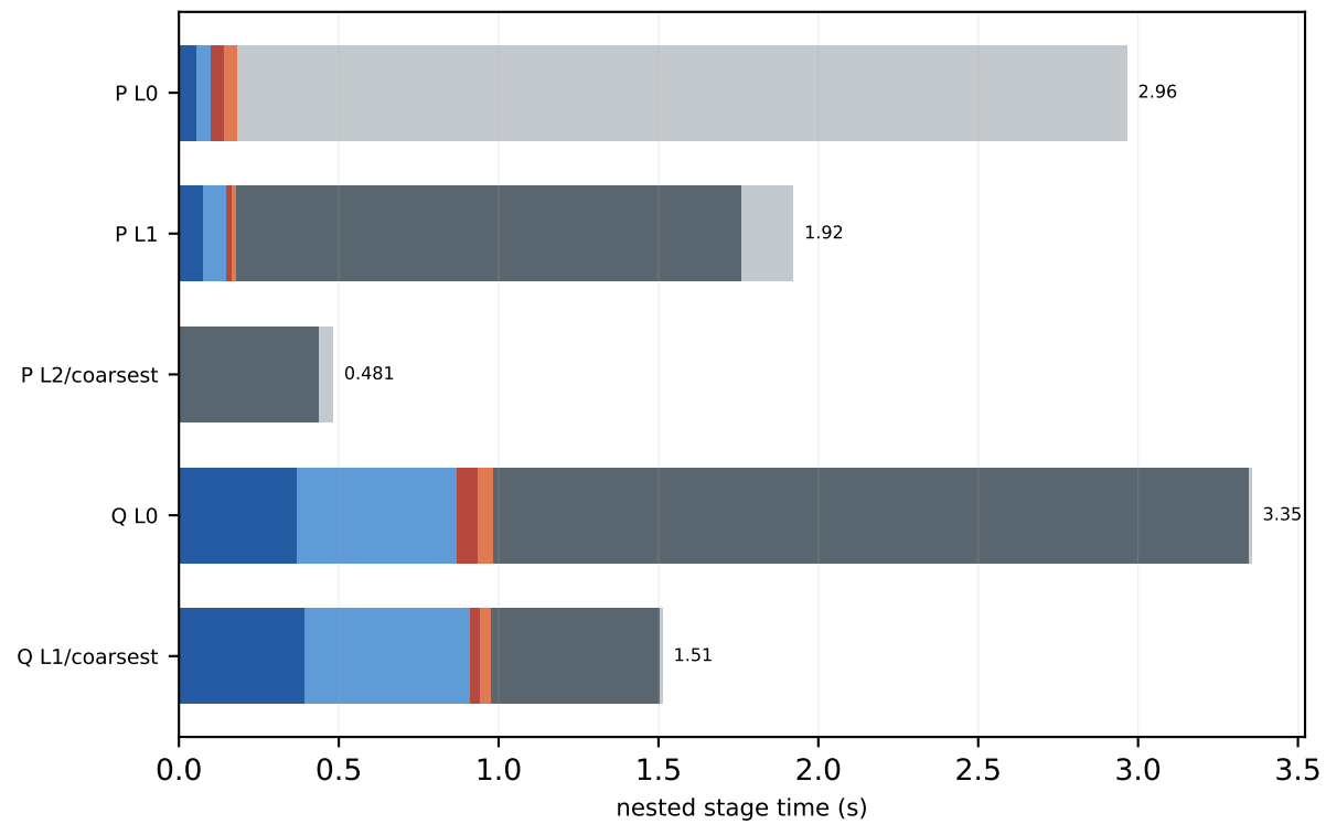
V100 c64 16x16x16x16 MG-3 trace-on
