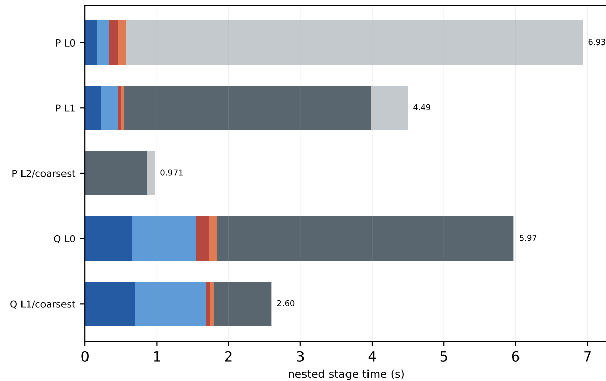
V100 c128 16x16x16x16 MG-3 trace-on
