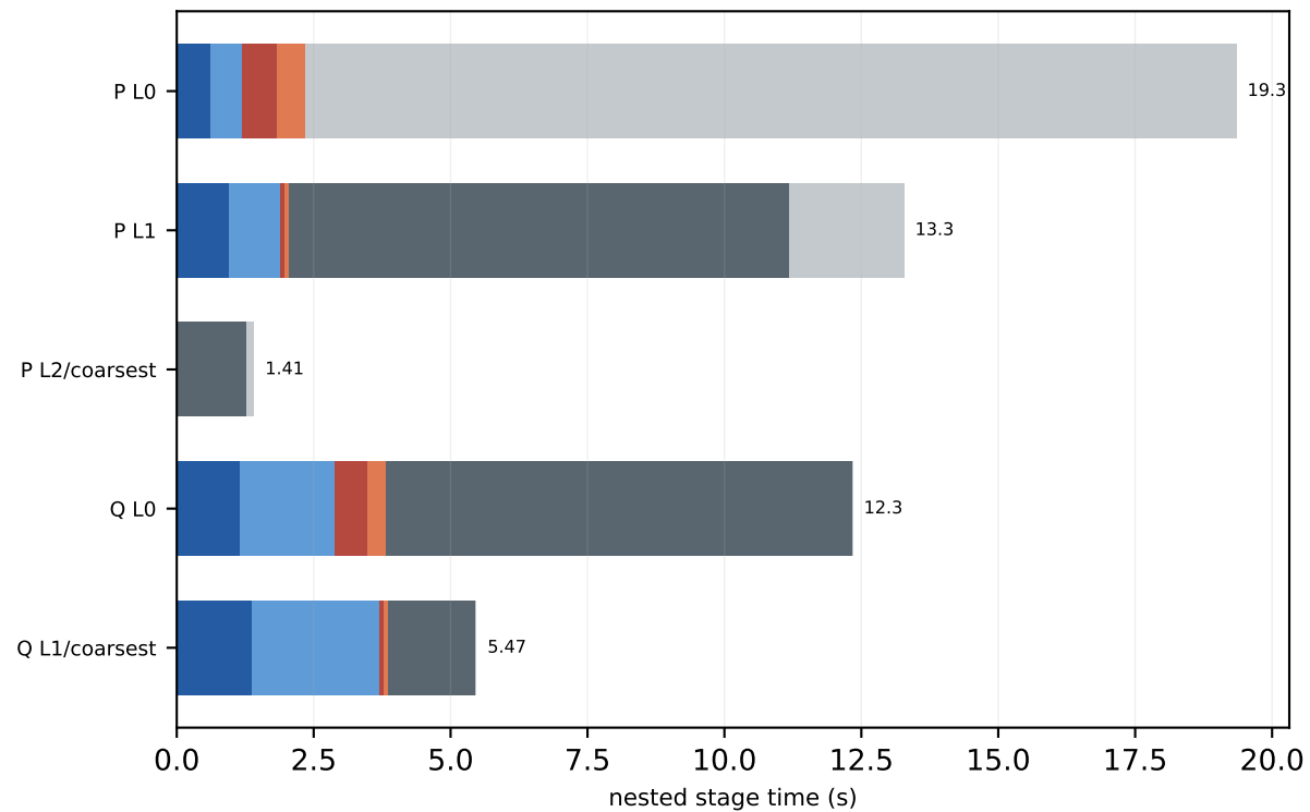
V100 c128 16x16x32x32 MG-3 trace-on
