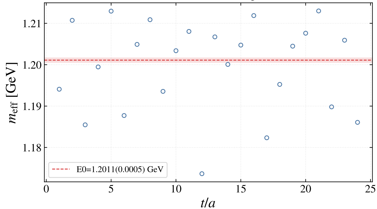
Effective Mass (lamet-agent)
