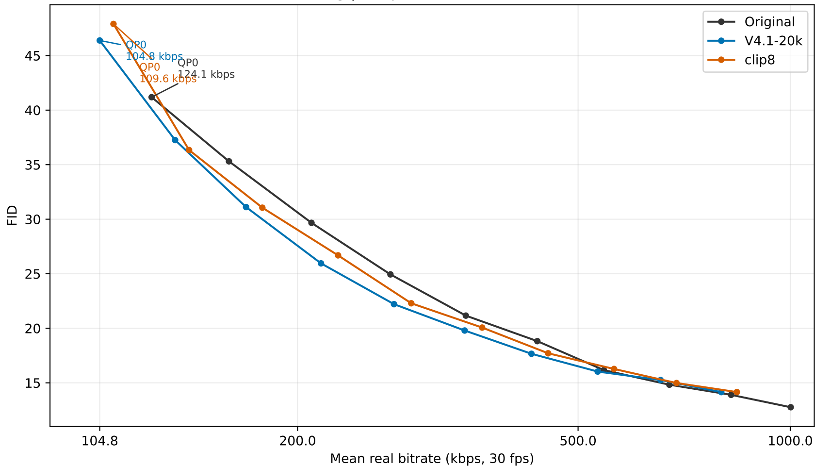
Fresh U-Long | 30 fps, 64 frames, canonical RGB
