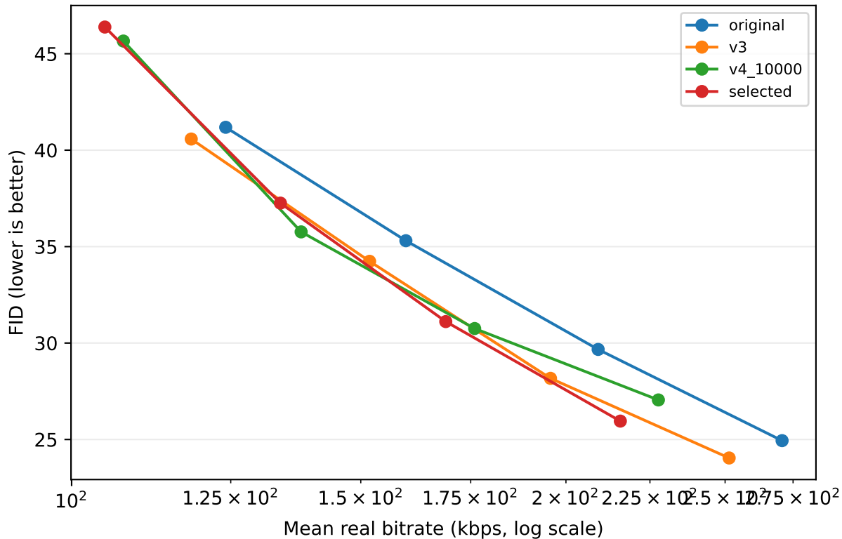
Final — FID
