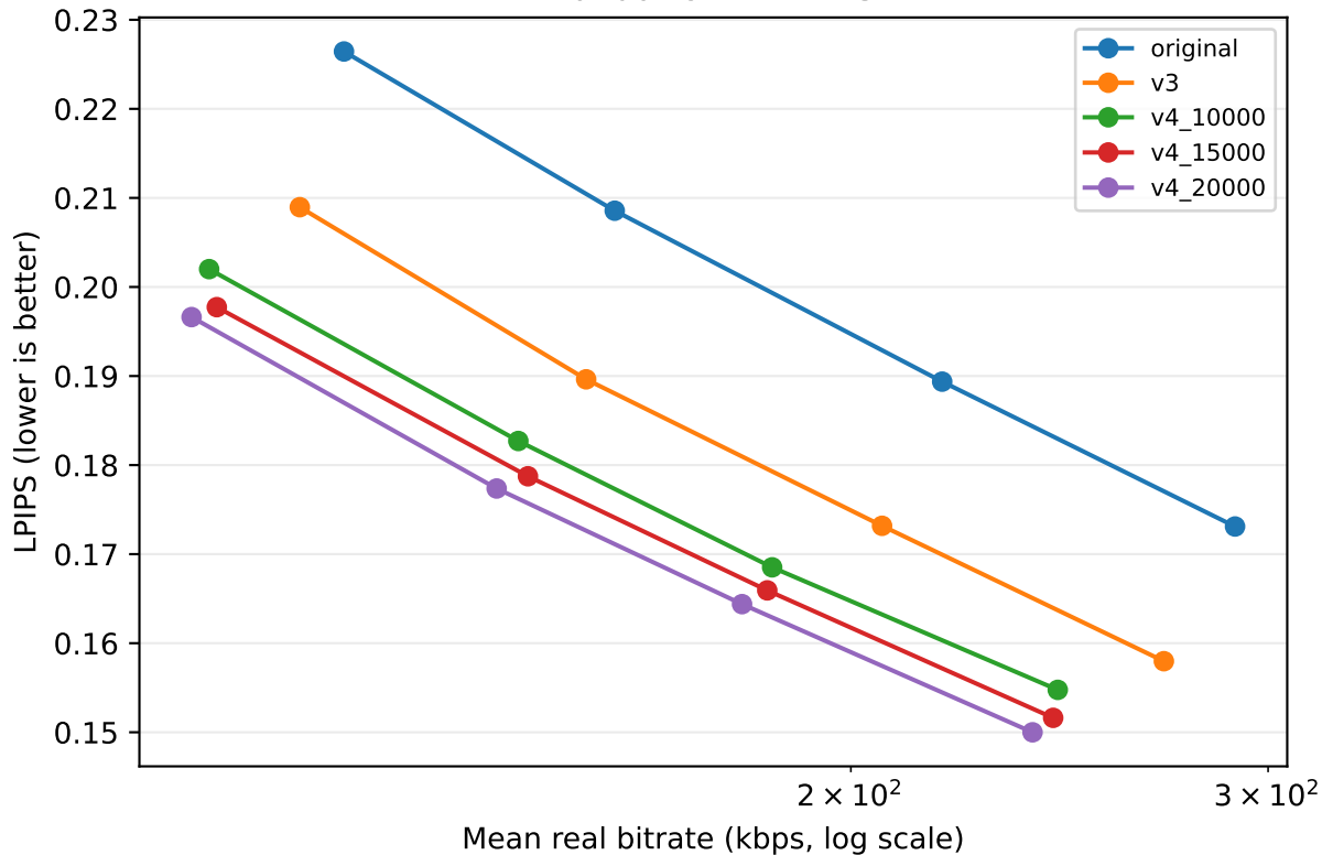
Validation — LPIPS
