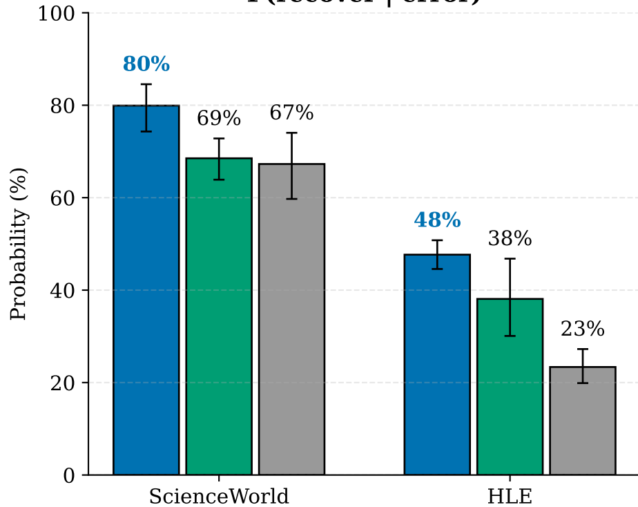
P(recover | error)
