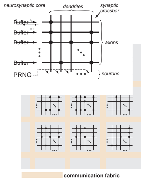
Figure 3: TrueNorth architecture. Neurosynaptic cores connect inputs to neurons using a synaptic crossbar. An asynchronous communication fabric routes events between cores.
