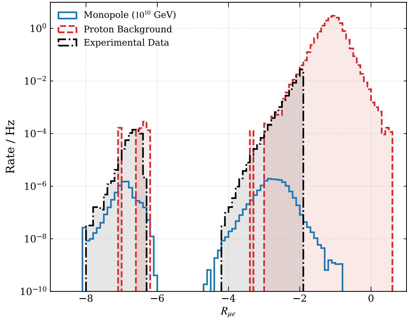
(b) Muon-to-Electron Ratio
