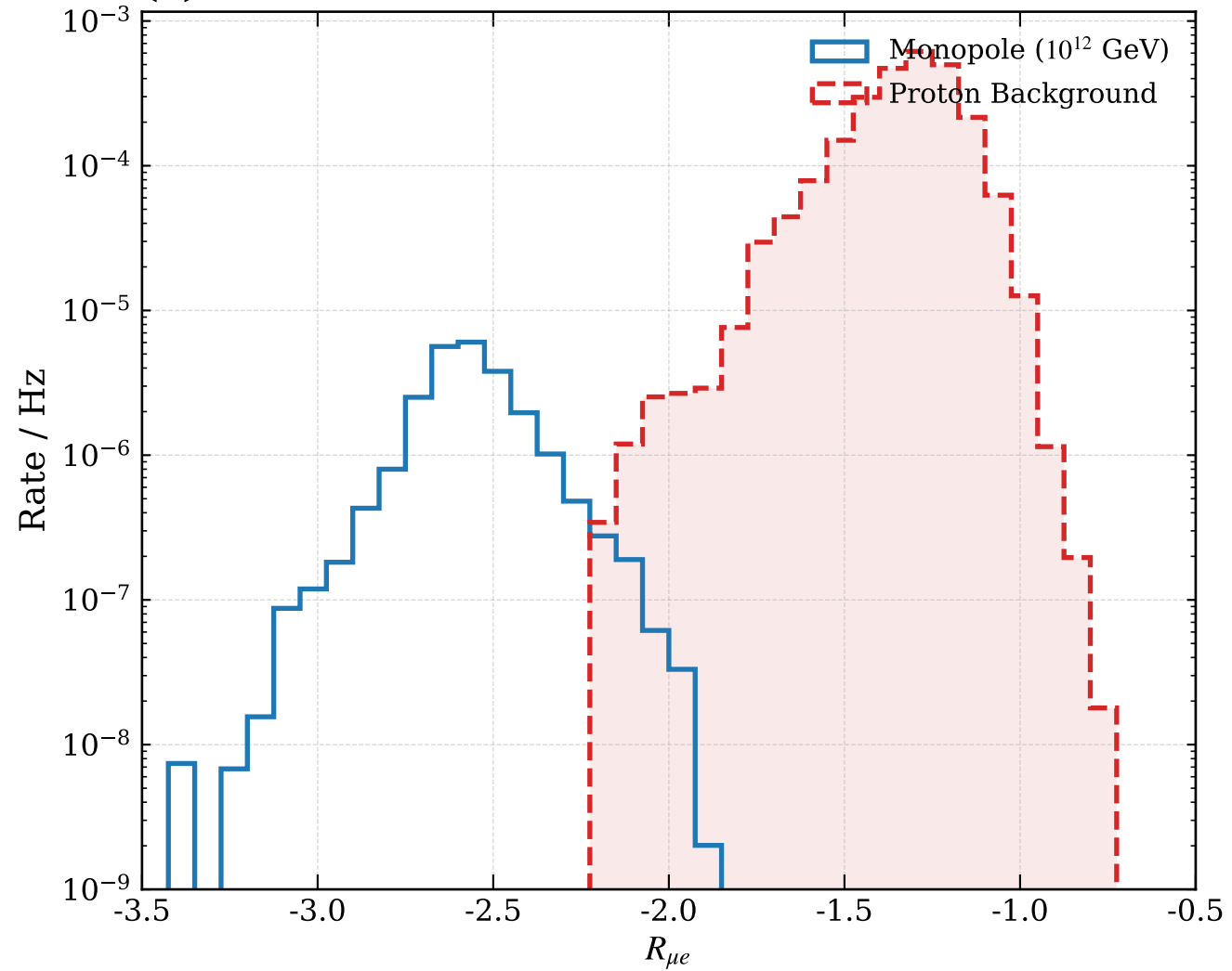
(b) Muon-to-EM Ratio
