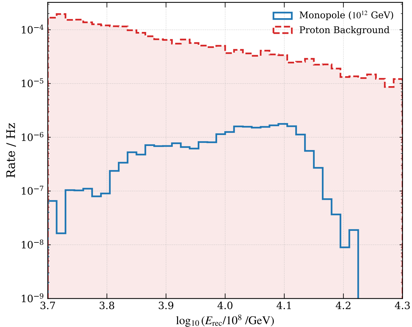
(a) Reconstructed Energy
