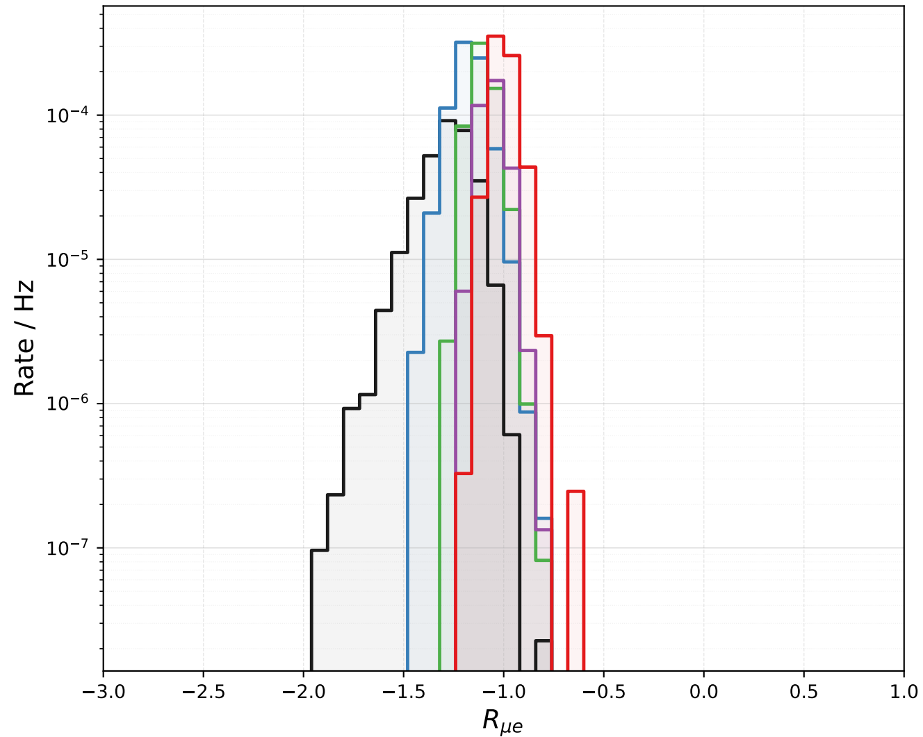
(a) Muon-to-EM Ratio
