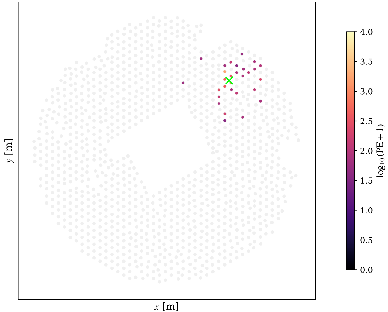
(b) MD Array Response
