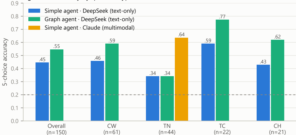
Agent QA accuracy by question type — NExT-QA val
