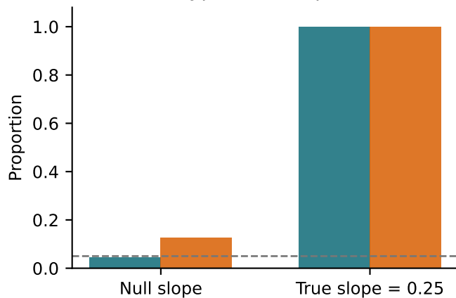
C. Bias under LD correlation
