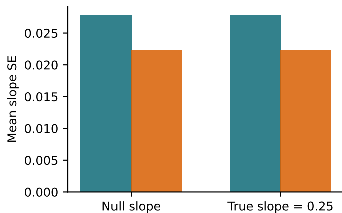
D. Standard-error distortion
