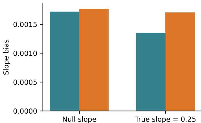
C. Bias under LD correlation
