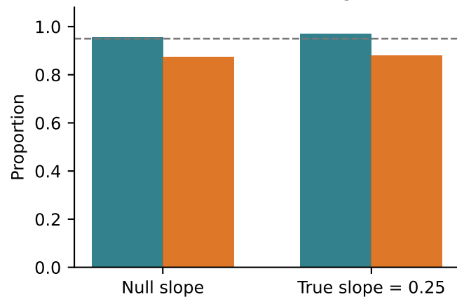
D. Standard-error distortion
