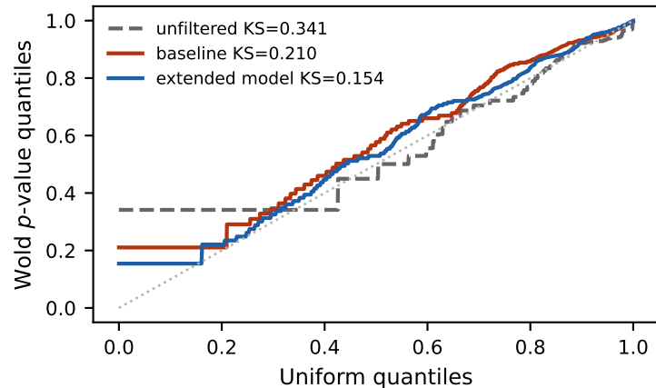
Wold KS before/after filtering
