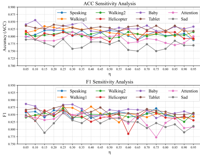
Fig. s-1. Sensitivity analysis of the hyperparameter \eta in terms of ACC and F1-score.
