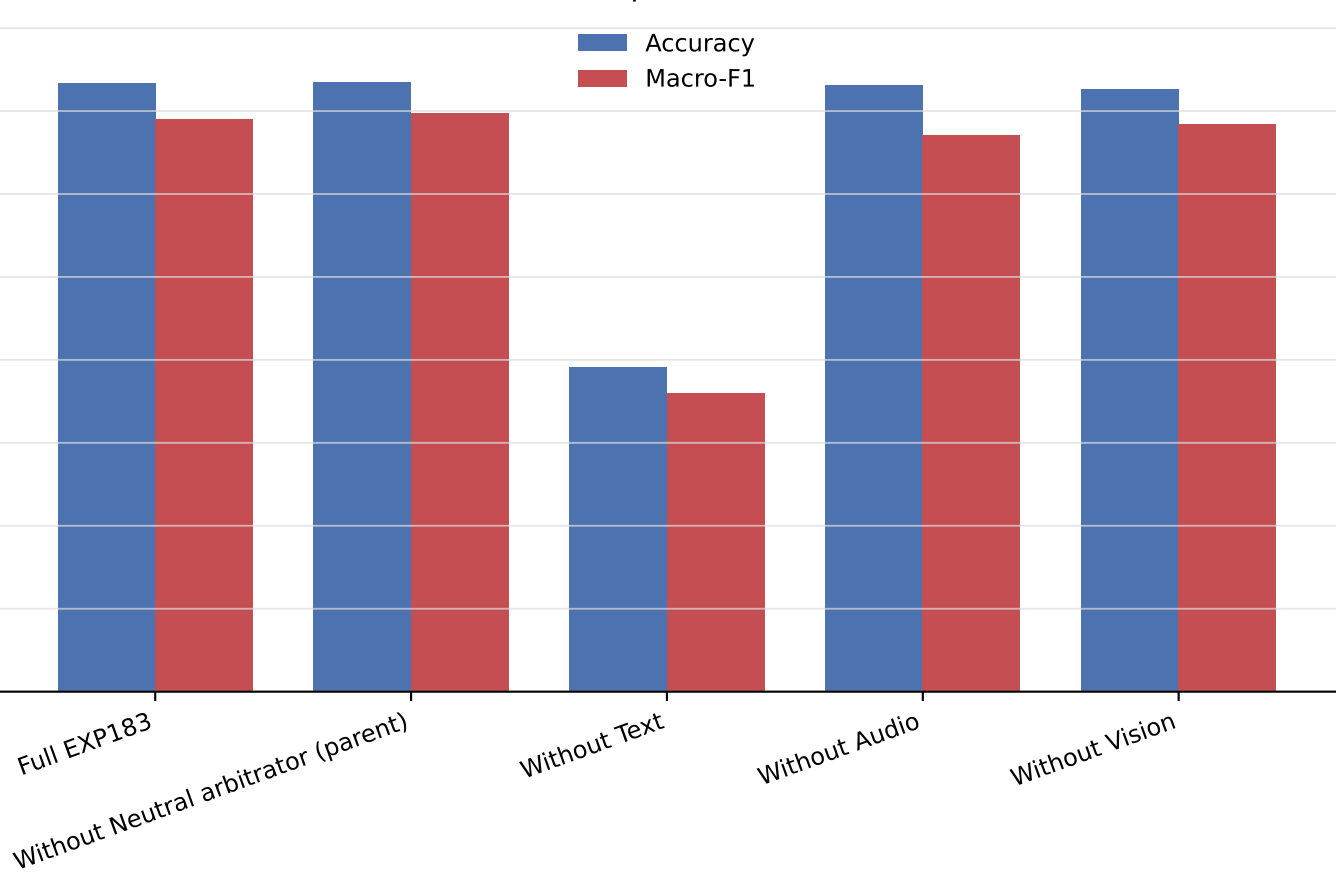
Frozen test component interventions
