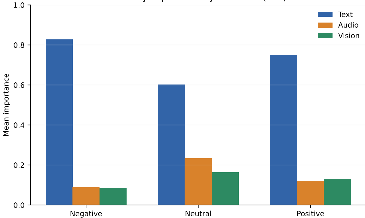
Modality importance by true class (test)
