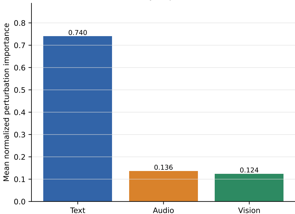
Global modality importance on test
