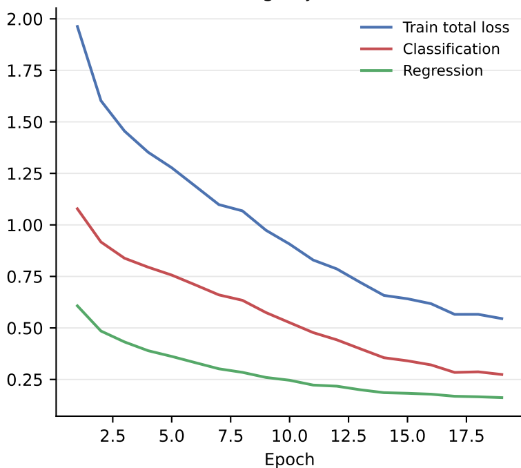
Training objectives
