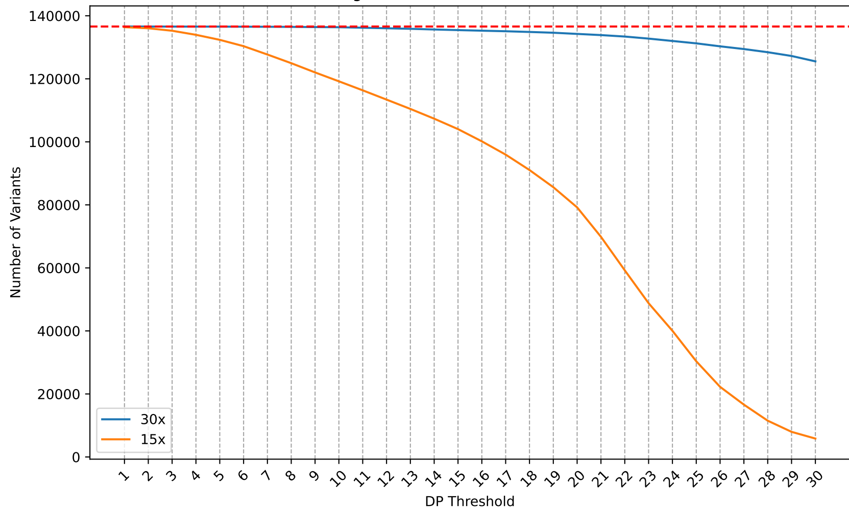
Remaining Variants Across DP Thresholds (PAR)
