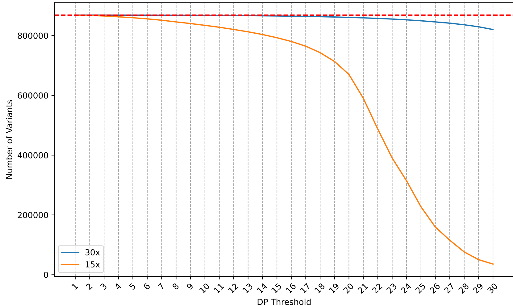
Remaining Variants Across DP Thresholds (chr21)
